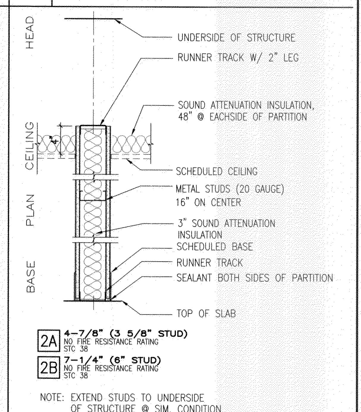
2 NEW PARTIAL HEIGHT PARTITION
