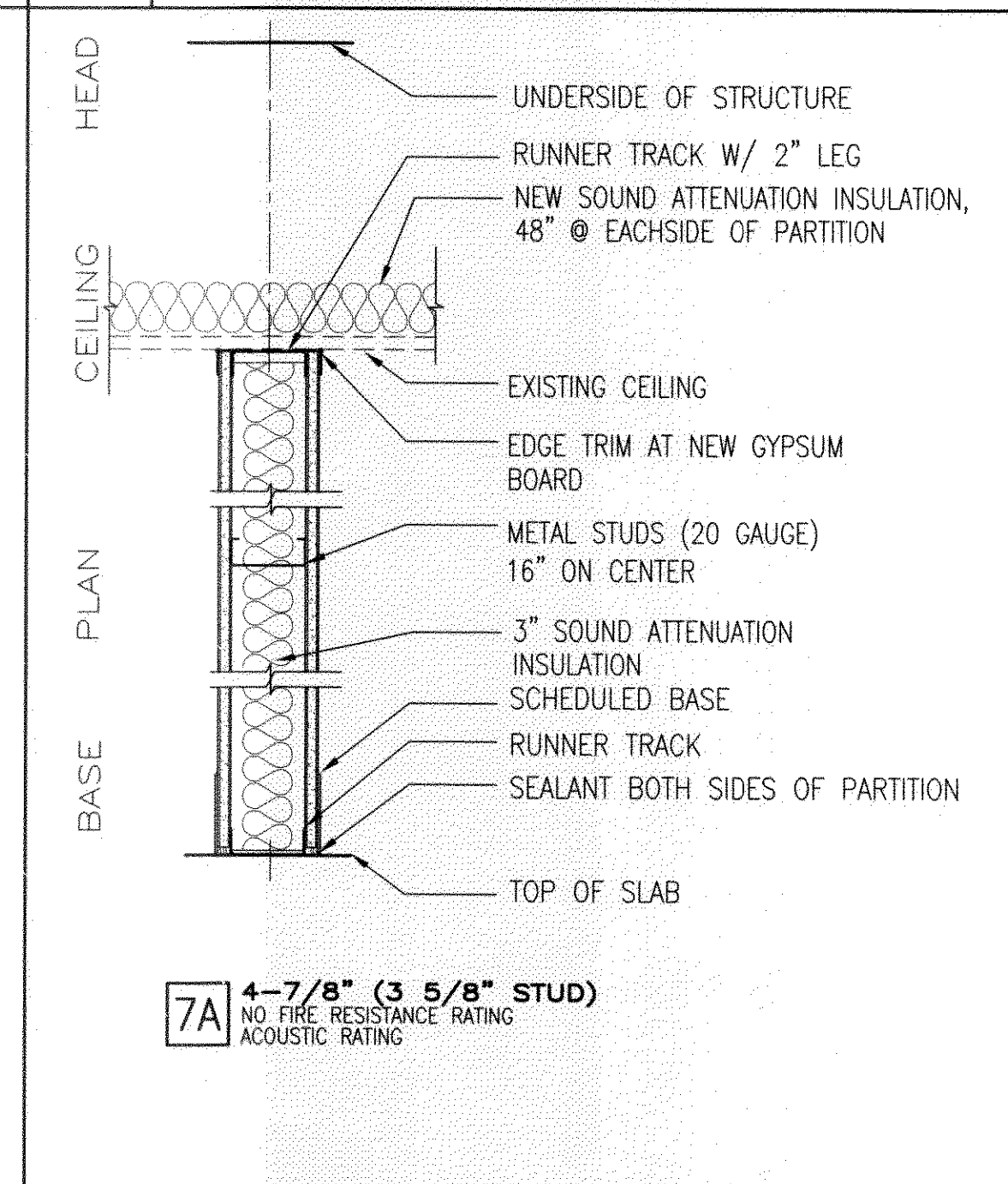
7 PARTIAL HEIGHT PARTITION WALL
