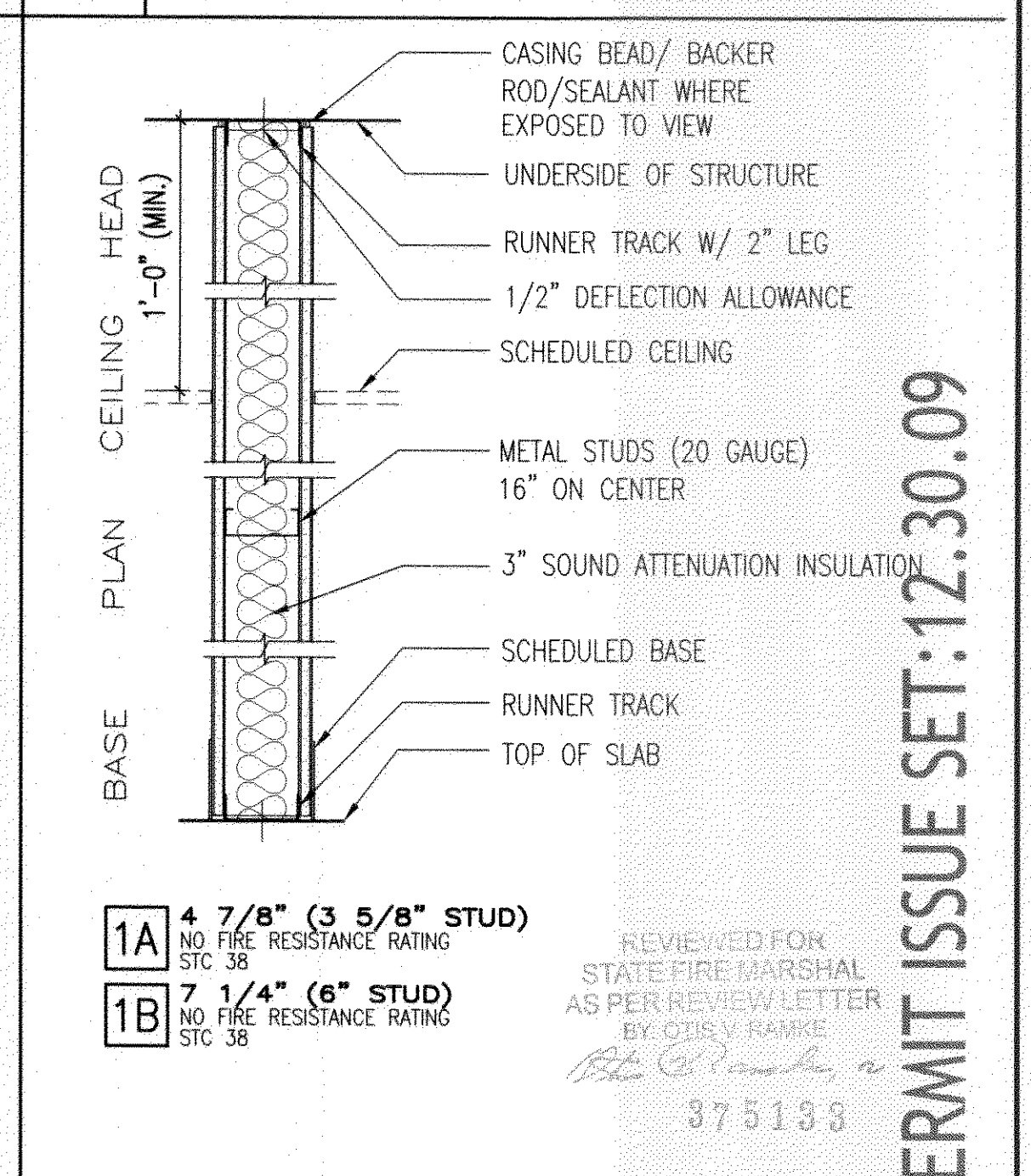
1 FULL HEIGHT PARTITION
