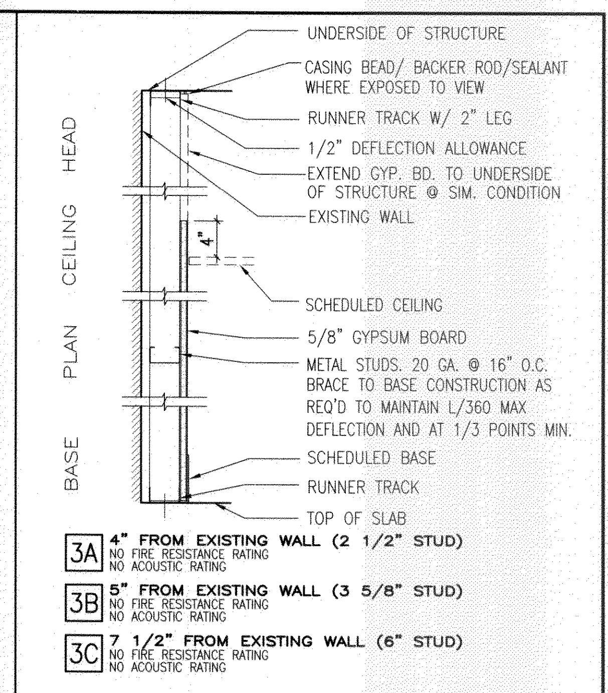
3 NEW PARTITION AT EXISTING WALL
