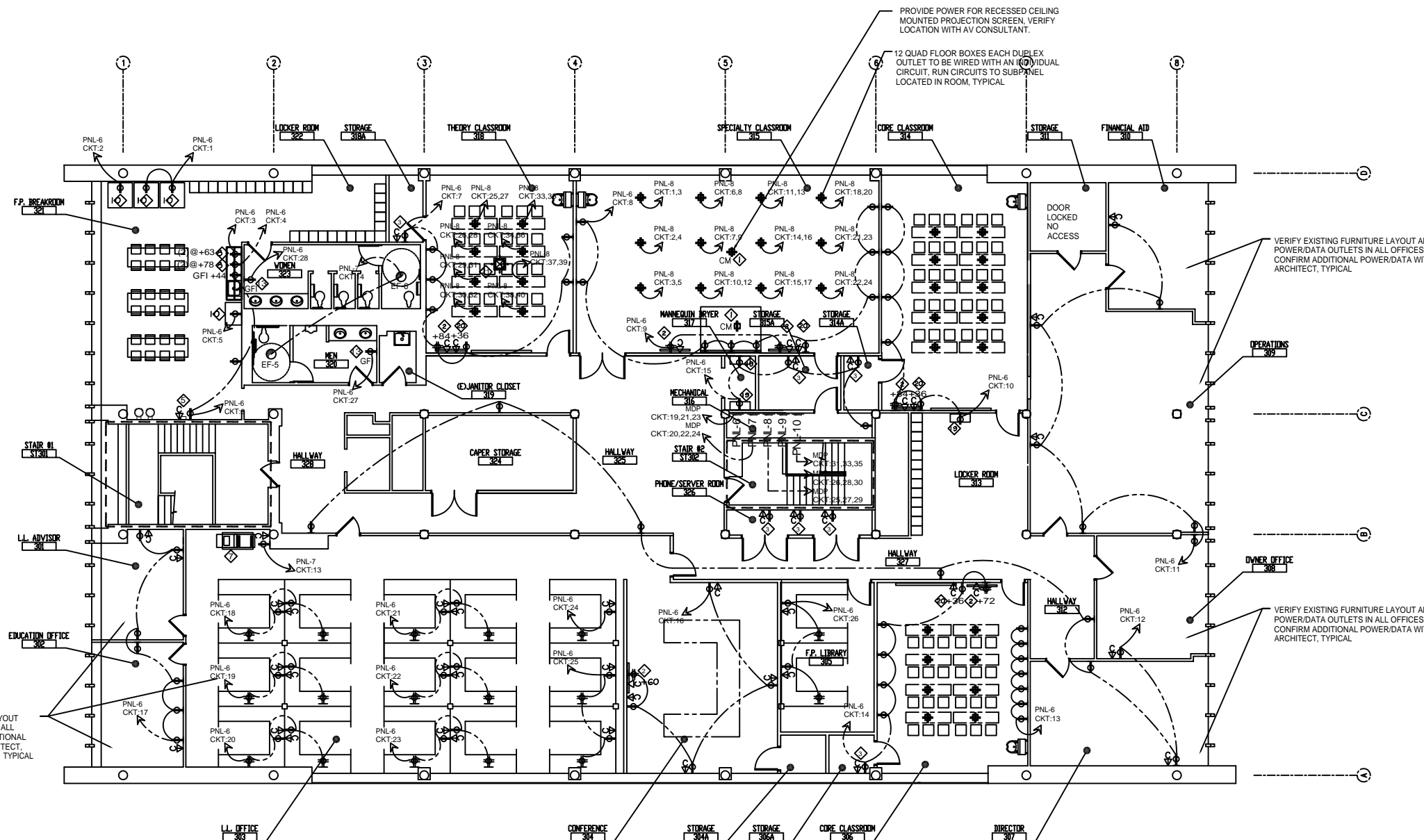
THIRD FLOOR POWER PLAN SCALE: 1/8"=1'
