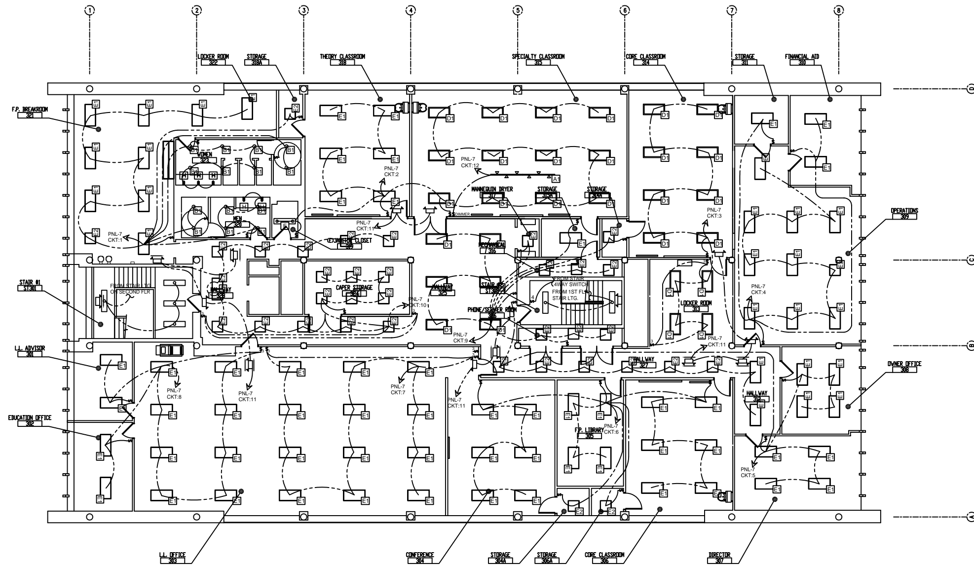
THIRD FLOOR LIGHTING PLAN SCALE: 1/8"=1'
