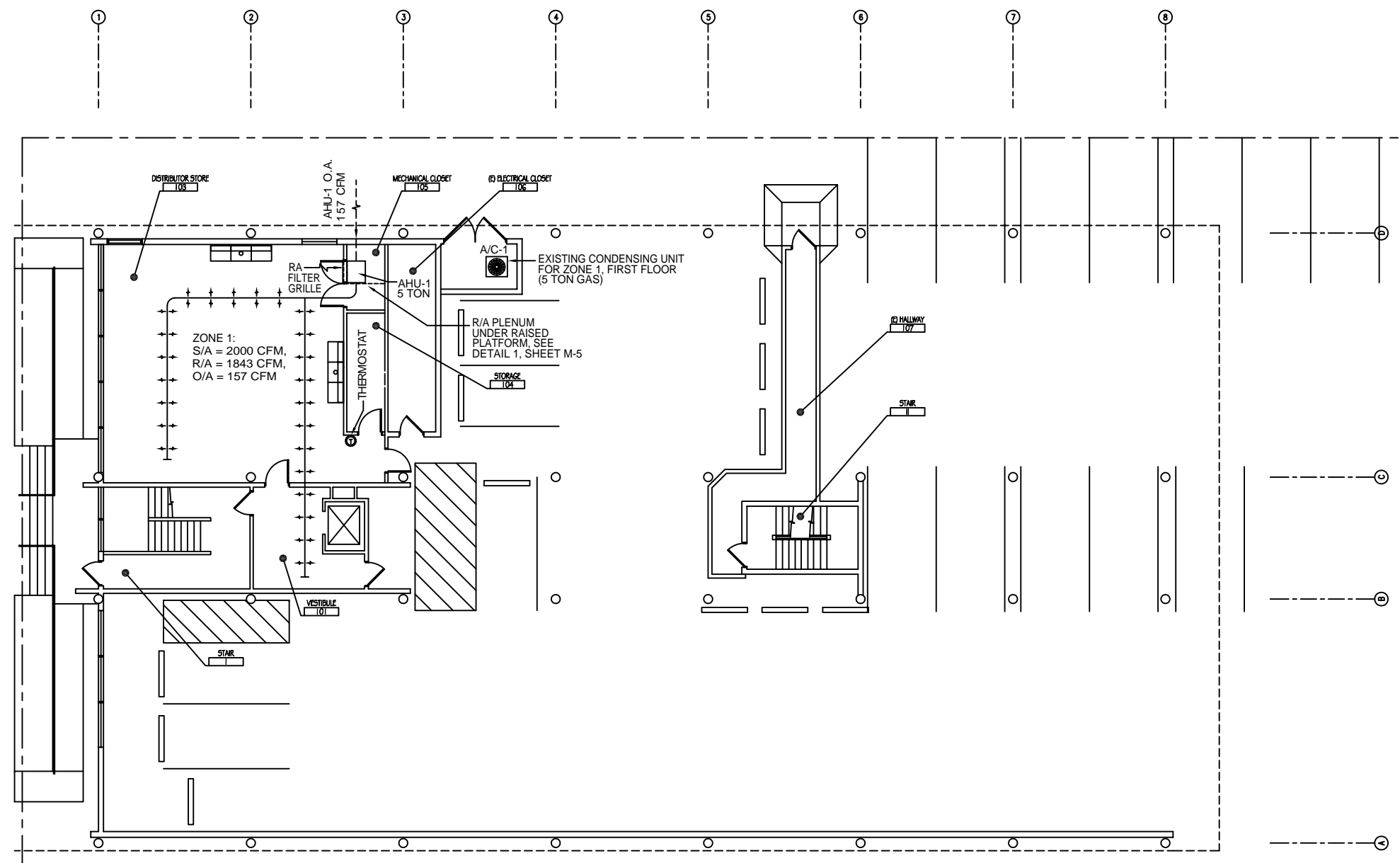
FIRST FLOOR MECHANICAL PLAN SCALE: 1/8"=1'
