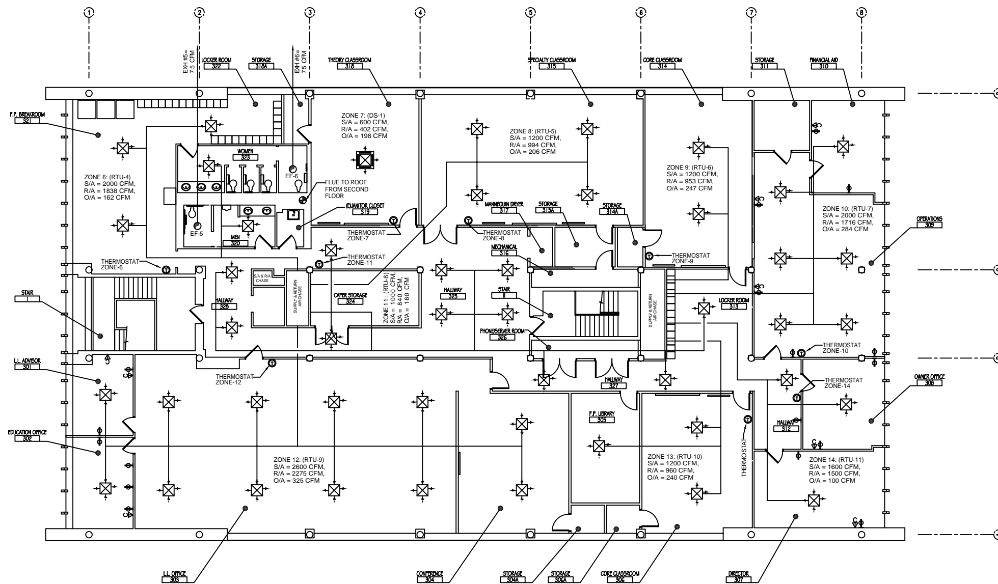
THIRD FLOOR MECHANICAL PLAN SCALE: 1/8"=1'
