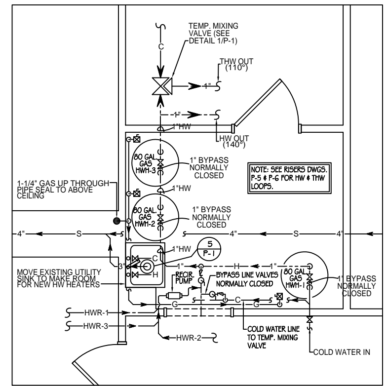
WATER HEATER ROOM LAYOUT PLAN NOT TO SCALE
