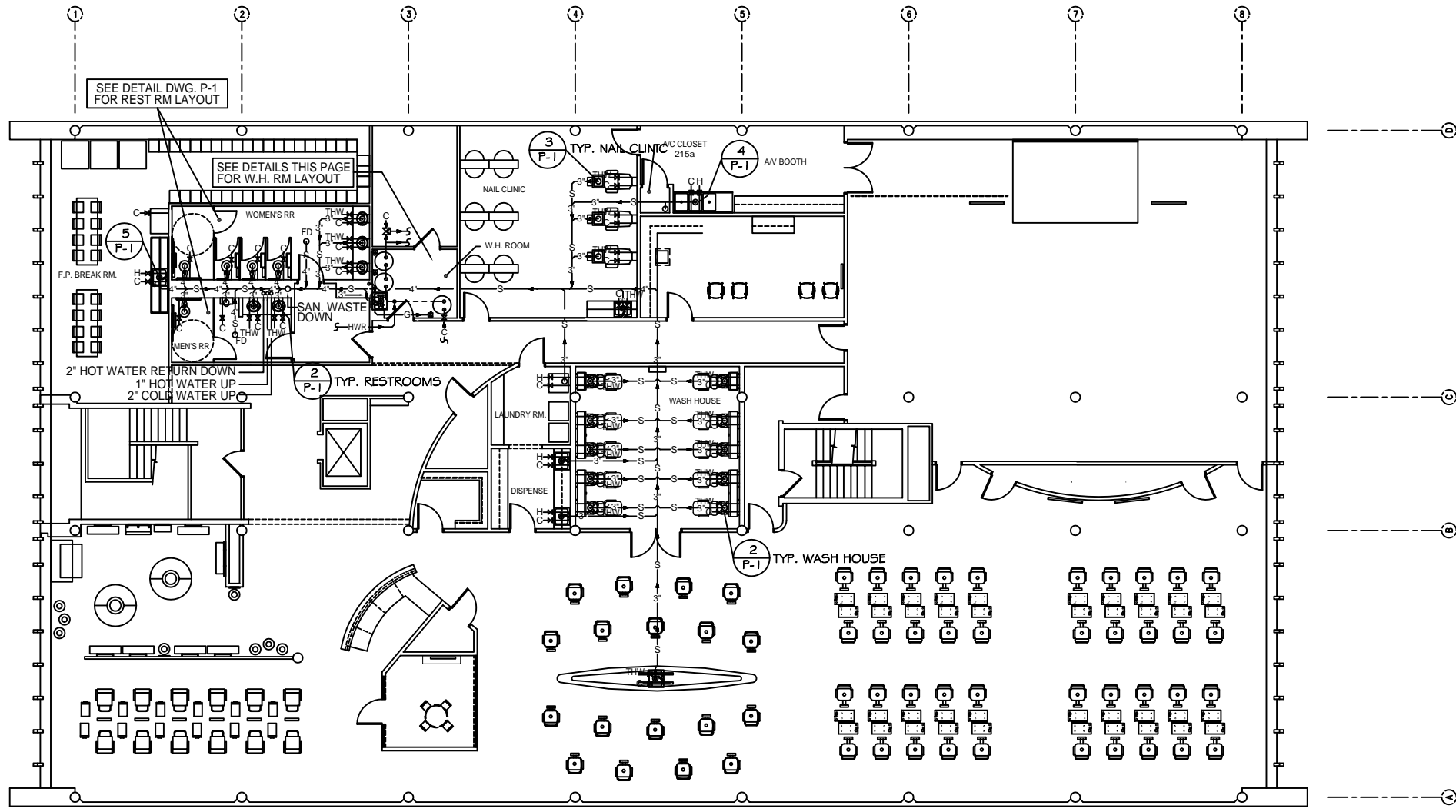
SECOND FLOOR PLUMBING PLAN SCALE: 1/8"=1'
