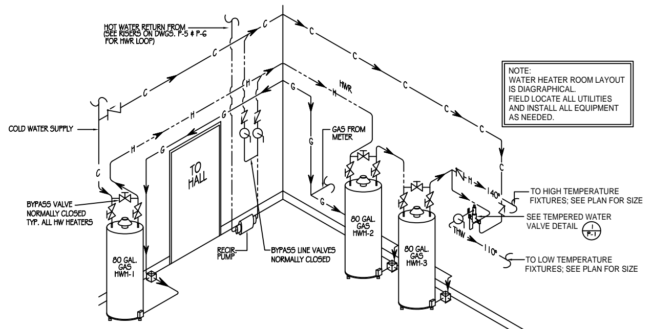
WATER HEATER ROOM LAYOUT DETAIL NOT TO SCALE
