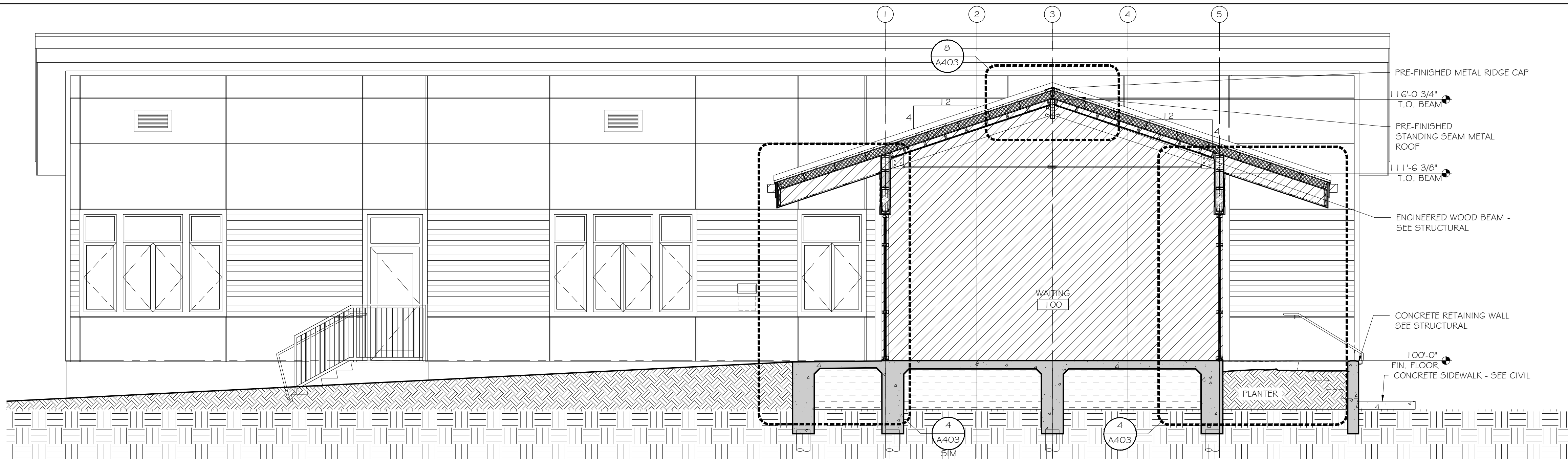
3 BUILDING SECTION A201 | A401 SCALE: 1/4" = 1'-0"
