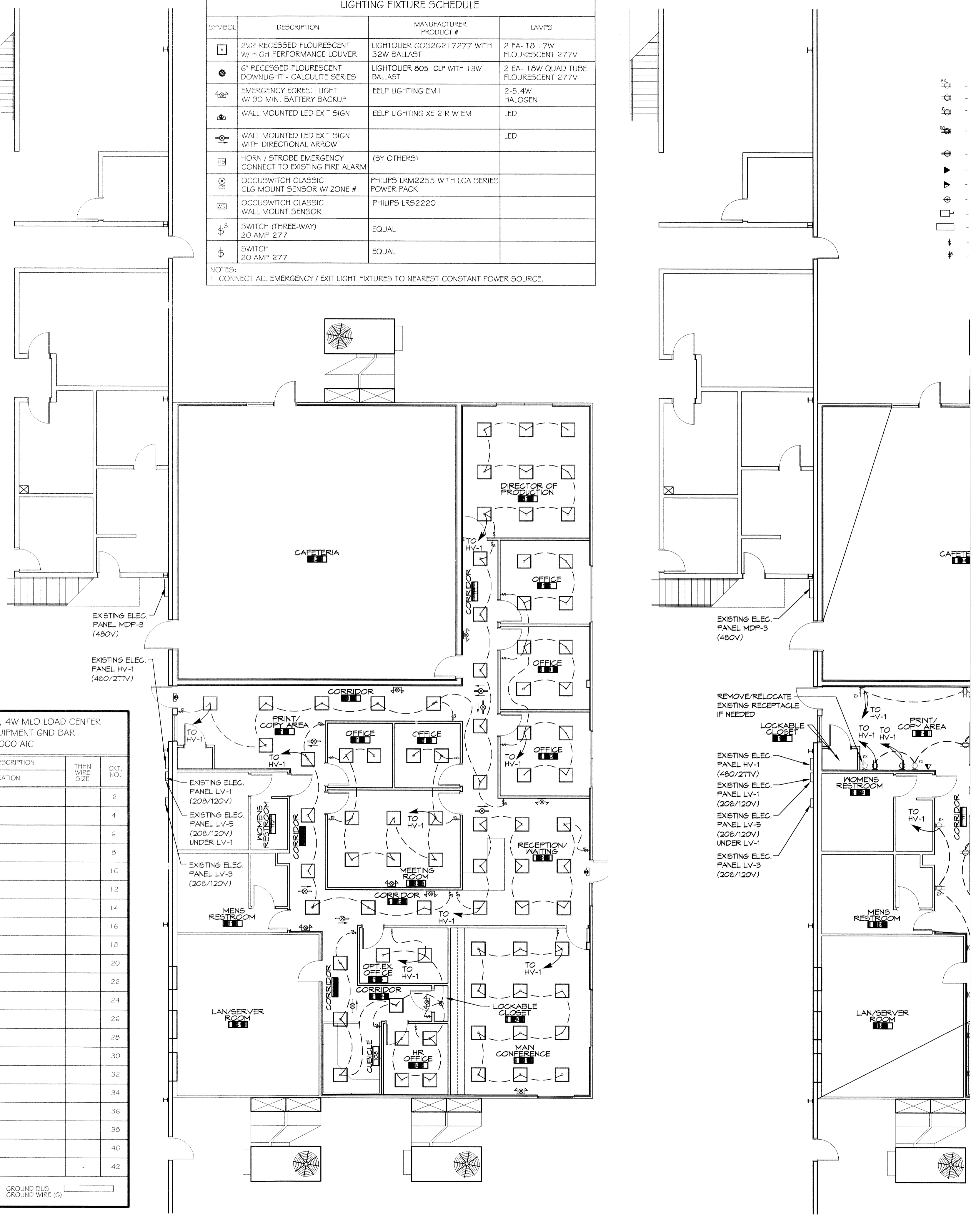
2 ELECTRICAL LIGHTING PLAN SCALE: 1/8" = 1'-0"
