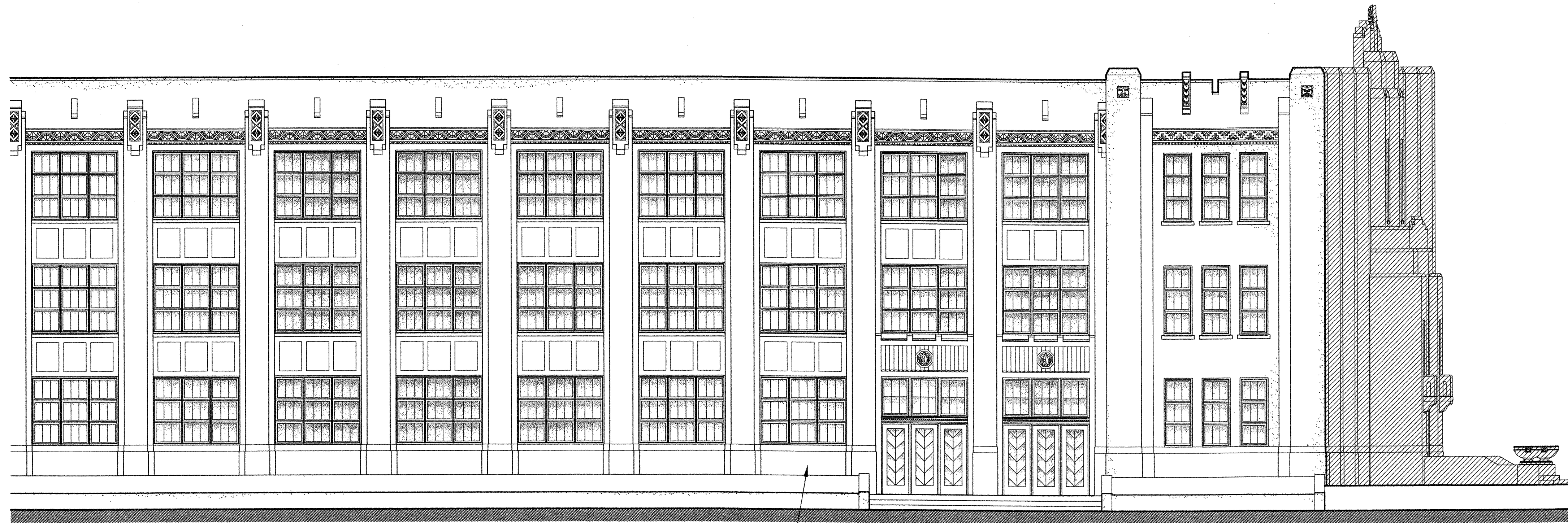
NEW CLINIC (AREA OF WORK INSIDE EXISTING BUILDING) JOSEPH STREET ELEVATION
