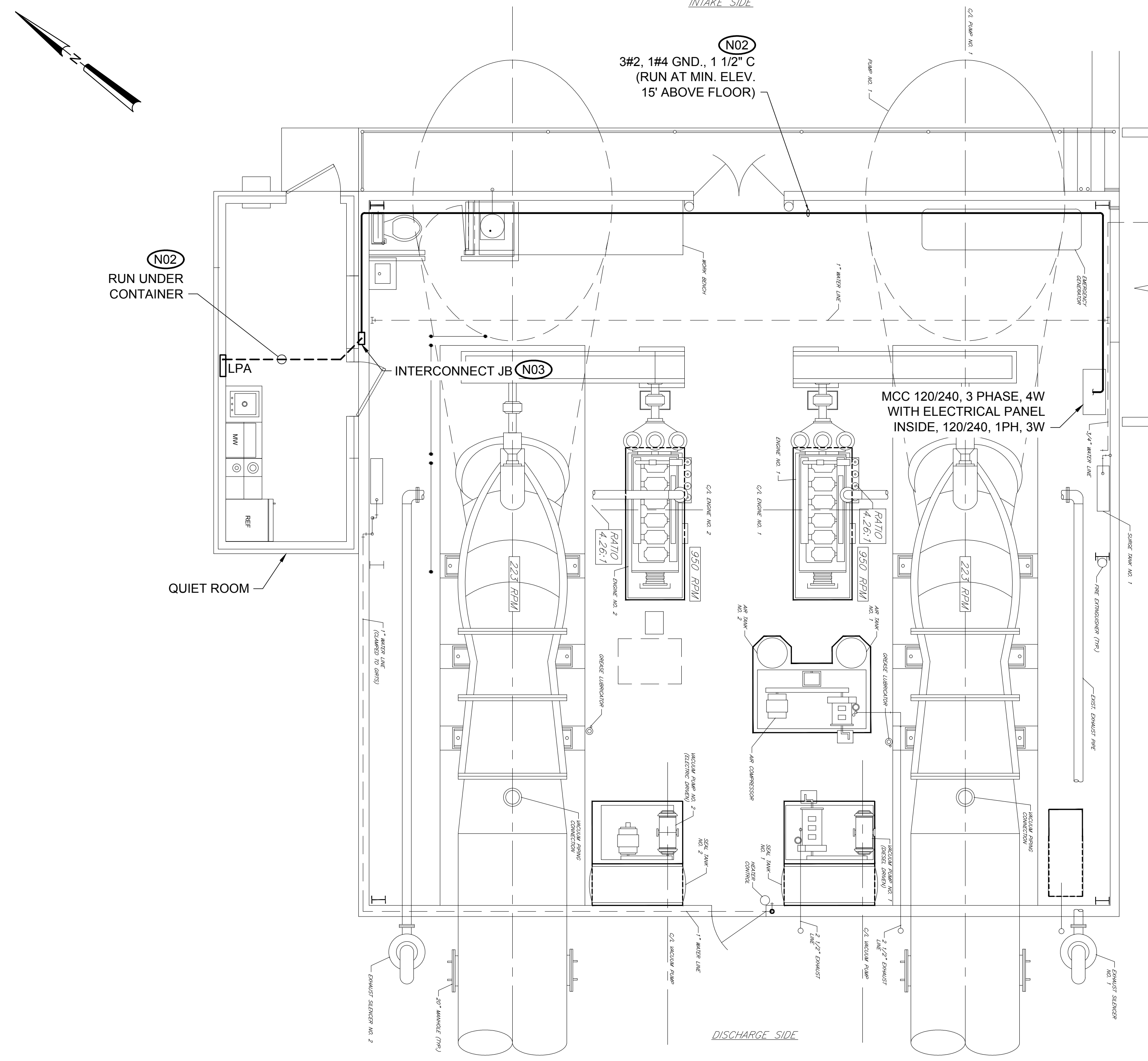
ELECTRICAL CONDUIT PLAN SCALE: 1/4" = 1'-0"
