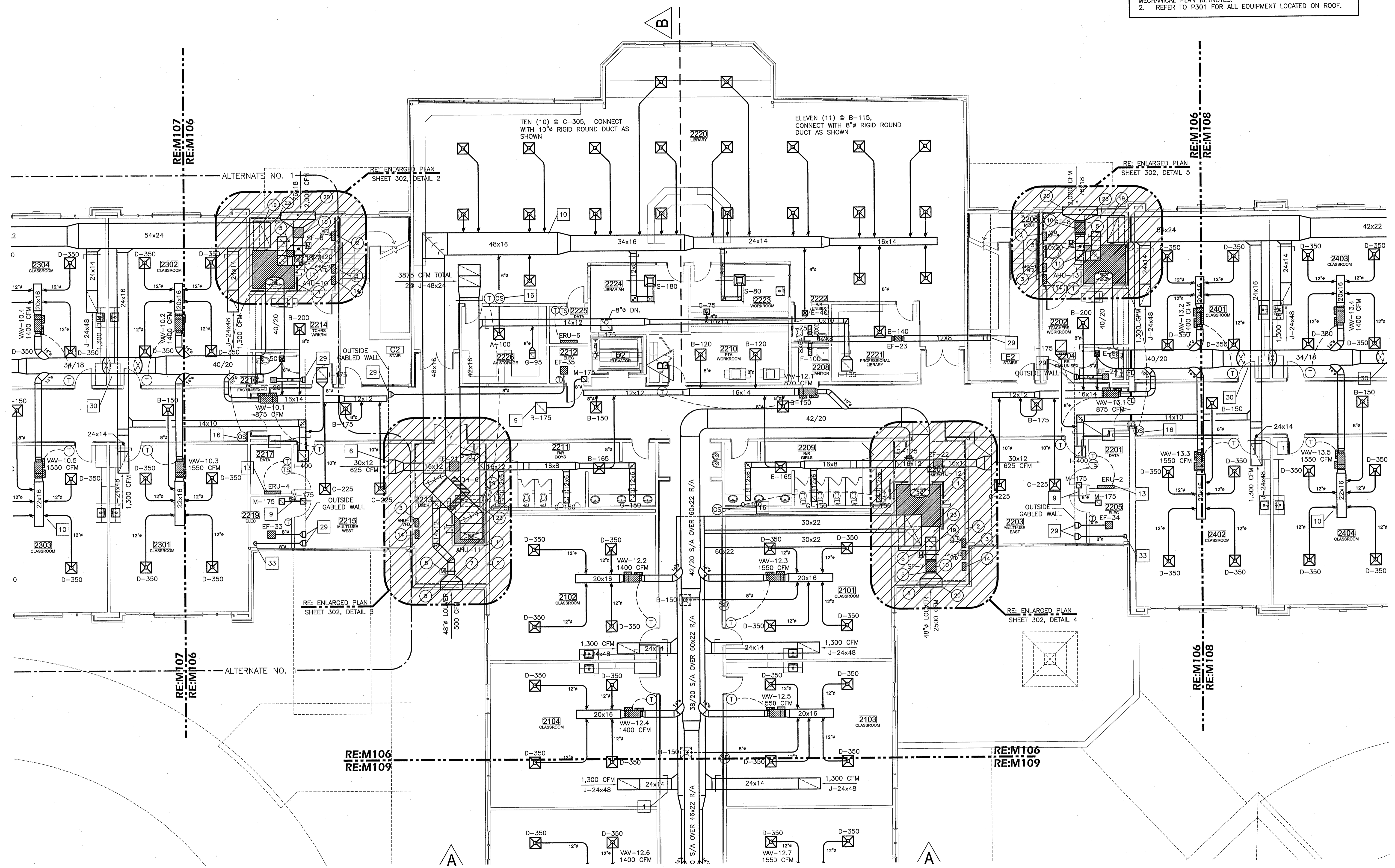
1 PARTIAL 2nd FLOOR PLAN - MECHANICAL Scale: 1/8"=1'-0"
