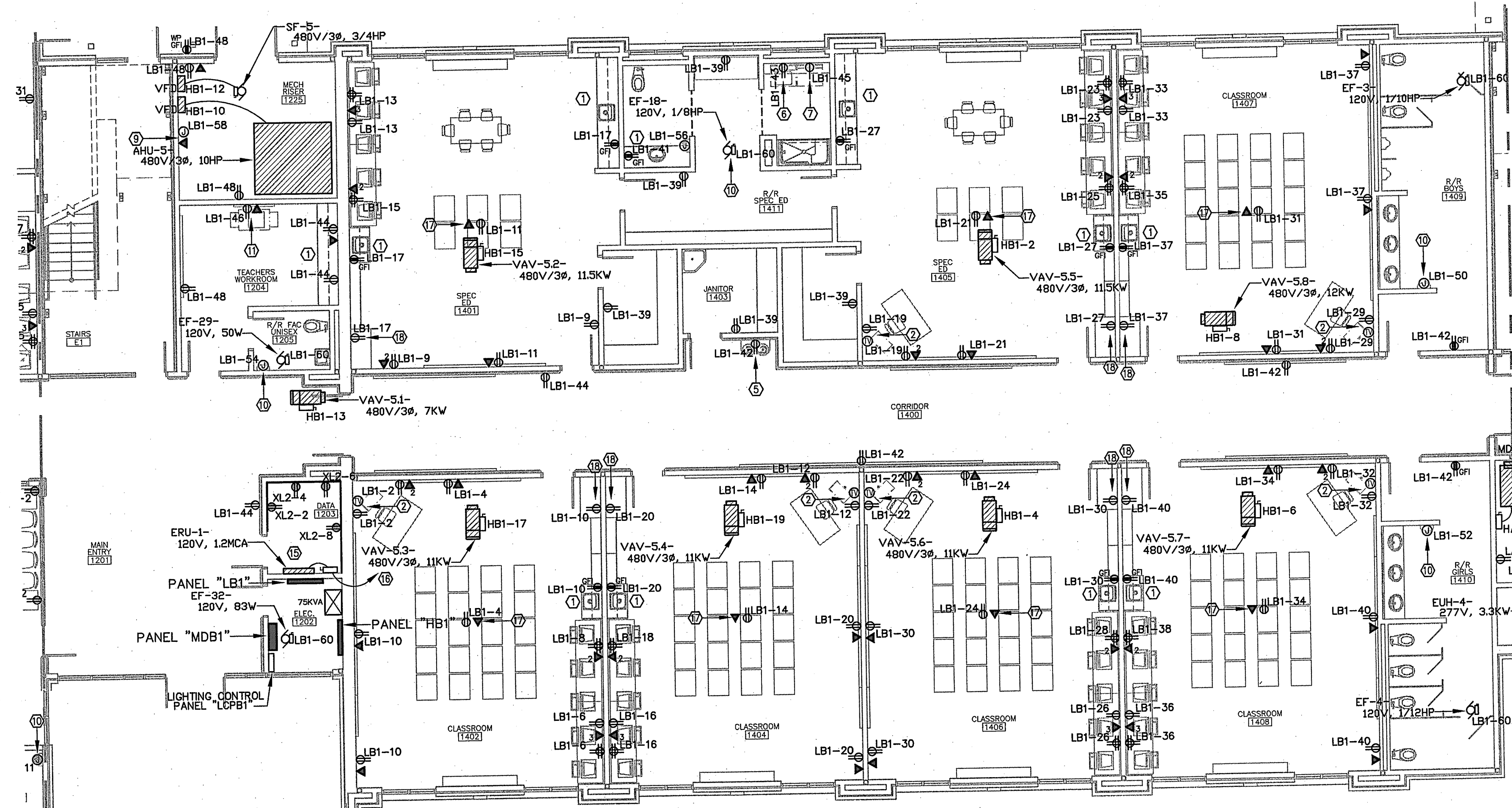
2 POWER PLAN- FIRST FLOOR WING 1400 SCALE: 1/8" = 1'-0"
