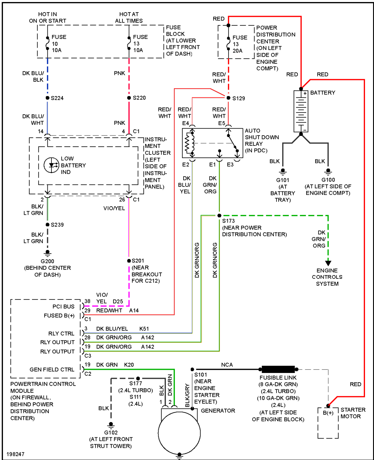
Fig. 51: Charging Circuit
