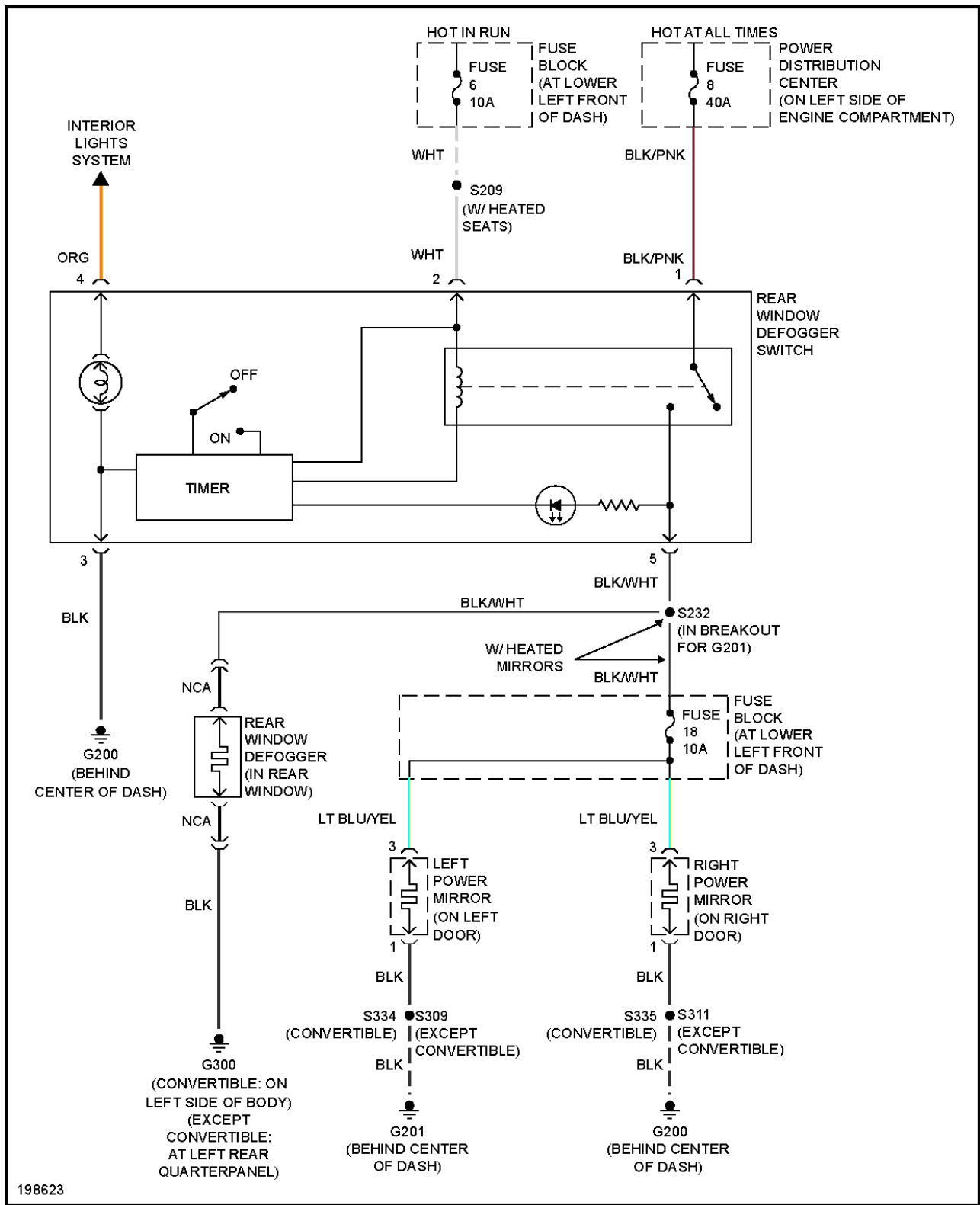
Fig. 10: Defoggers Circuit
