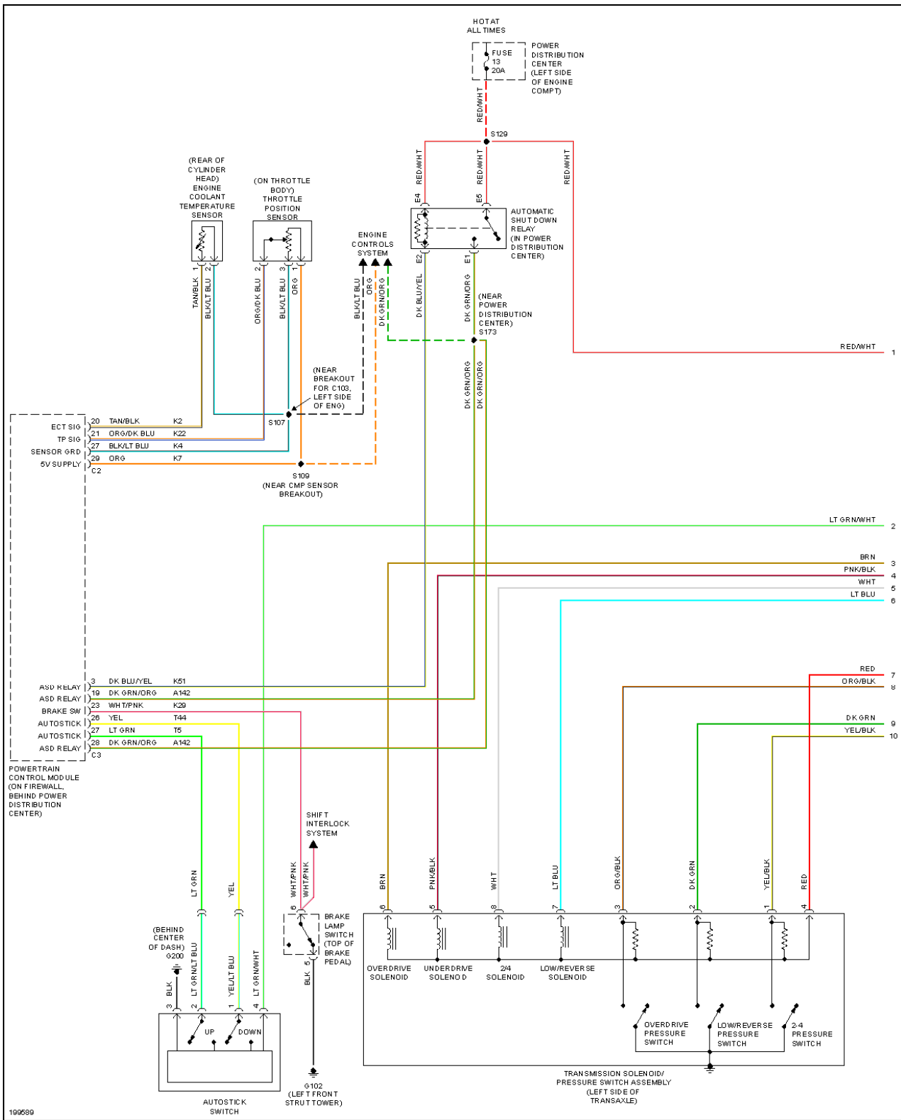
Fig. 57: 2.4L Turbo, A/T Circuit (1 of 2)
