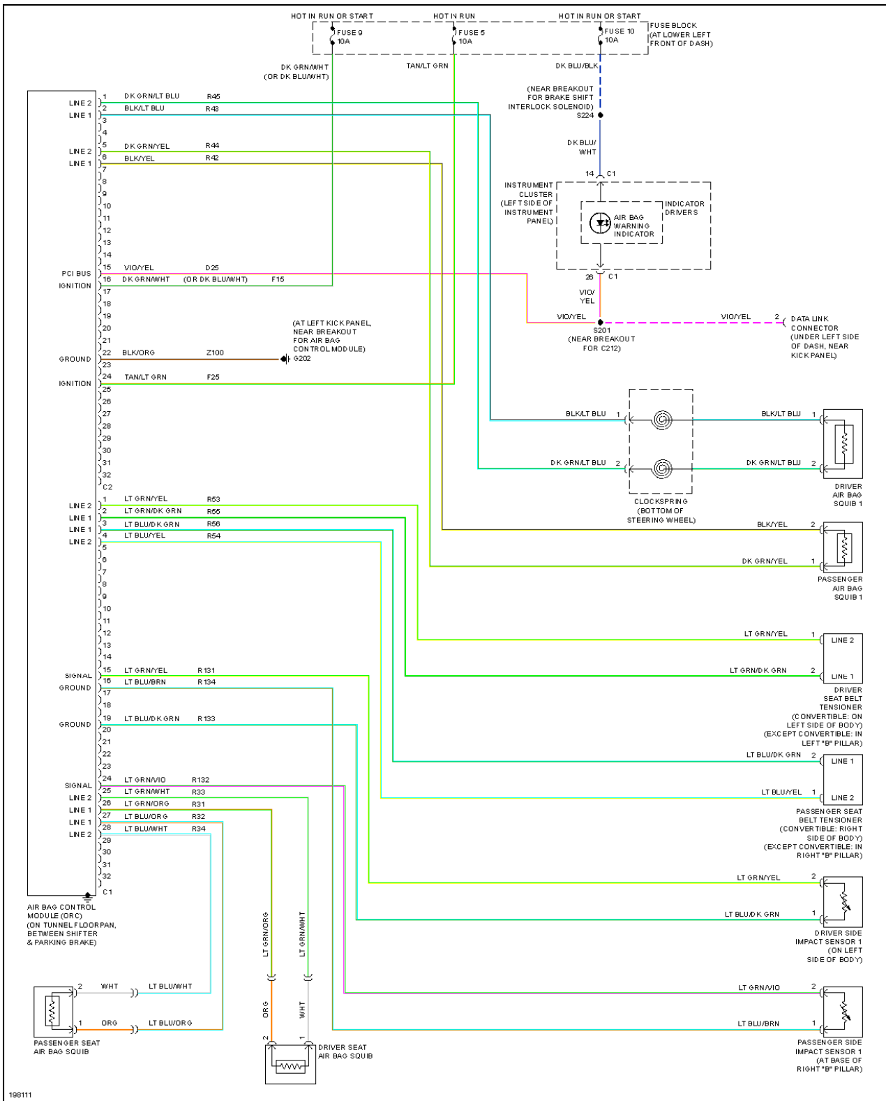
Fig. 54: Supplemental Restraints Circuit, Premium
