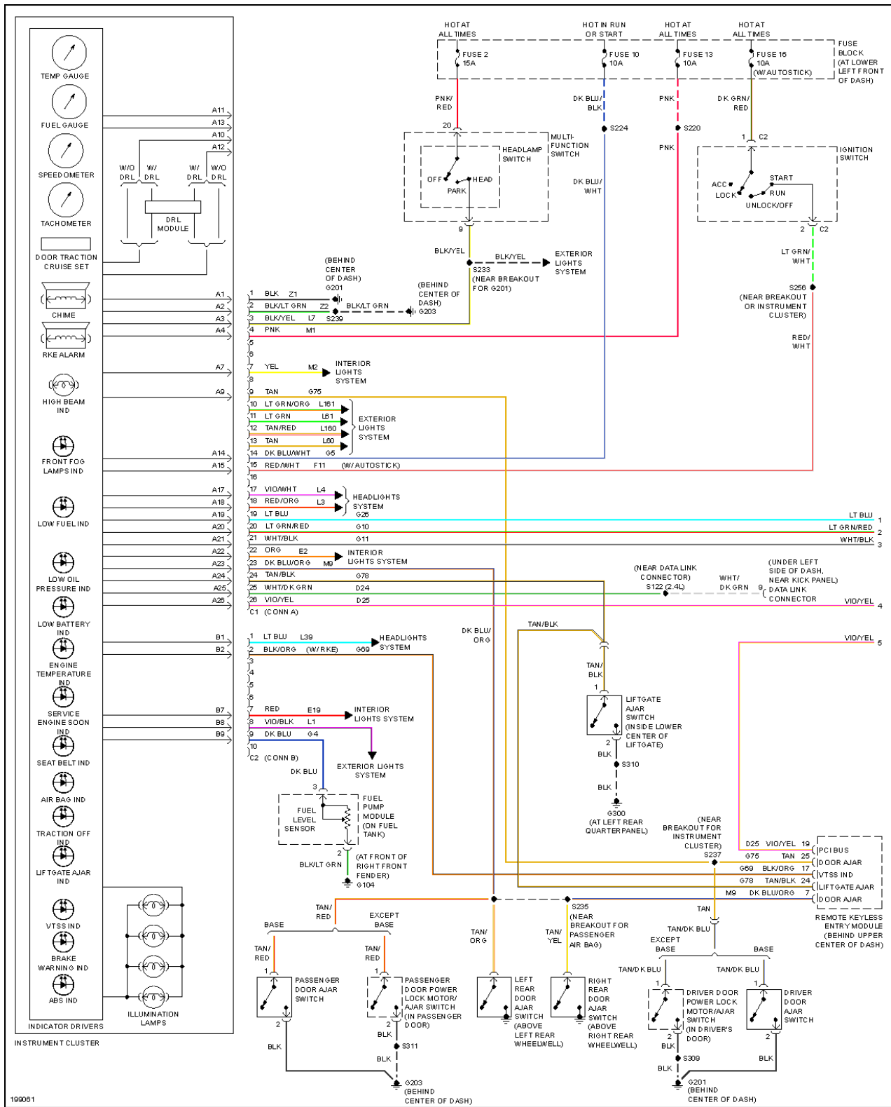
Fig. 26: Instrument Cluster Circuit, Except Convertible (1 of 2)
