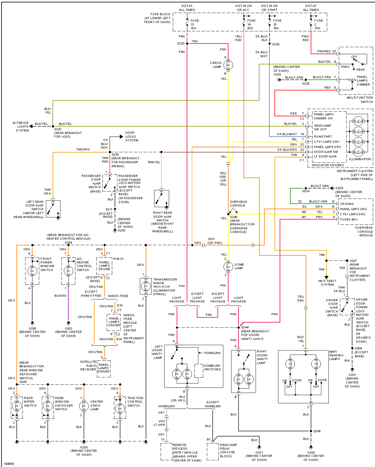
Fig. 31: Interior Lights Circuit, Except Convertible
