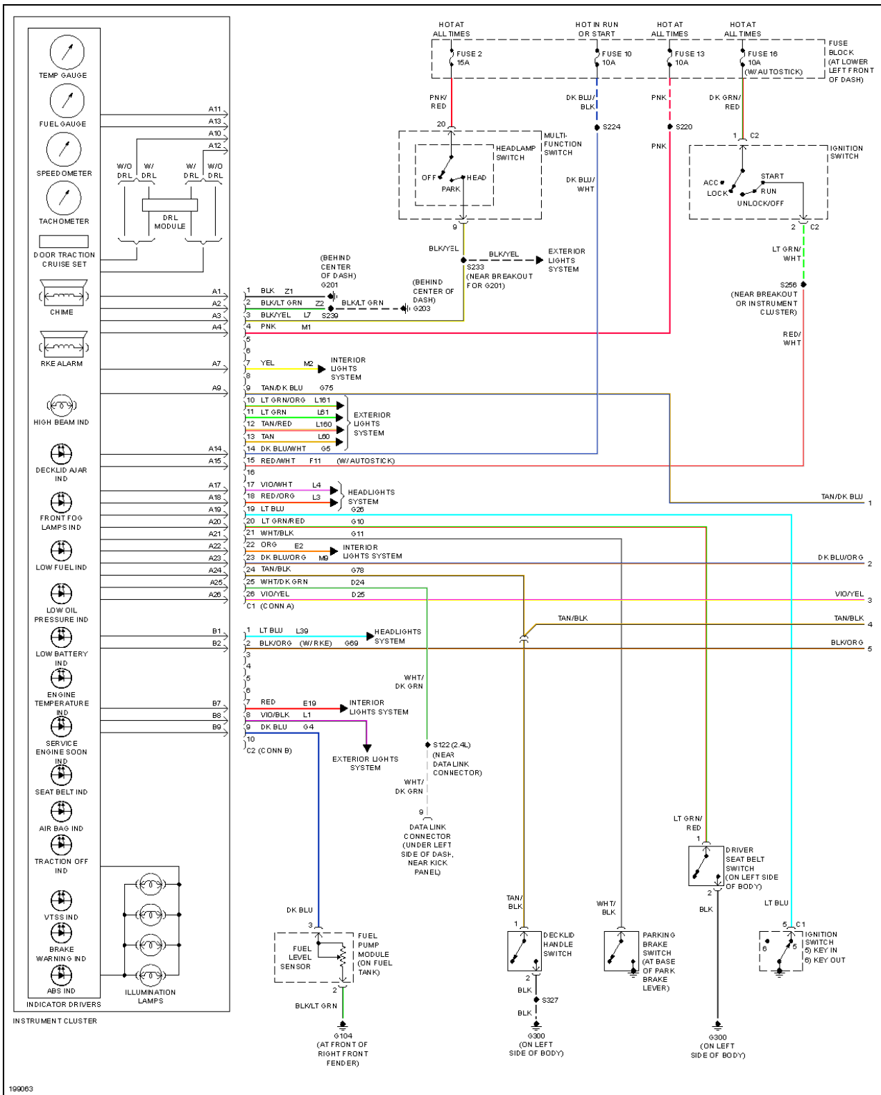
Fig. 24: Instrument Cluster Circuit, Convertible (1 of 2)
