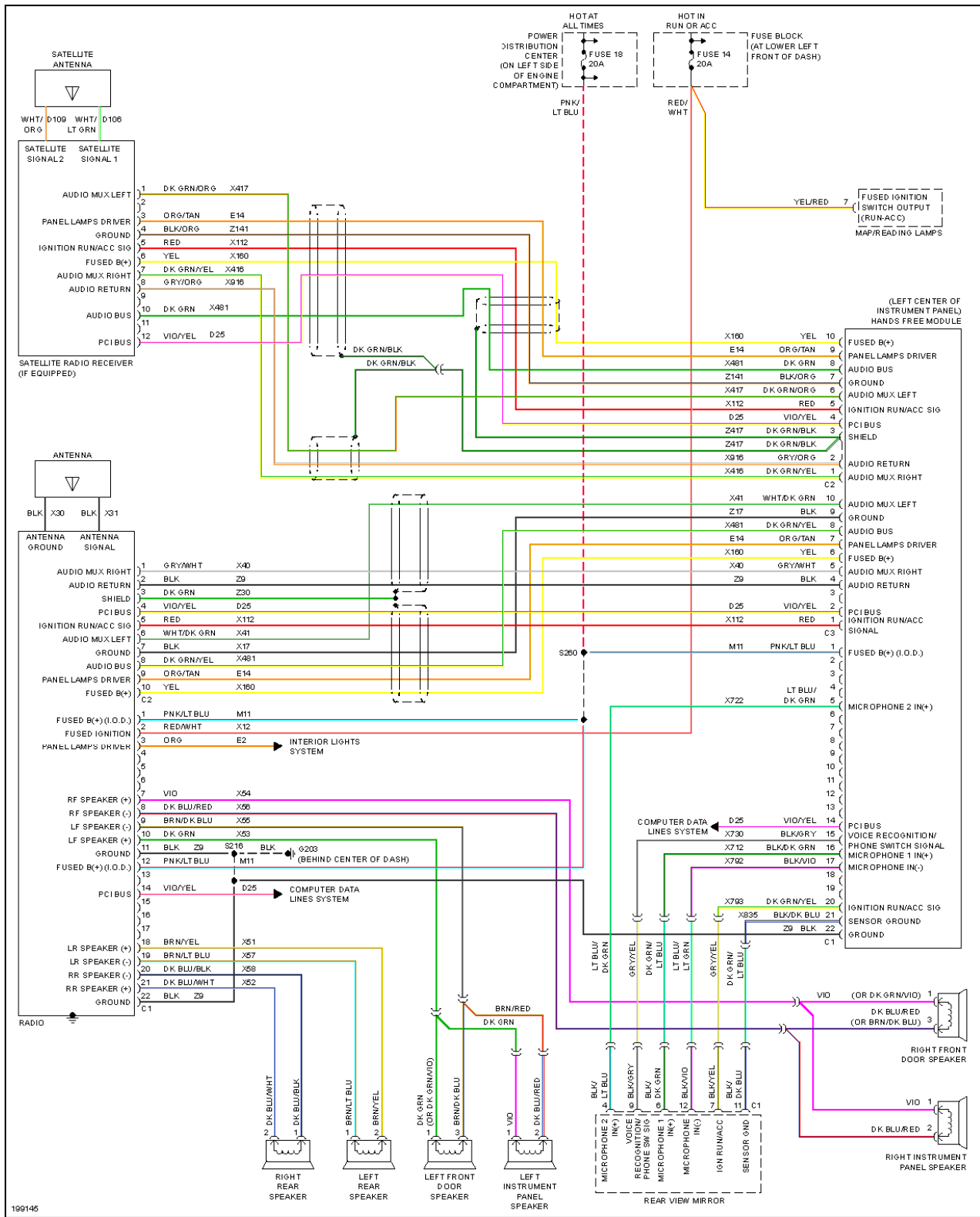
Fig. 48: Radio Circuit, Except Convertible W/ Hands Free
