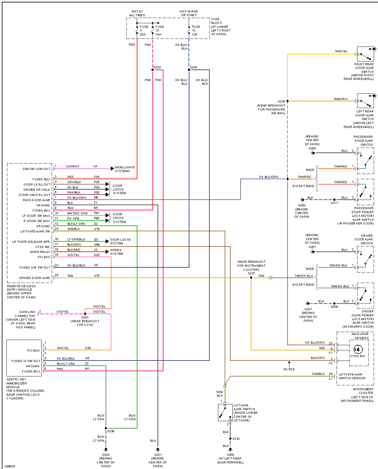
Fig. 5: Anti-theft Circuit, Except Convertible
