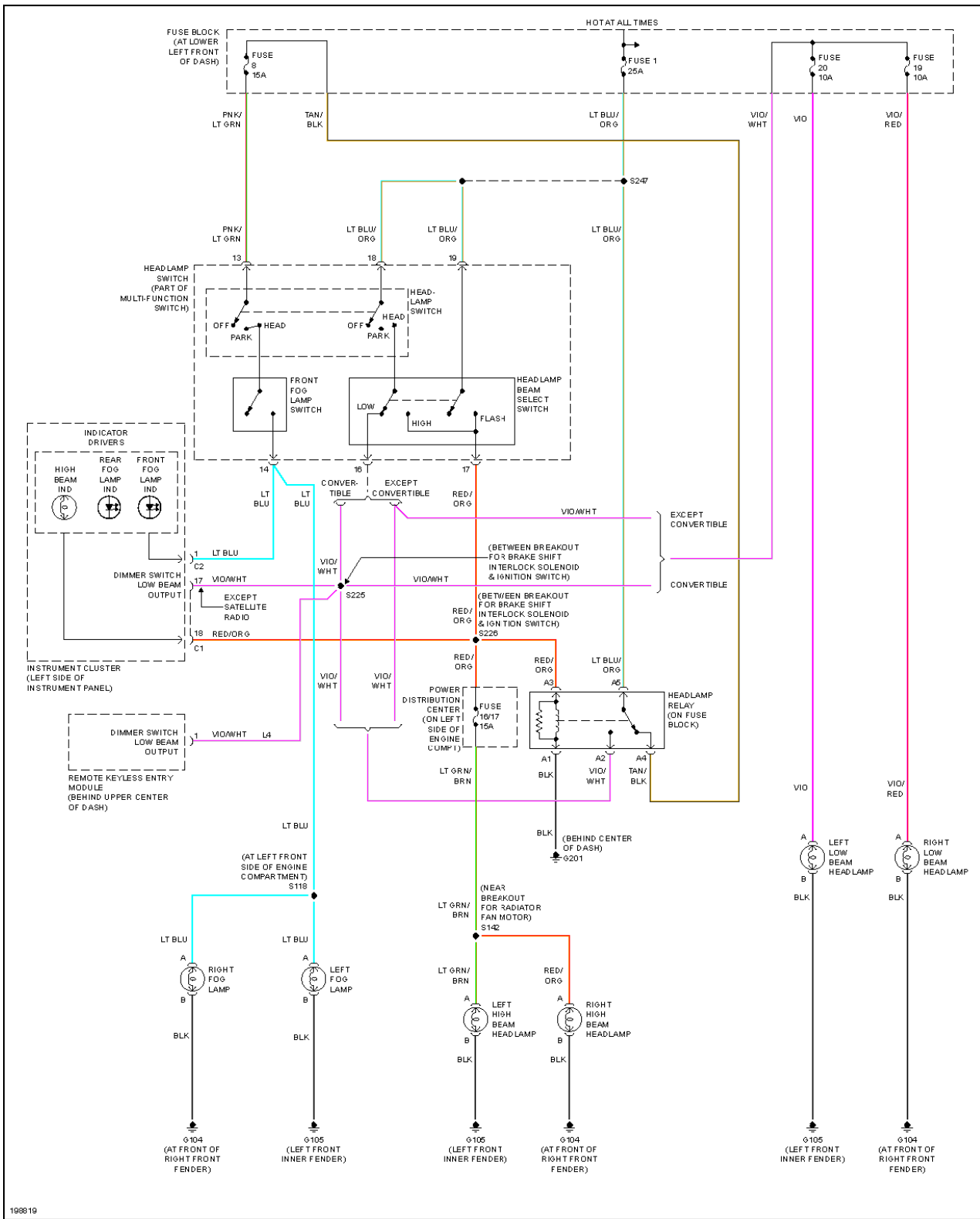
Fig. 22: Headlights Circuit
