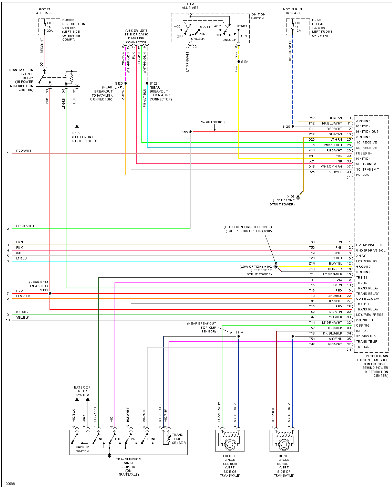
Fig. 56: 2.4L, A/T Circuit (2 of 2)
