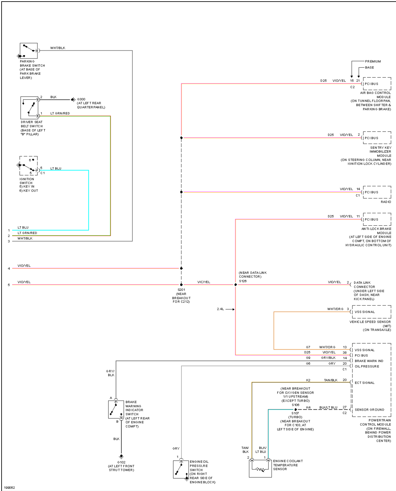
Fig. 27: Instrument Cluster Circuit, Except Convertible (2 of 2)
