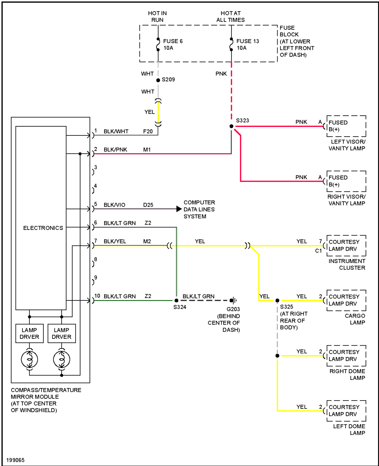
Fig. 28: Overhead Console Circuit, Convertible
