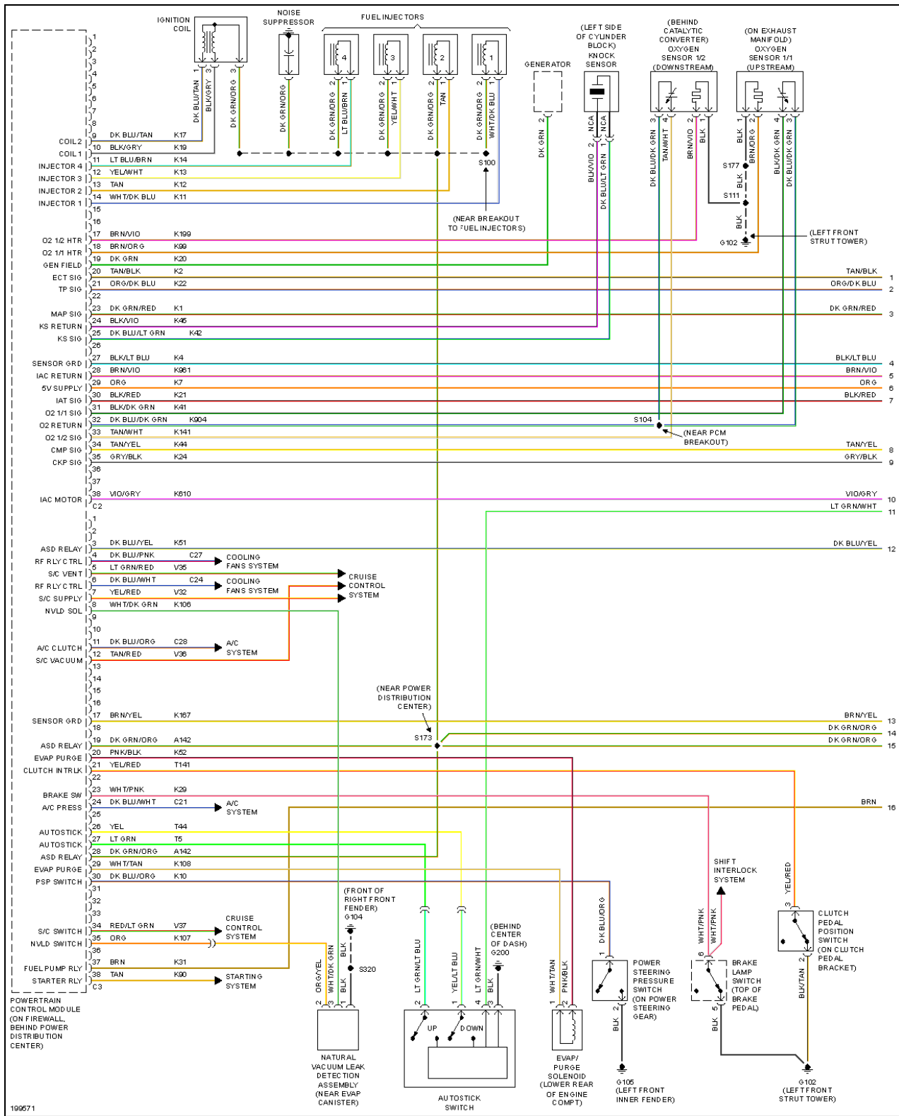
Fig. 14: 2.4L Turbo, Engine Performance Circuit (1 of 3)
