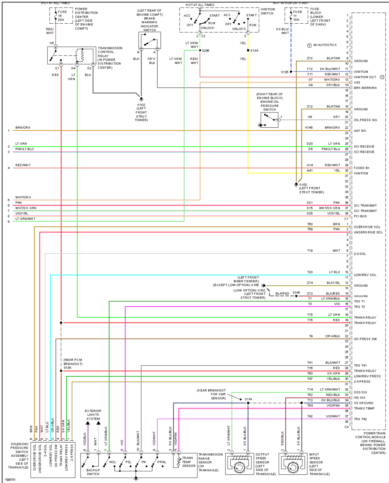
Fig. 13: 2.4L, Engine Performance Circuit (3 of 3)
