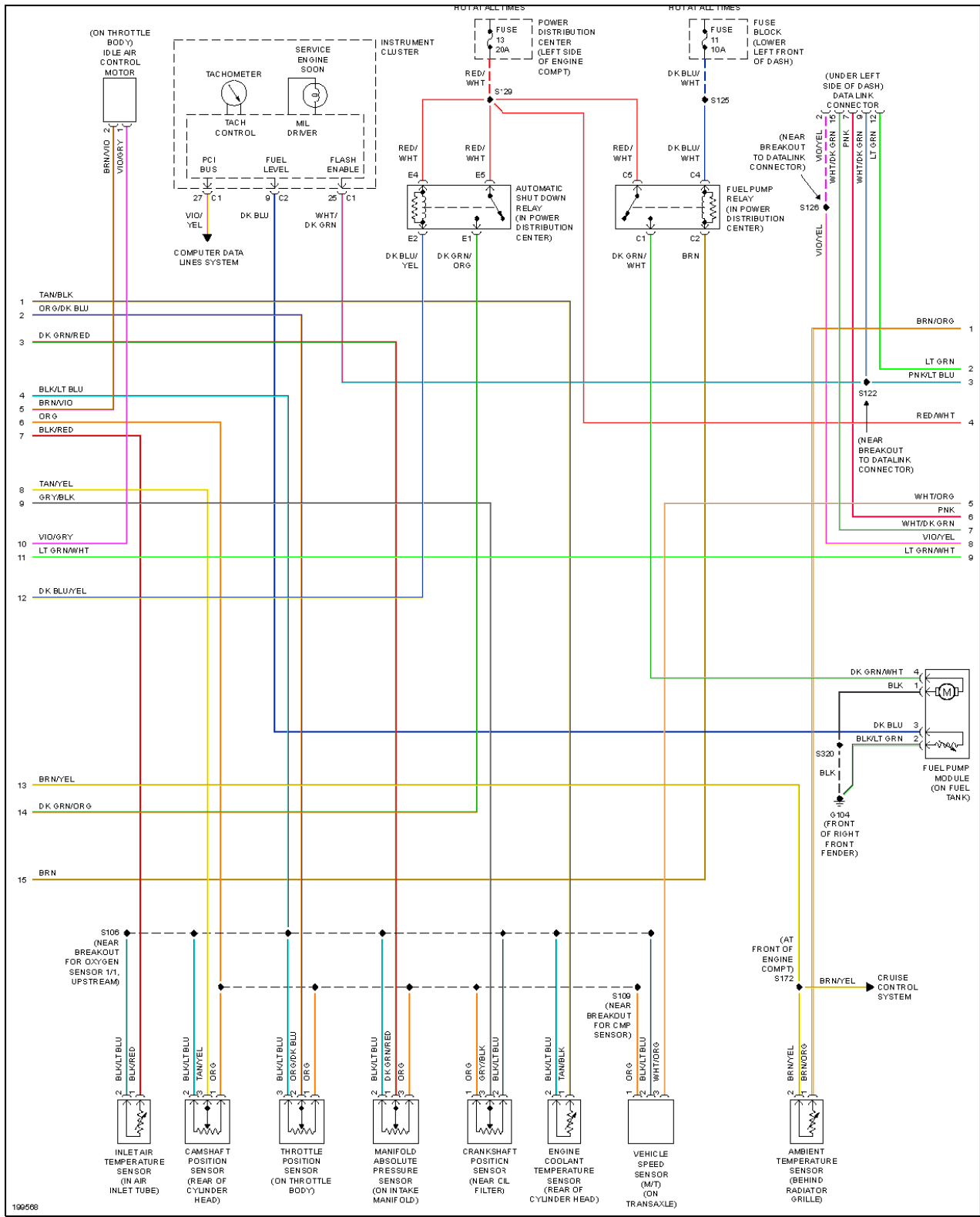
Fig. 12: 2.4L, Engine Performance Circuit (2 of 3)
