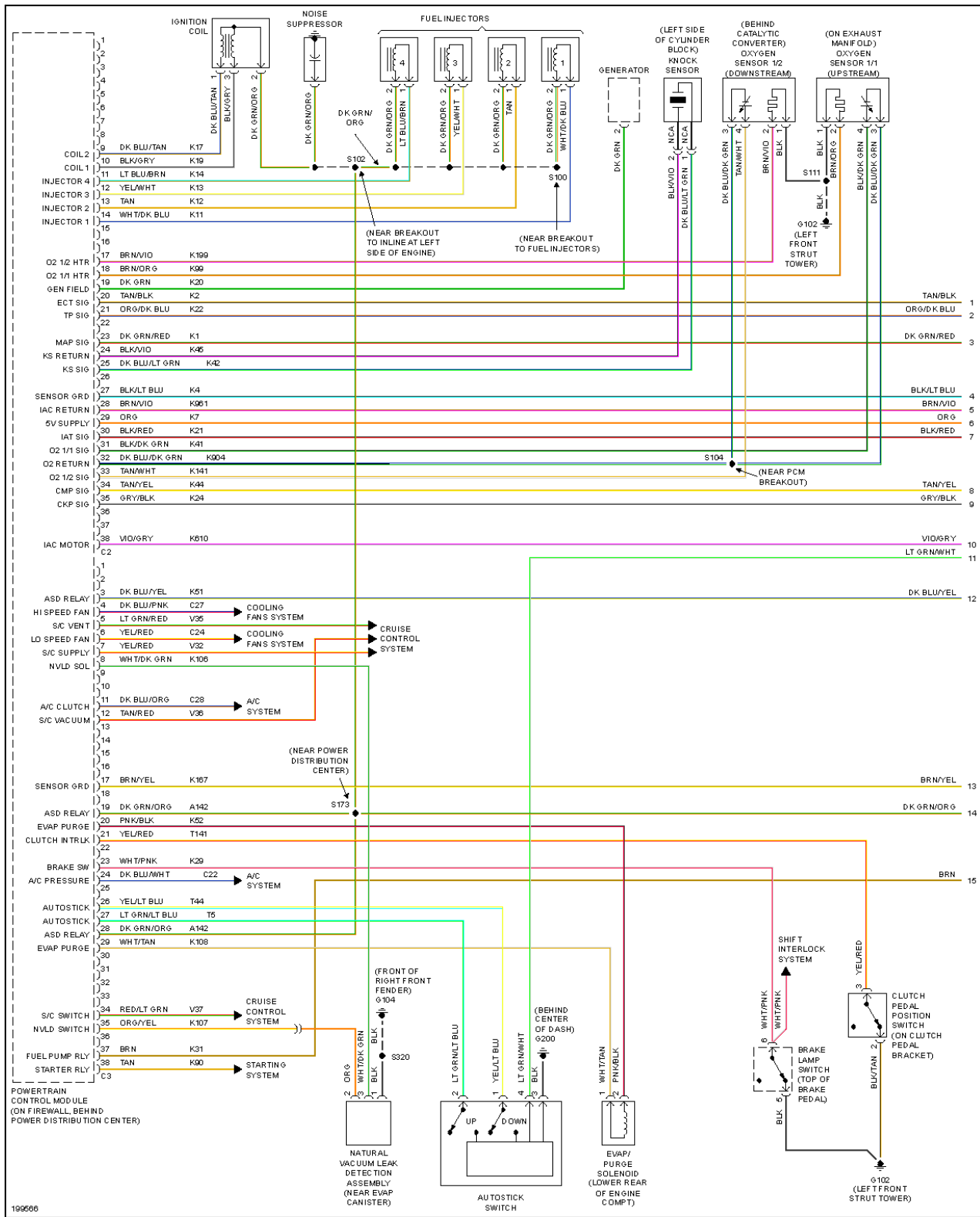
Fig. 11: 2.4L, Engine Performance Circuit (1 of 3)
