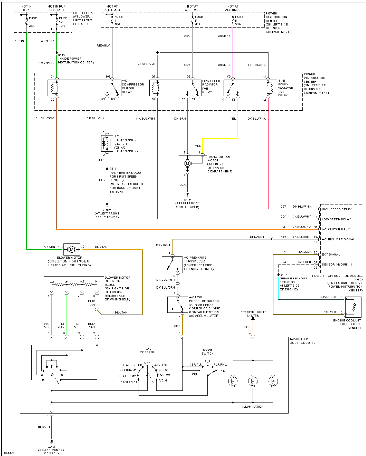
Fig. 2: 2.4L Turbo, Manual A/C Circuit
