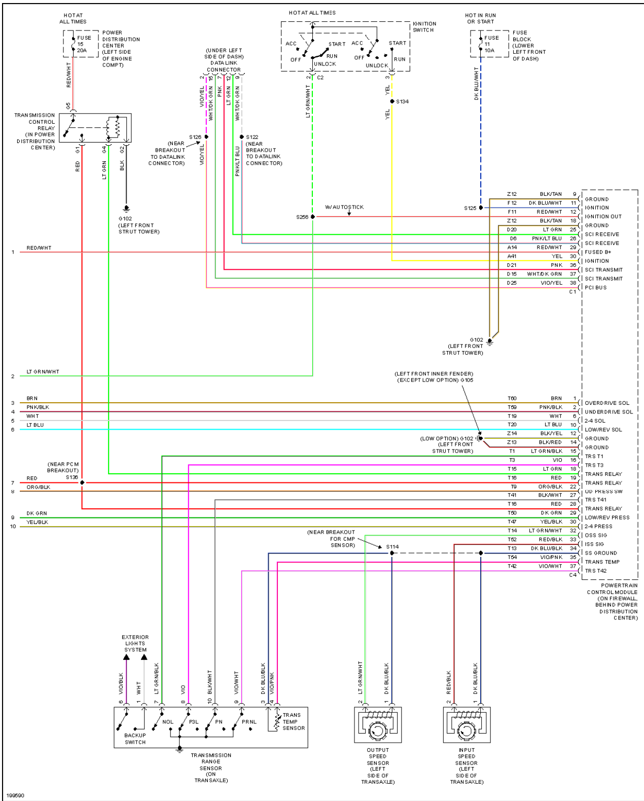
Fig. 58: 2.4L Turbo, A/T Circuit (2 of 2)
