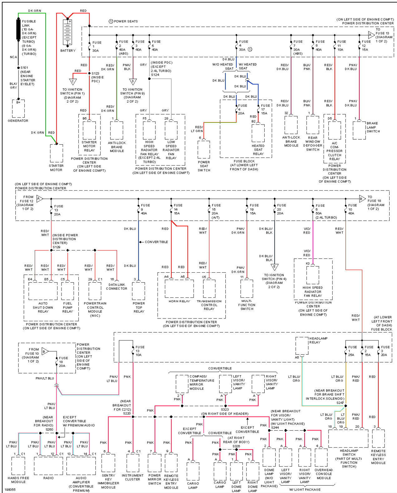
Fig. 32: Power Distribution Circuit (1 of 2)
