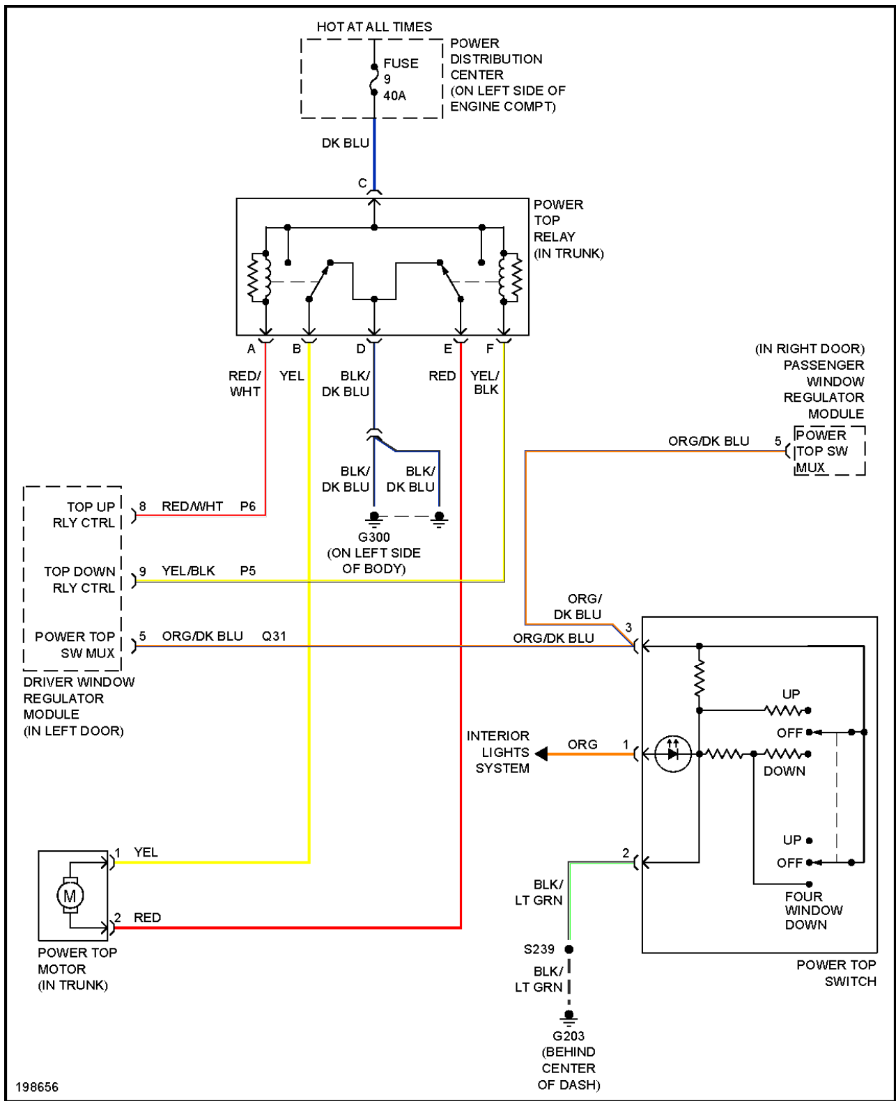
Fig. 39: Convertible Top Circuit
