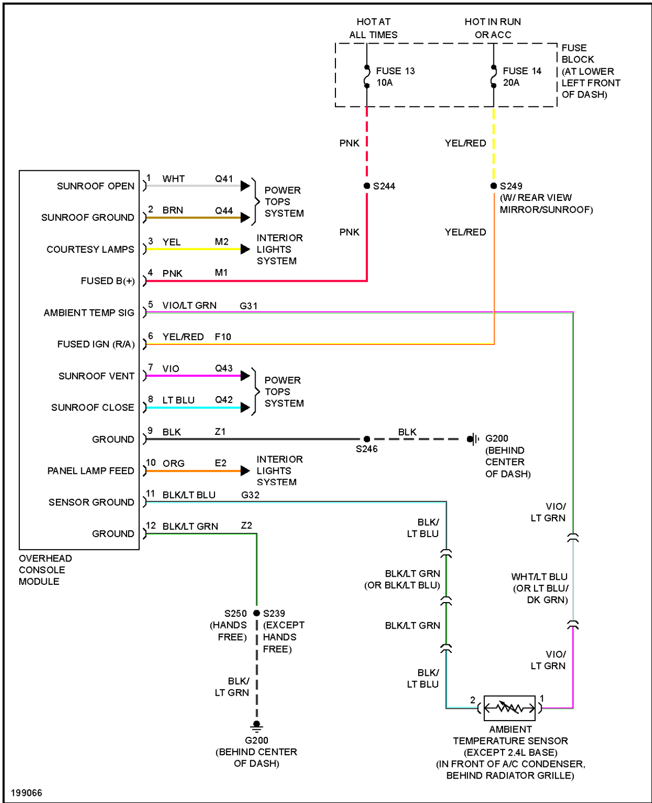
Fig. 29: Overhead Console Circuit, Except Convertible
