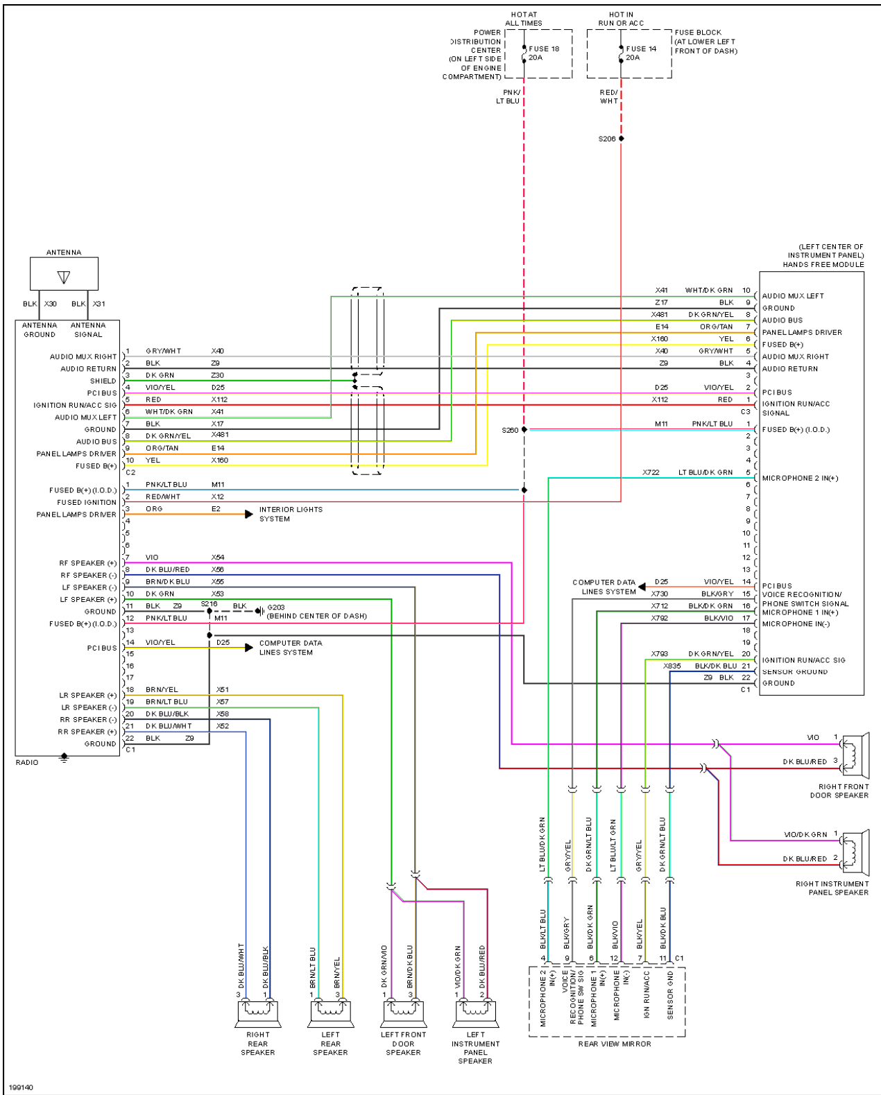
Fig. 43: Radio Circuit, Convertible Base Radio W/ Hands Free
