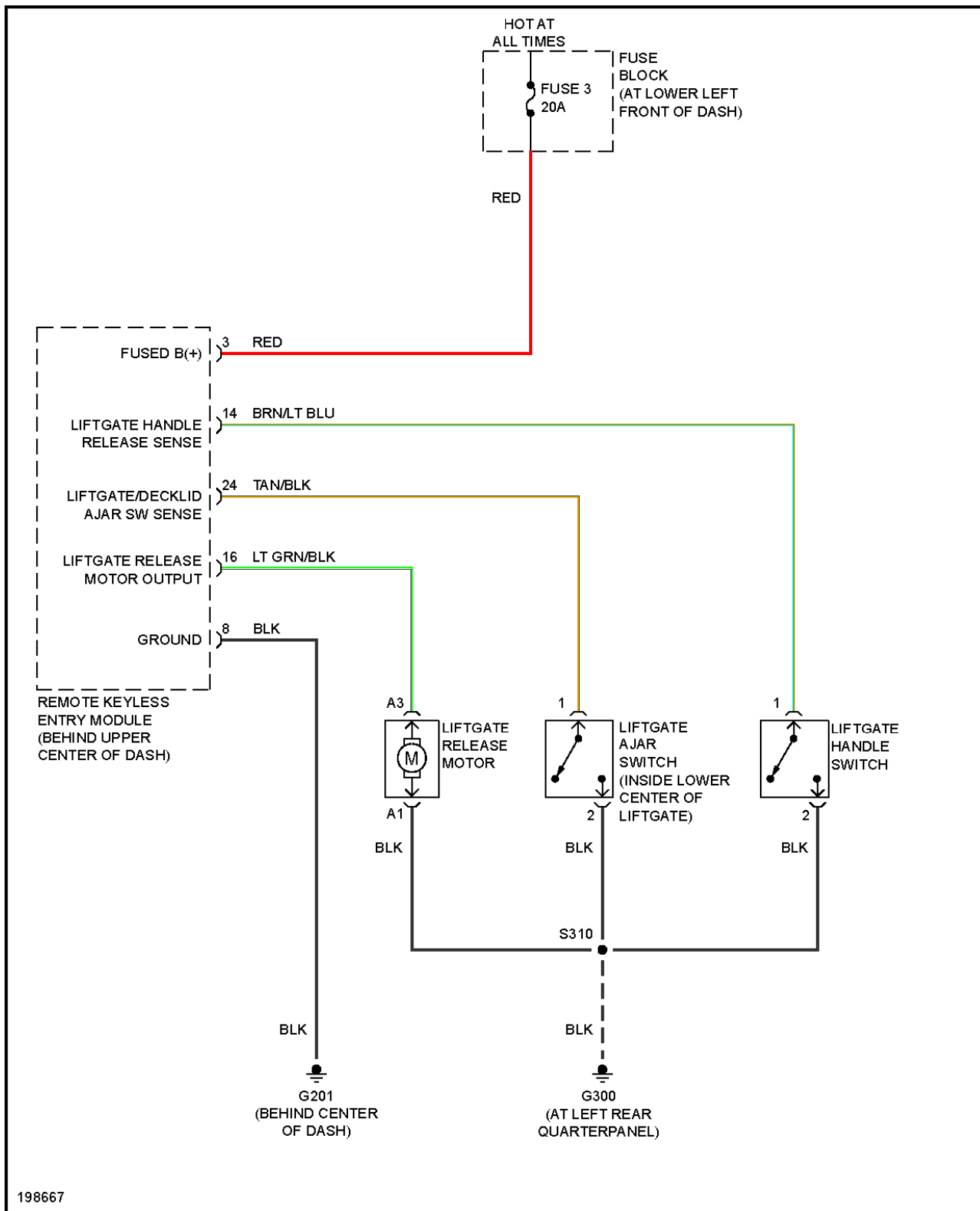
Fig. 59: Liftgate Release Circuit, Except Convertible
