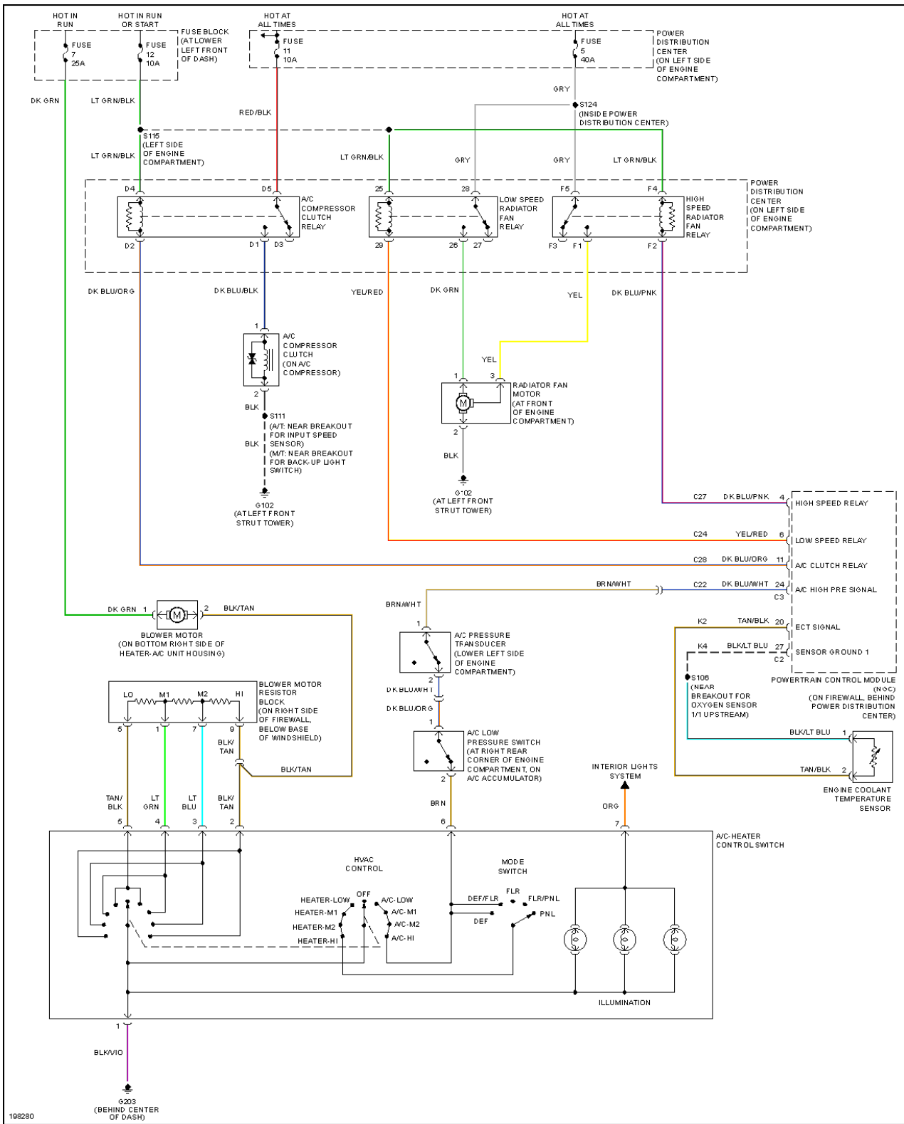
Fig. 1: 2.4L, Manual A/C Circuit
