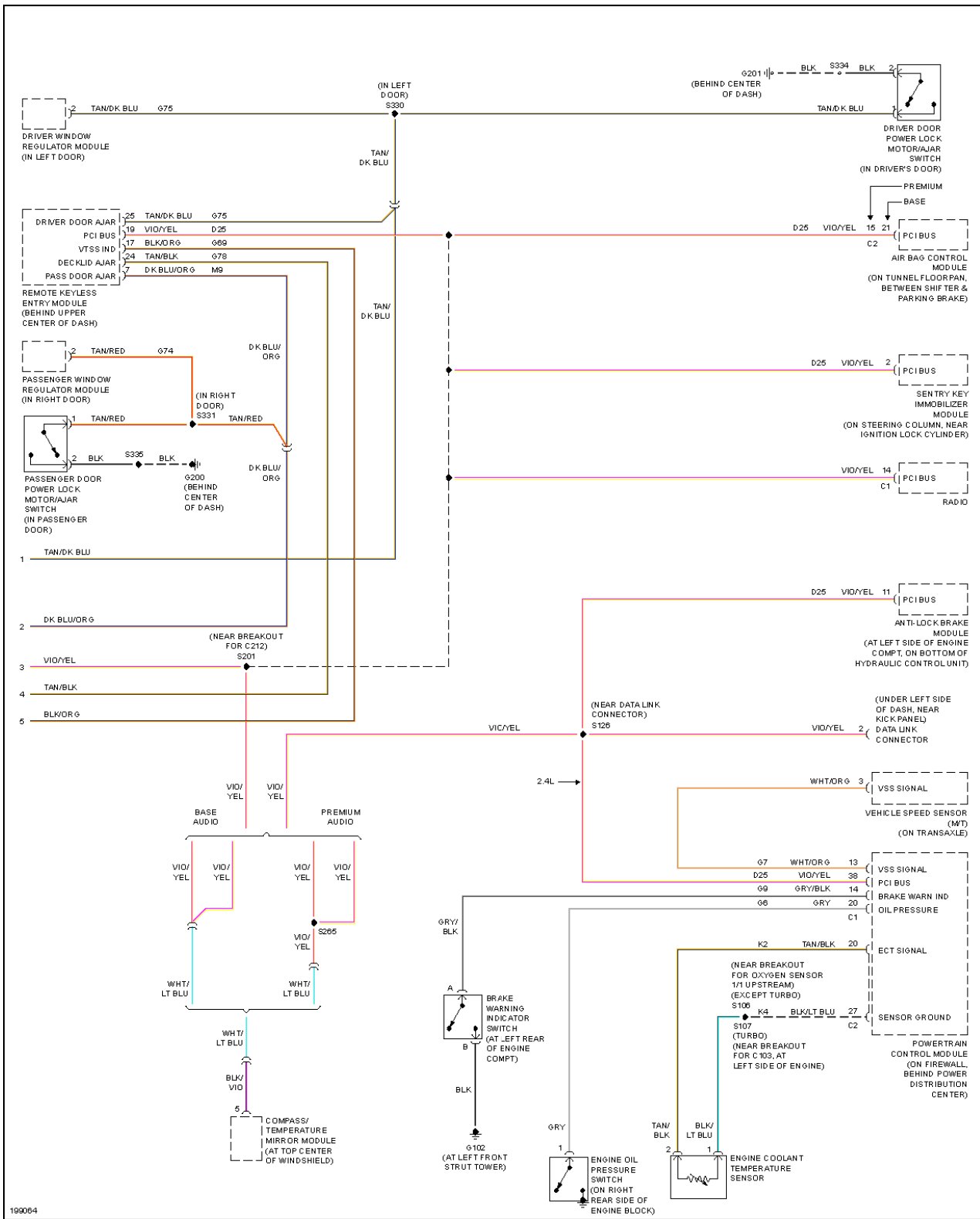
Fig. 25: Instrument Cluster Circuit, Convertible (2 of 2)
