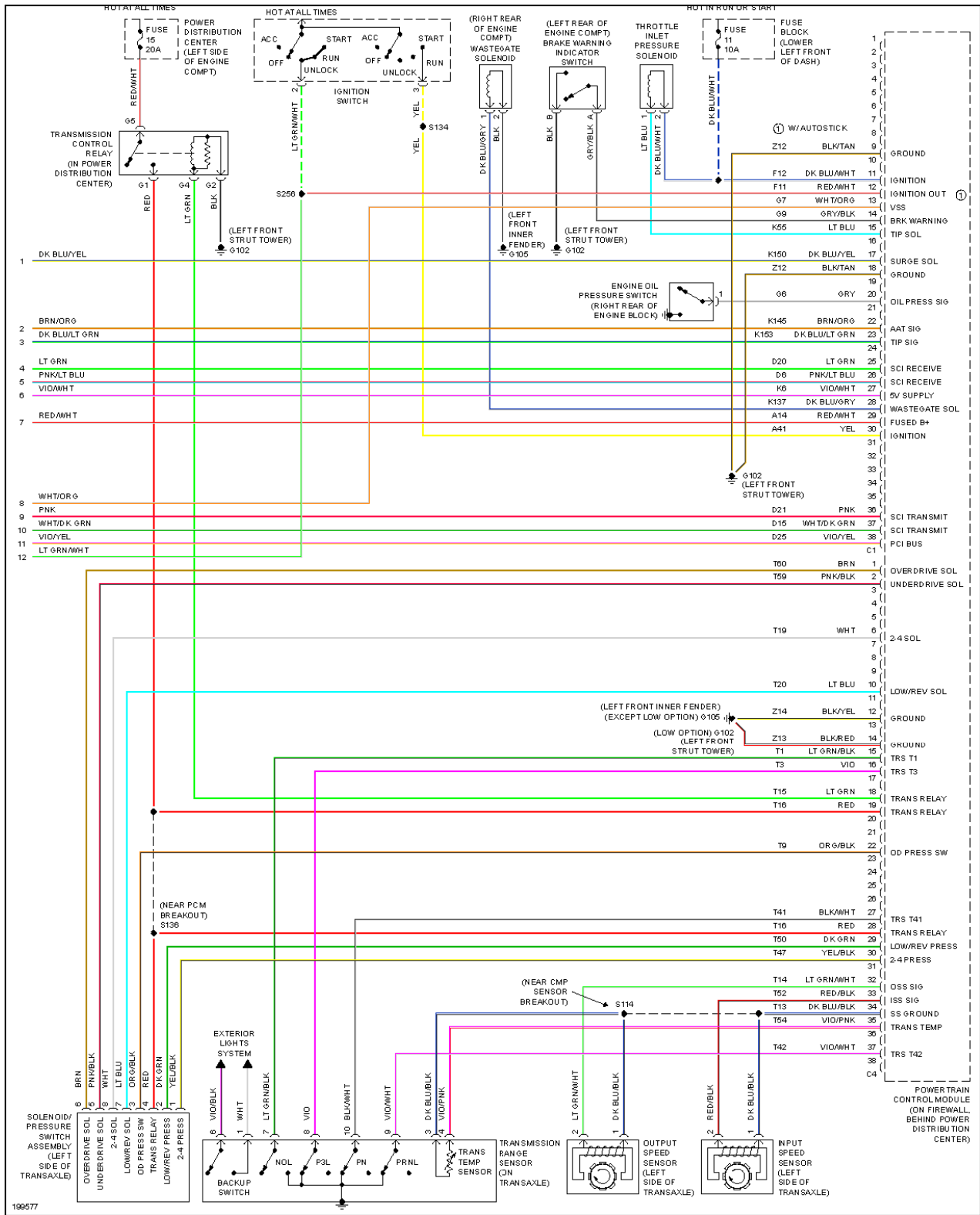
Fig. 16: 2.4L Turbo, Engine Performance Circuit (3 of 3)
