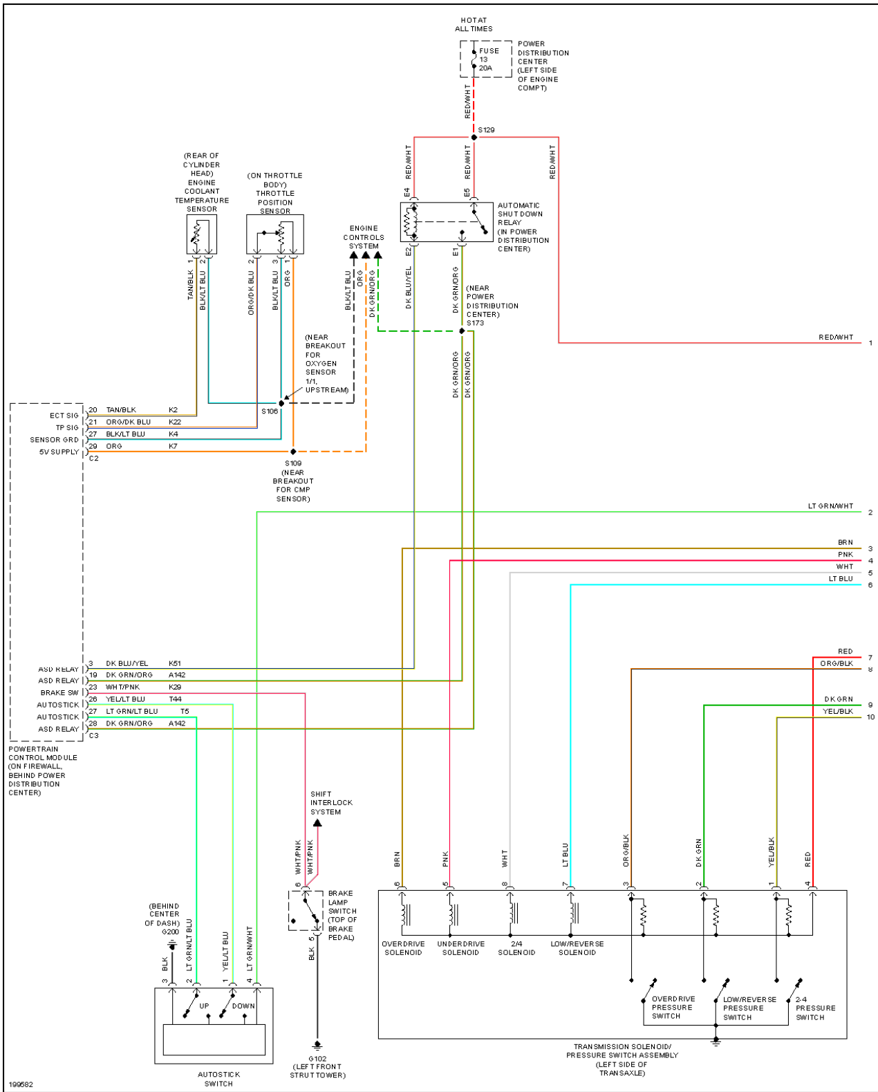
Fig. 55: 2.4L, A/T Circuit (1 of 2)
