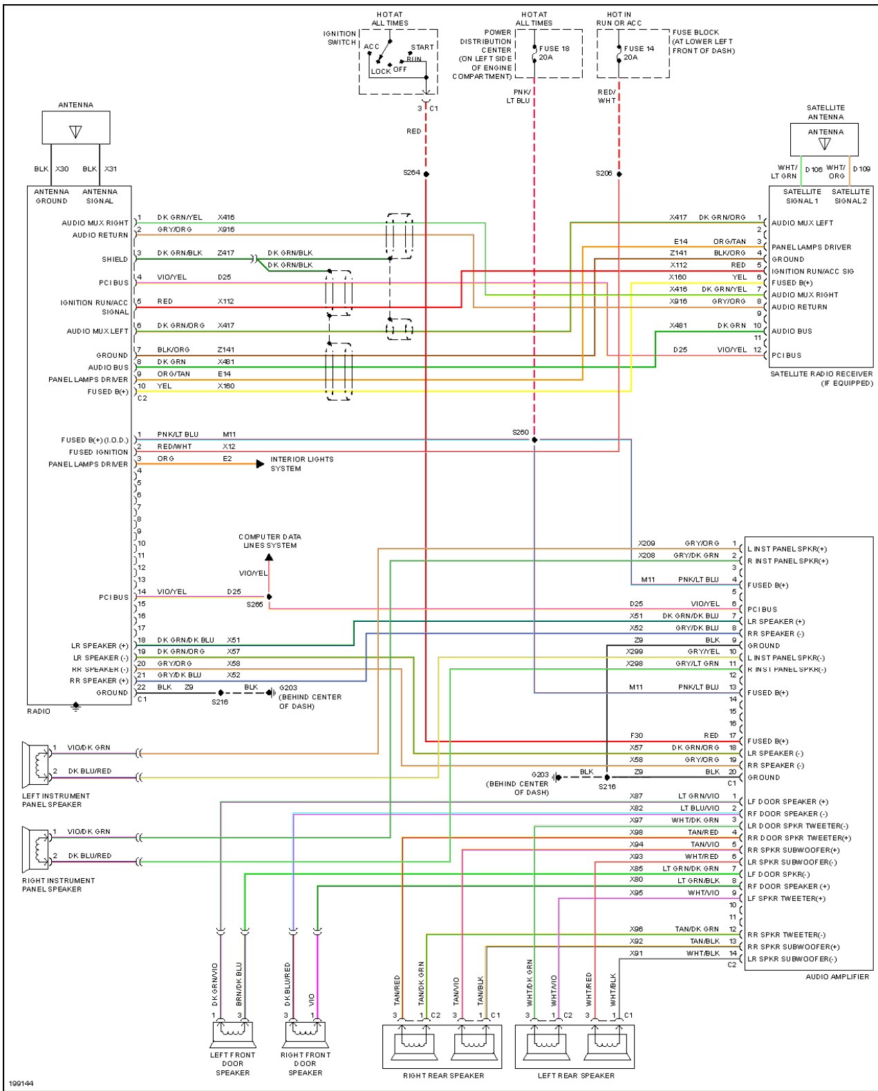
Fig. 47: Radio Circuit, Convertible Premium Radio W/O Hands Free
