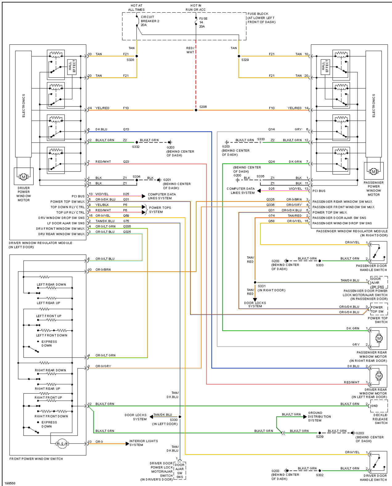
Fig. 41: Power Windows Circuit, Convertible
