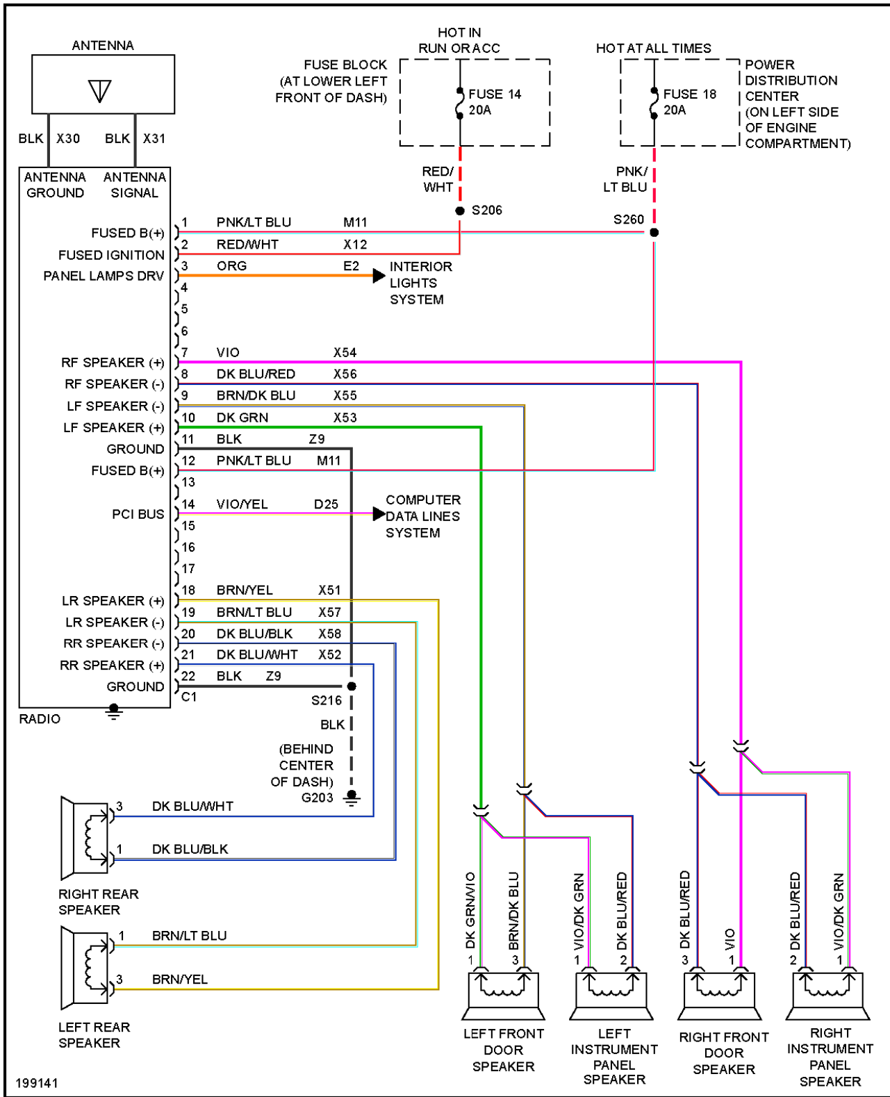
Fig. 44: Radio Circuit, Convertible Base Radio W/O Hands Free
