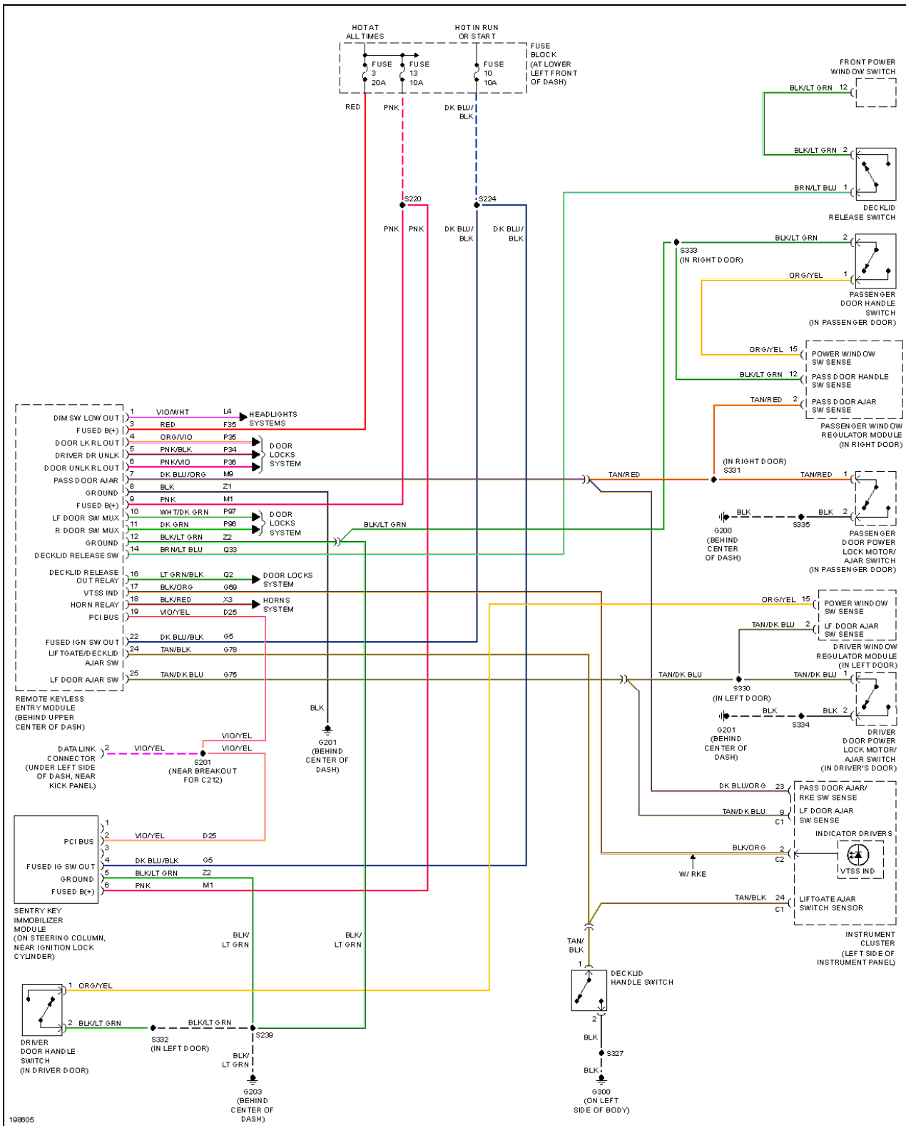
Fig. 4: Anti-theft Circuit, Convertible
