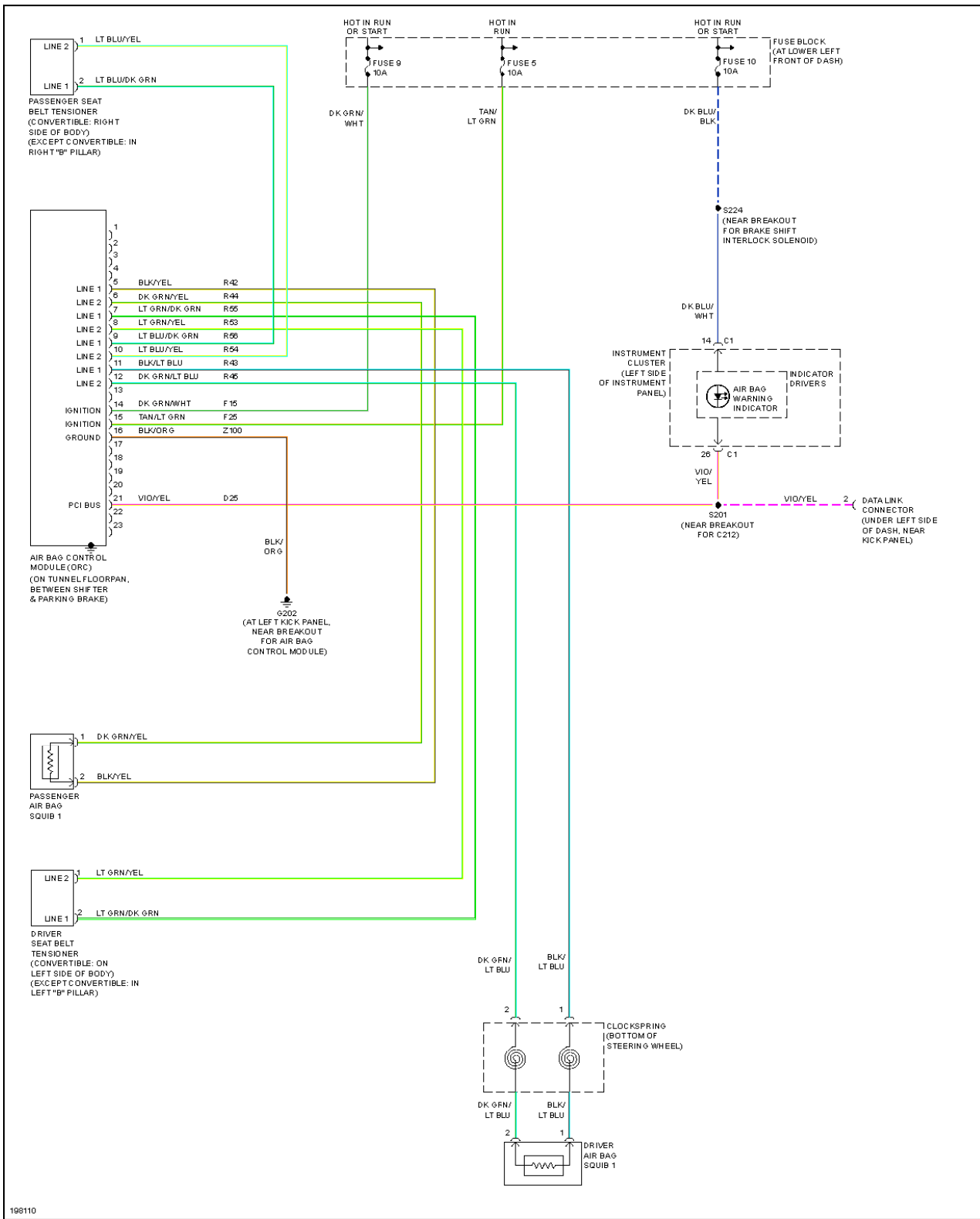
Fig. 53: Supplemental Restraints Circuit, Base
