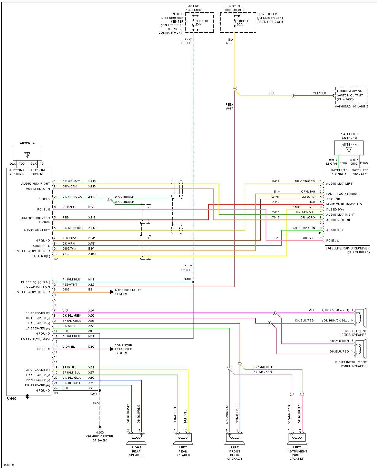
Fig. 49: Radio Circuit, Except Convertible W/O Hands Free
