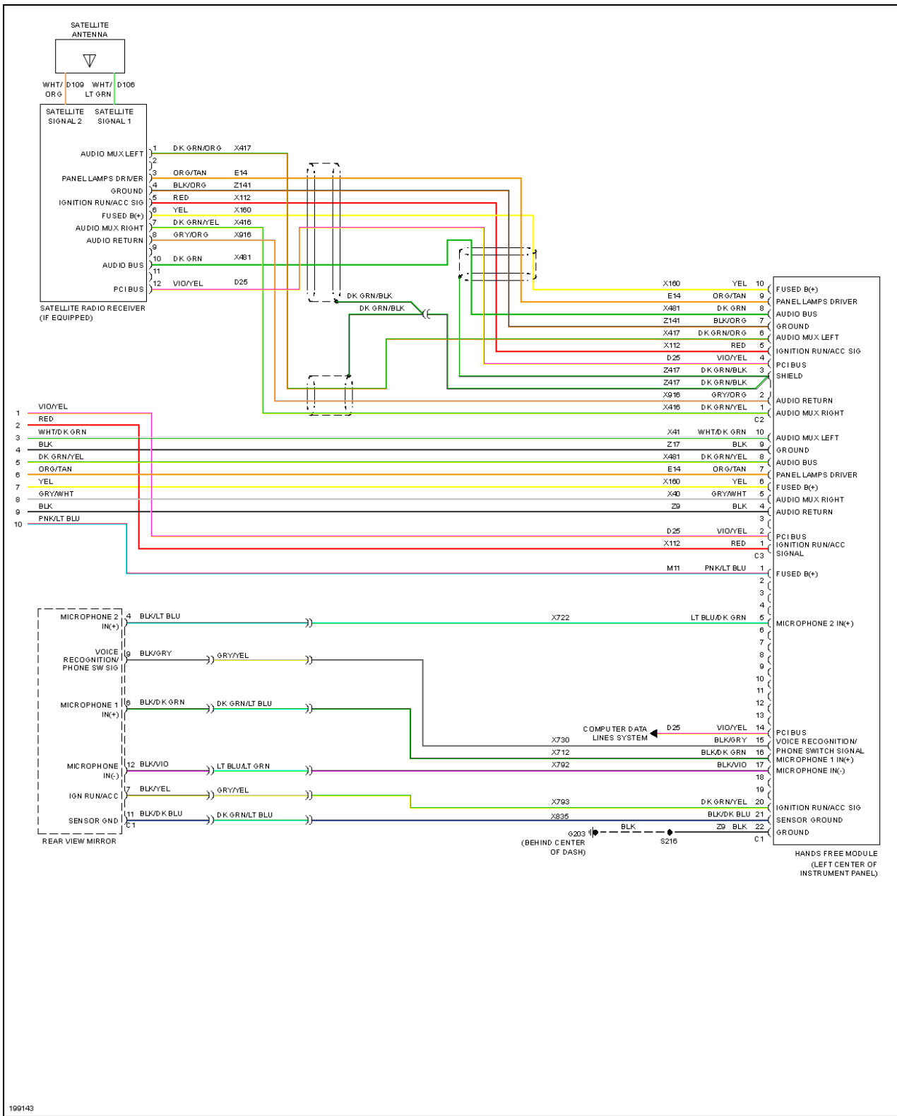
Fig. 46: Radio Circuit, Convertible Premium Radio W/ Hands Free (2 of 2)
