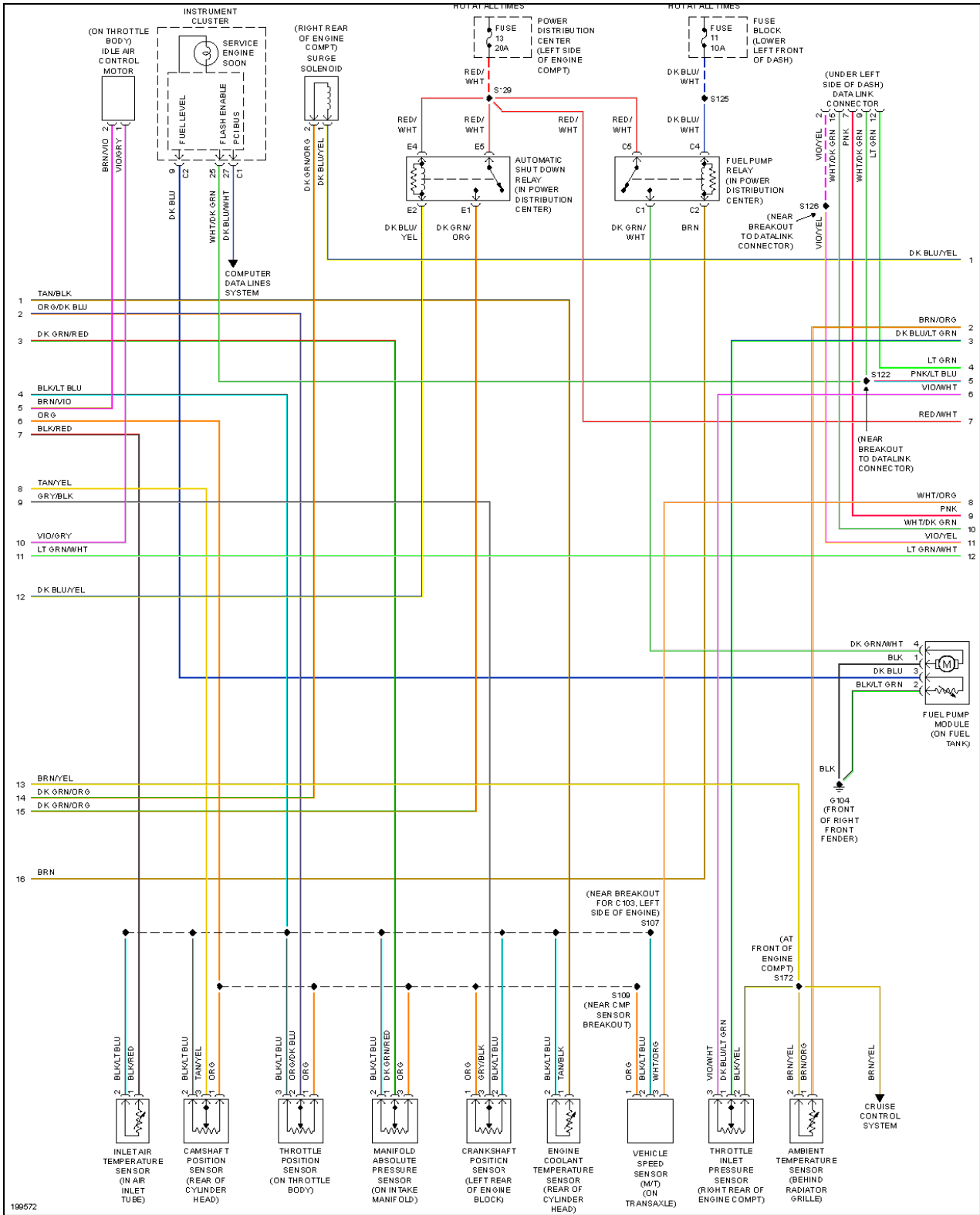
Fig. 15: 2.4L Turbo, Engine Performance Circuit (2 of 3)
