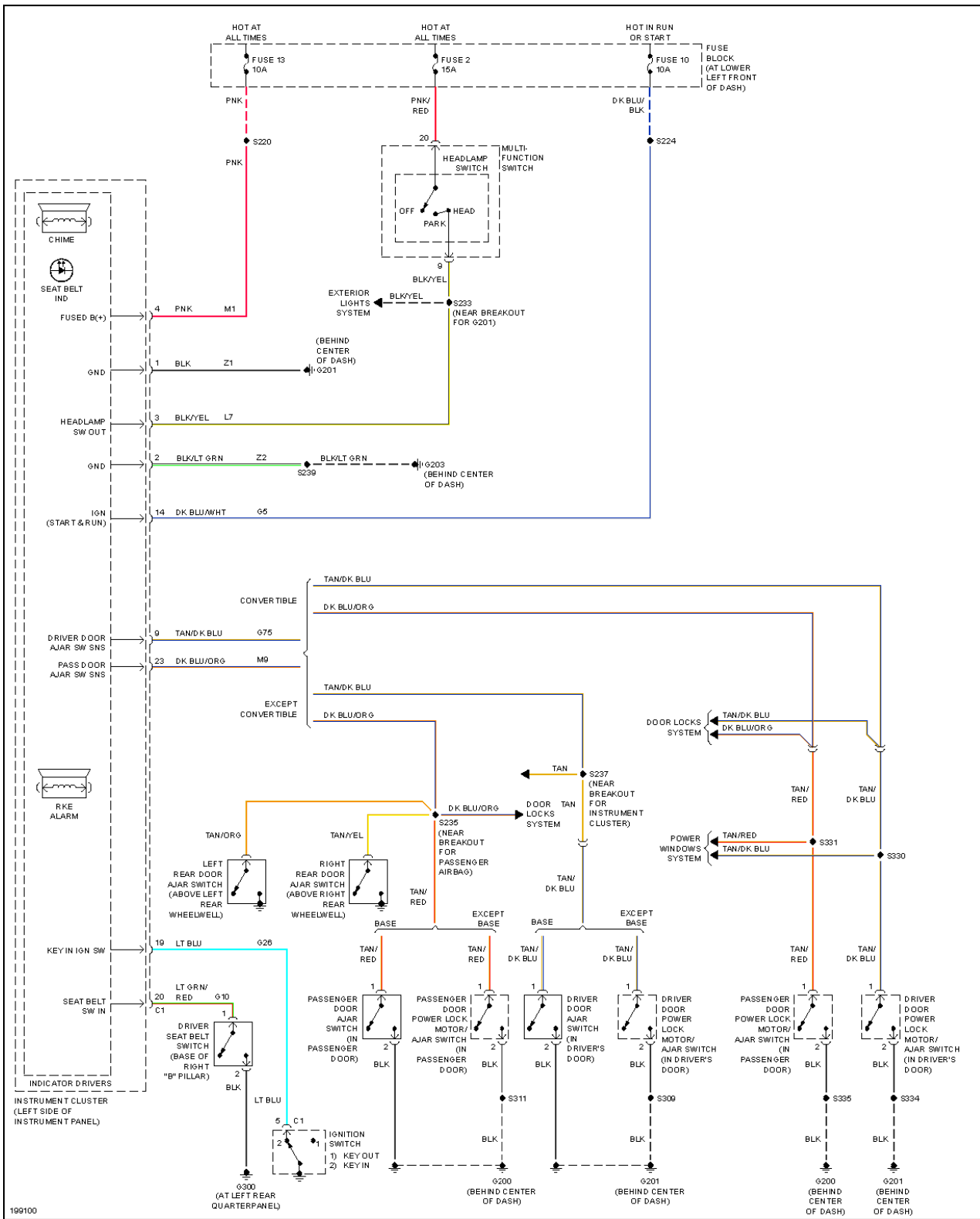
Fig. 60: Warning Systems Circuit
