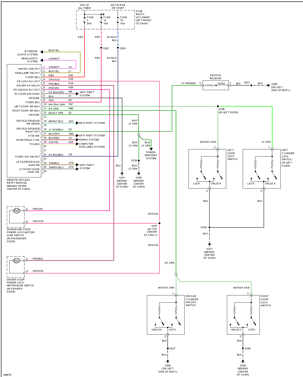
Fig. 34: Power Door Locks Circuit, Convertible
