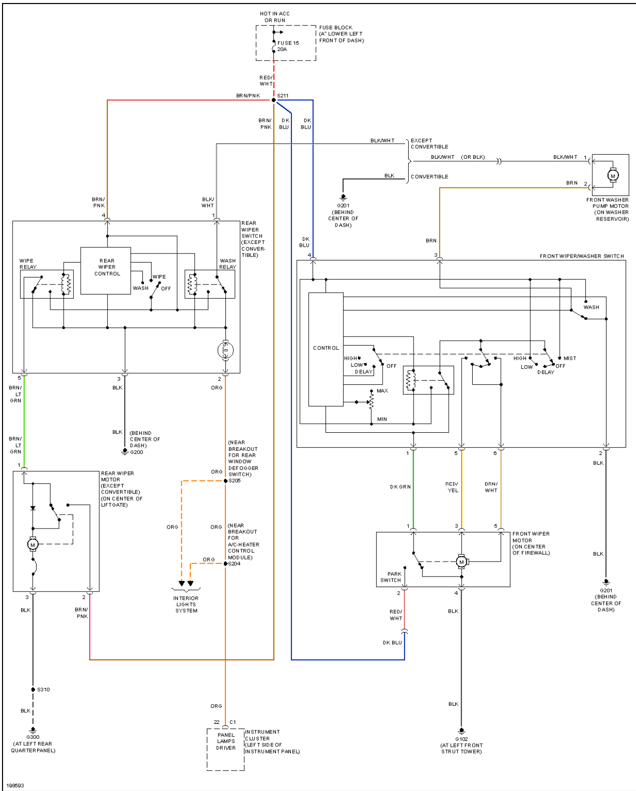
Fig. 61: Wiper/Washer Circuit
