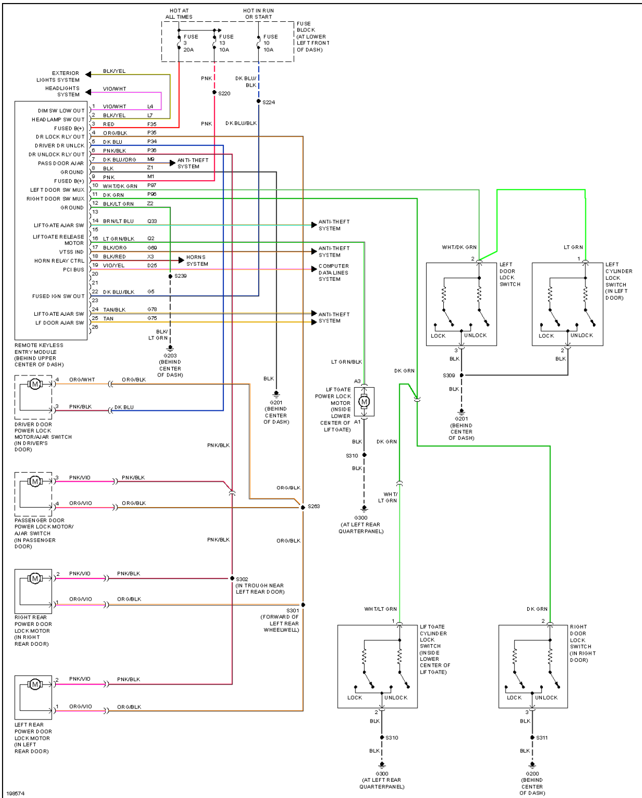
Fig. 35: Power Door Locks Circuit, Except Convertible
