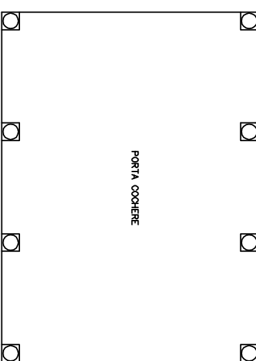
BUILDING #1 FLOOR FRAMING PLAN SCALE: 3/16" = 1'-0"
