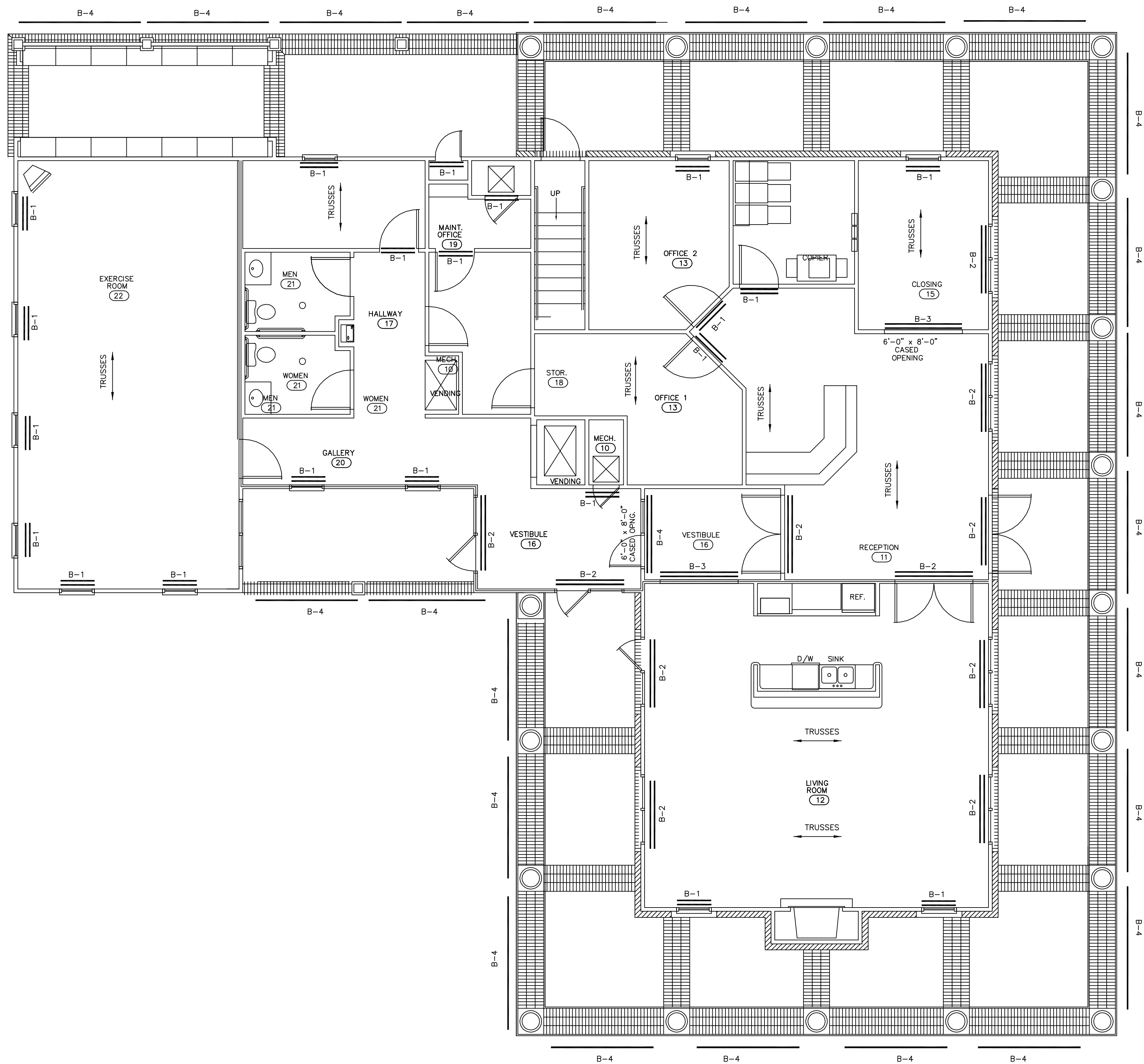
LEASING OFFICE 1 ST FLOOR FRAMING PLAN SCALE: 1/4" = 1'-0"
