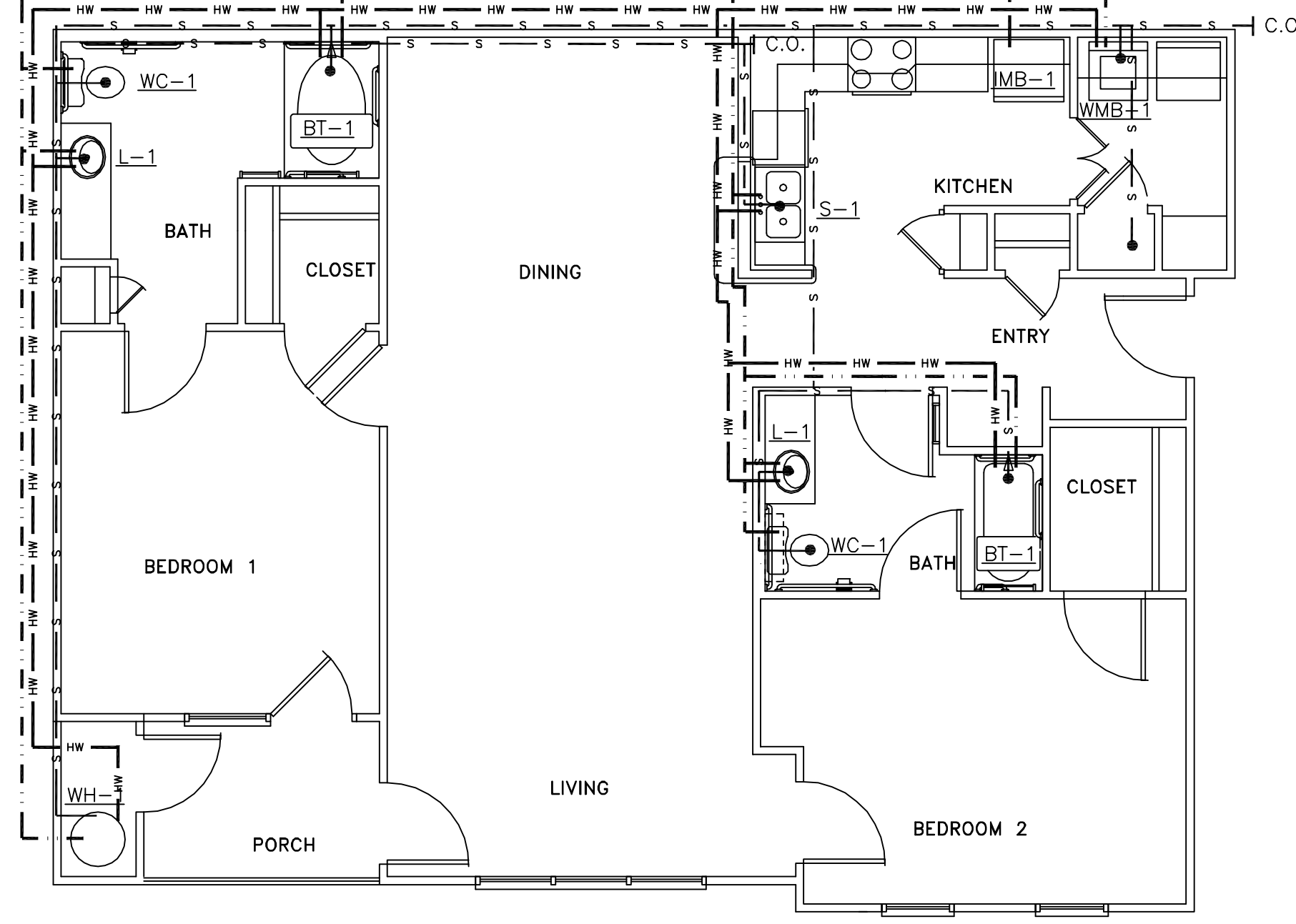
PLUMBING PLAN UNIT 2B-HC SCALE: 1/4" = 1'-0"
