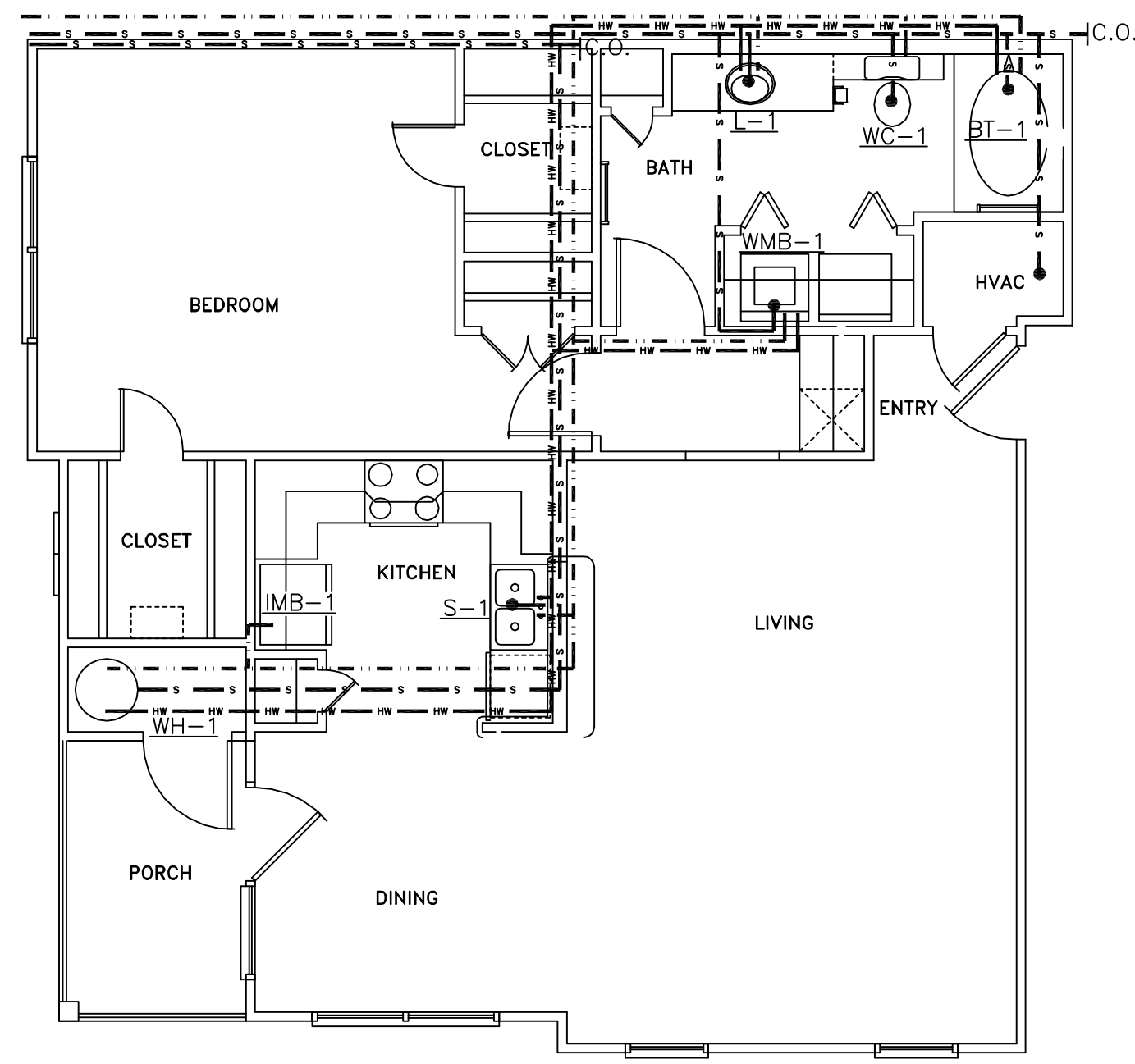
PLUMBING PLAN UNIT 1B SCALE: 1/4" = 1'-0"
