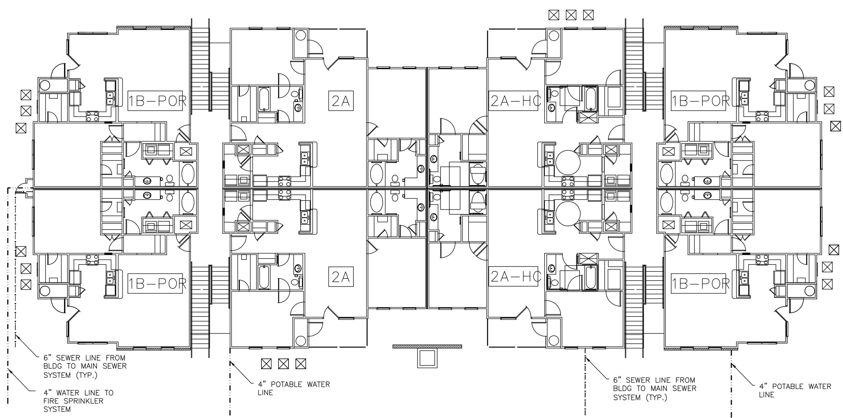
BLDG #8 FIRST FLOOR PLUMBING SCALE: 1/8" = 1'-0"
