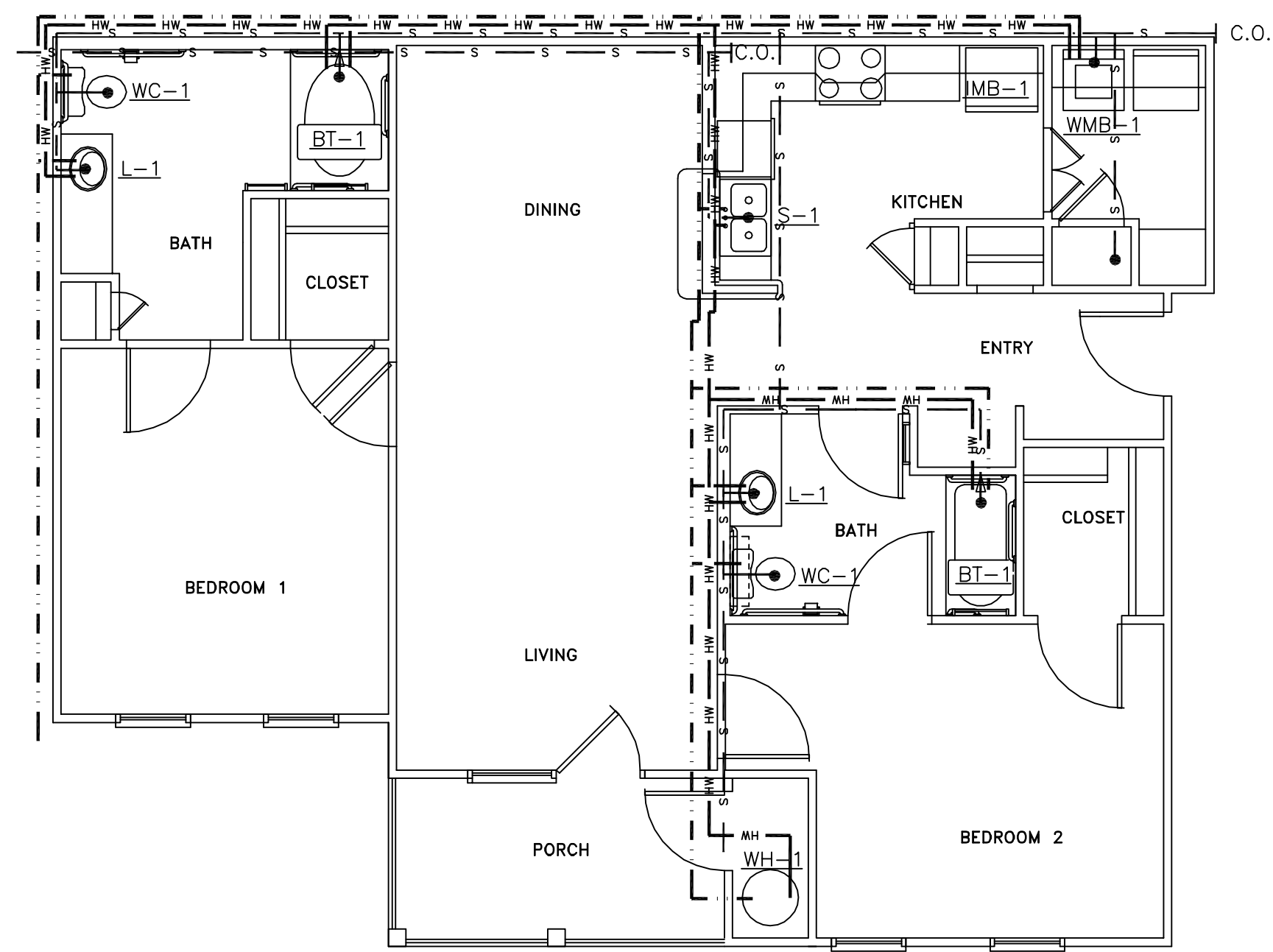
PLUMBING PLAN UNIT 2A-HC SCALE: 1/4" = 1'-0"
