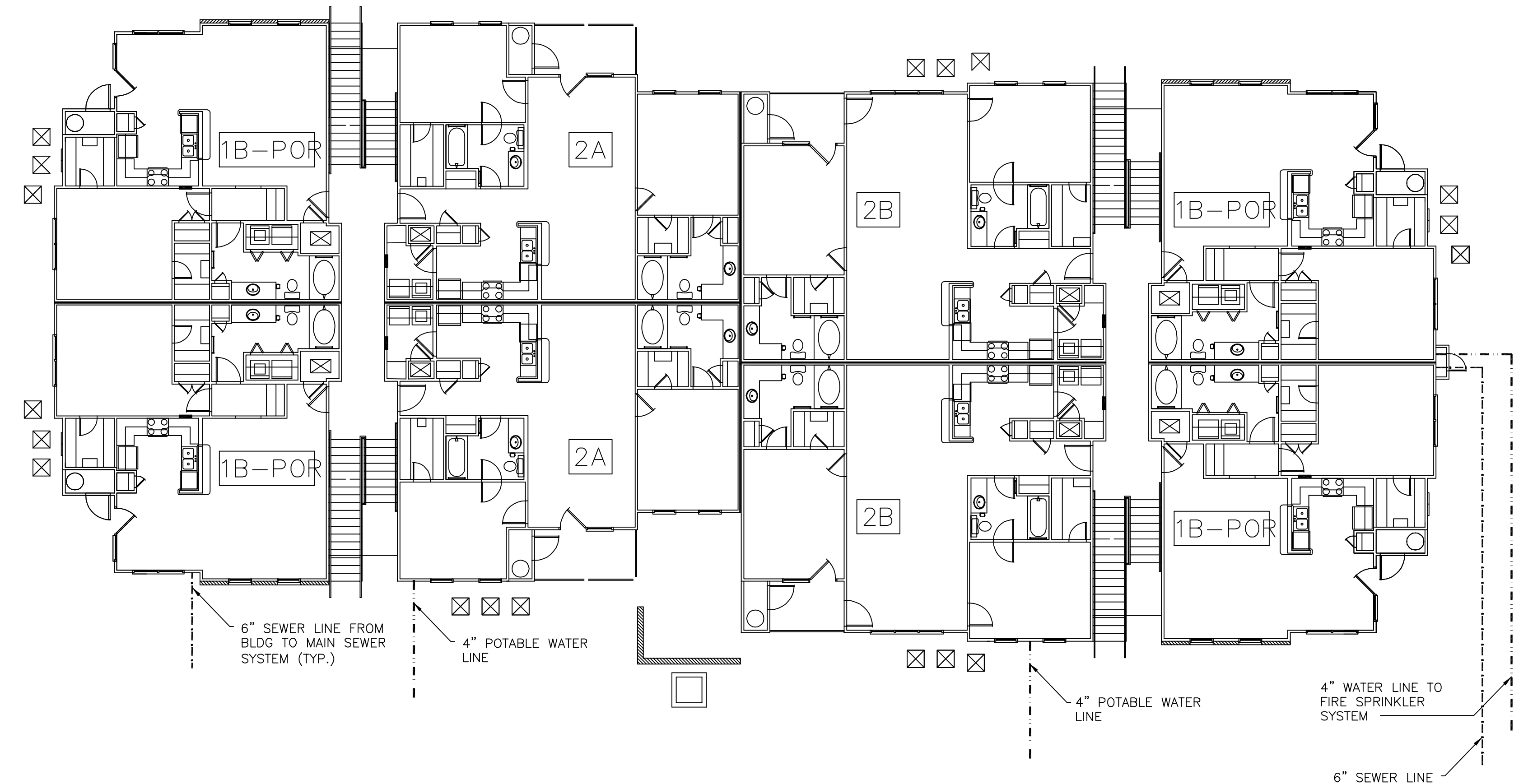
BLDG #9 FIRST FLOOR PLUMBING SCALE: 1/8" = 1'-0"
