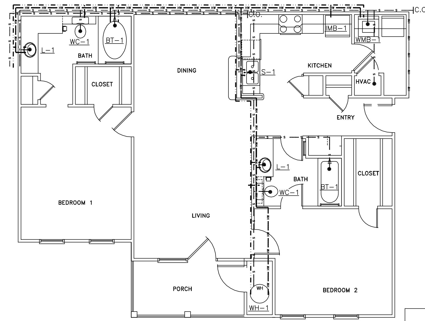
PLUMBING PLAN UNIT 2A SCALE: 1/4" = 1'-0"
