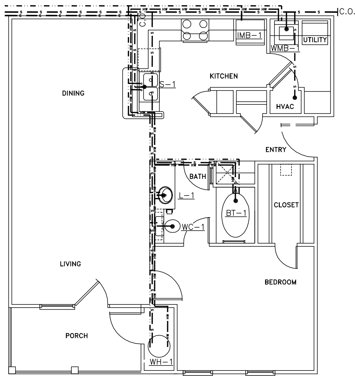
PLUMBING PLAN UNIT 1A SCALE: 1/4" = 1'-0"
