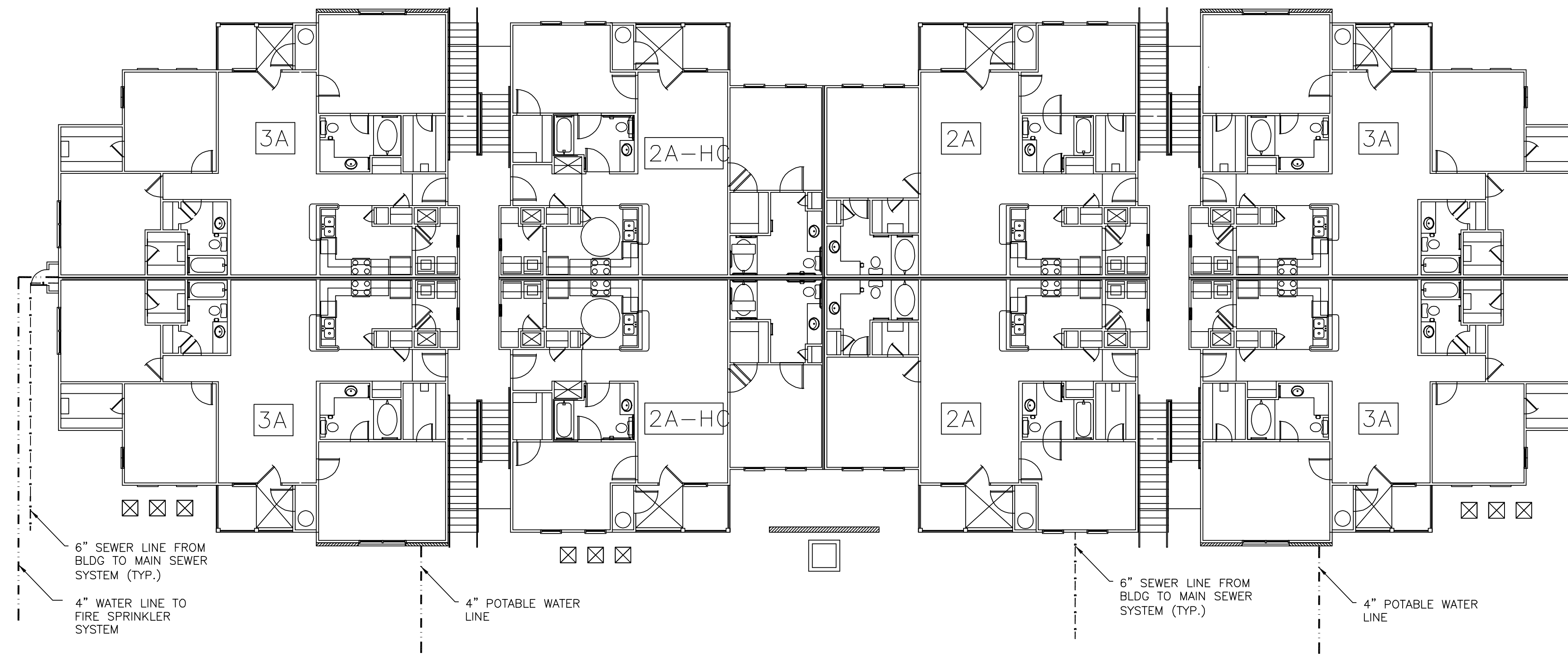
BLDG #4 & #10 FIRST FLOOR PLUMBING SCALE: 1/8" = 1'-0"
