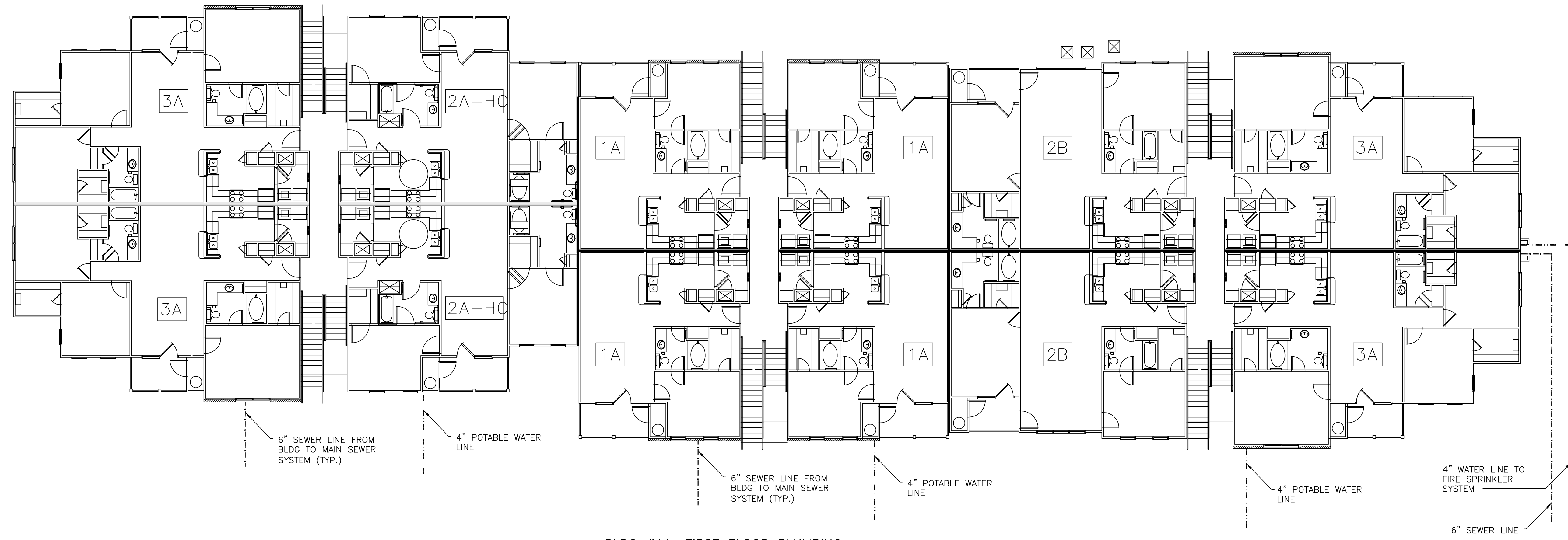
BLDG #11, FIRST FLOOR PLUMBING SCALE: 1/8" = 1'-0"
