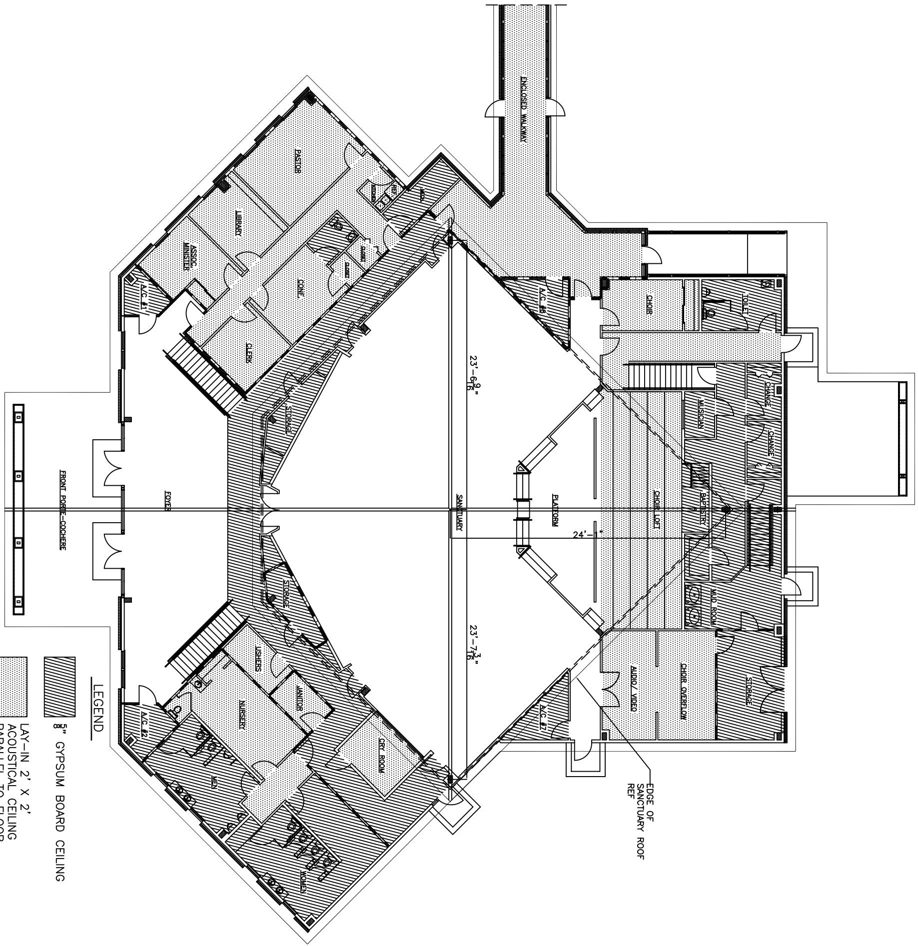
REFLECTIVE CEILING PLAN SCALE: 1/8" = 1'-0"
