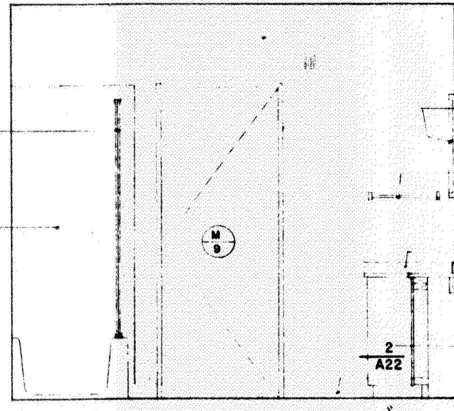
north elev. - bath "1" rectory
