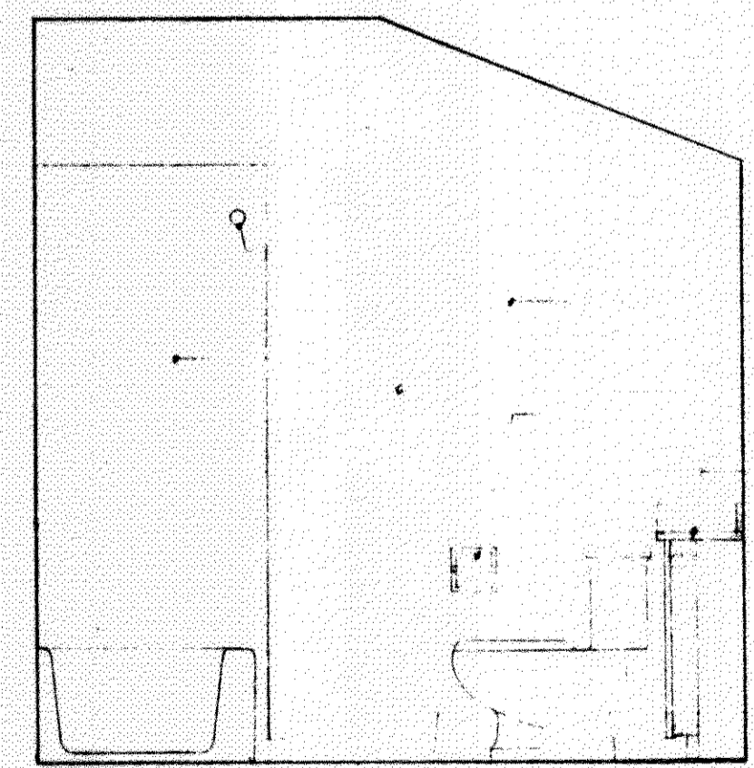
north elev. bath "2" north elev.-bath "3"-opposite hand rectory
