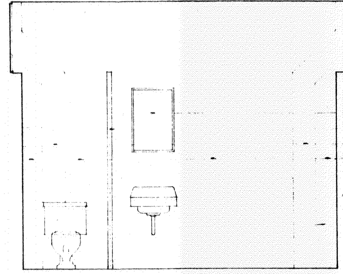
west elev. -toilet "2" (sanctuary) east elev. -toilet "1" (sanctuary) same but opp. hand
