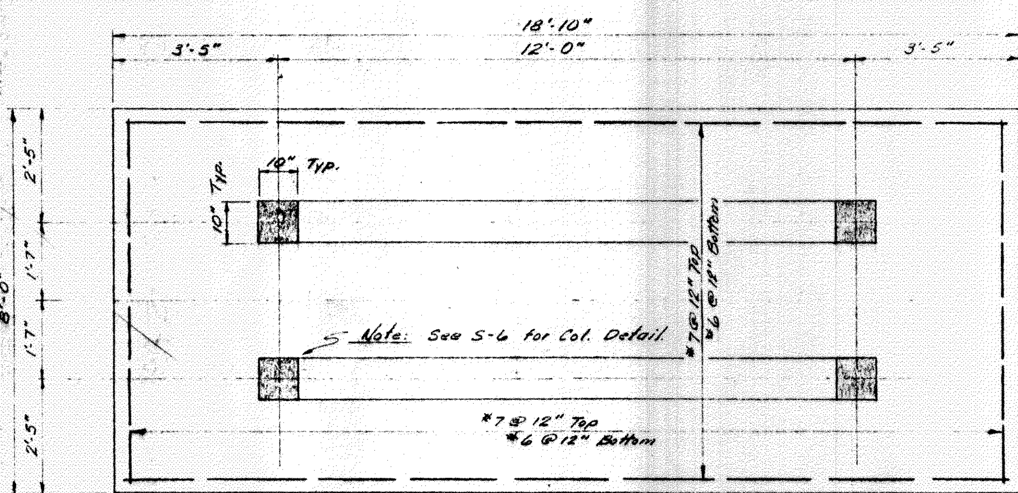
TYPICAL COLUMN FOOTING TYPE 'B'
