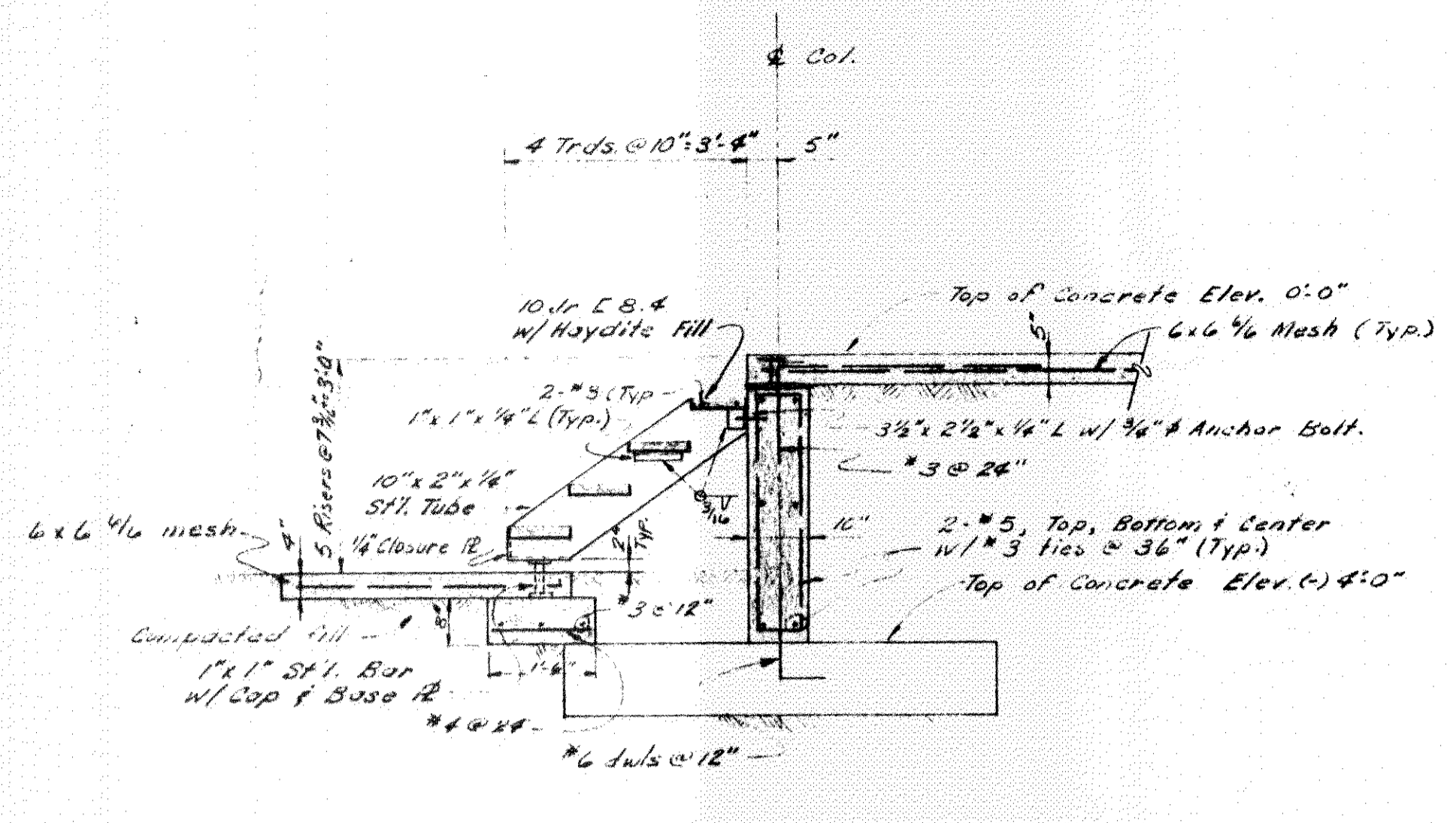
SECTION 3-3
