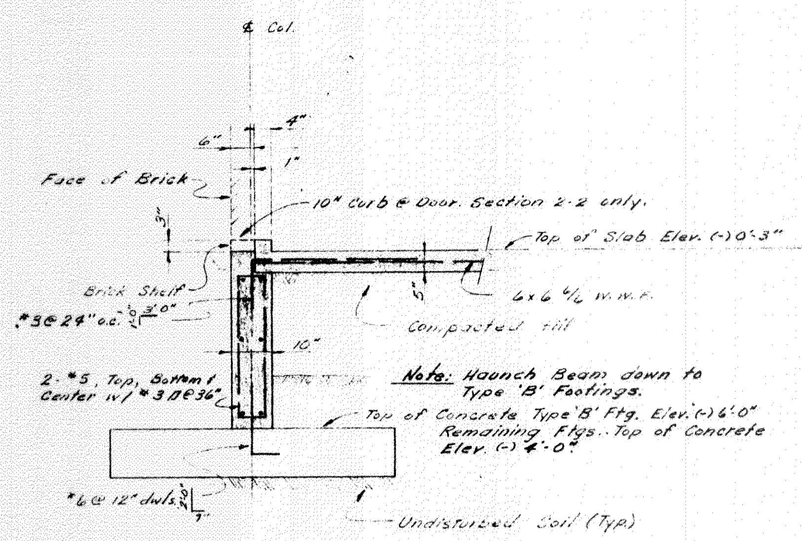
SECTION 1-1 SECTION 2-2 as noted
