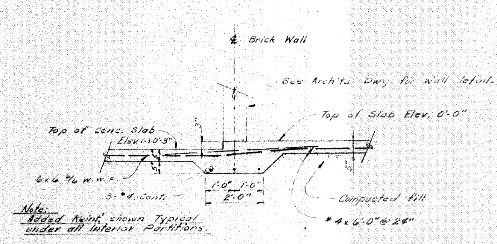
SECTION 5-5
