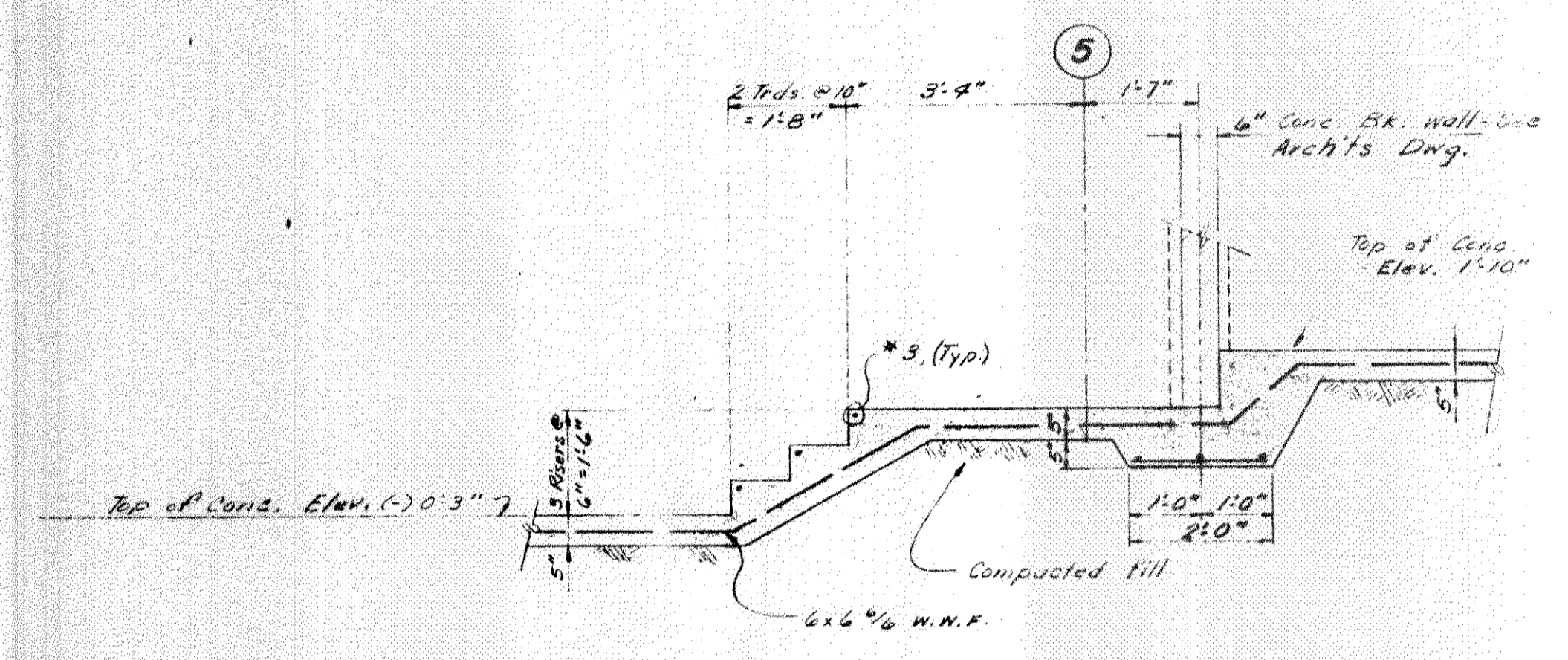
SECTION 7-7
