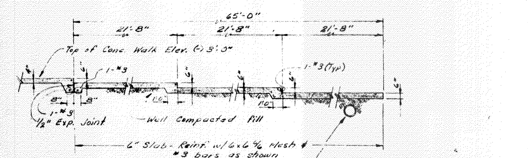
SECTION 10-10
