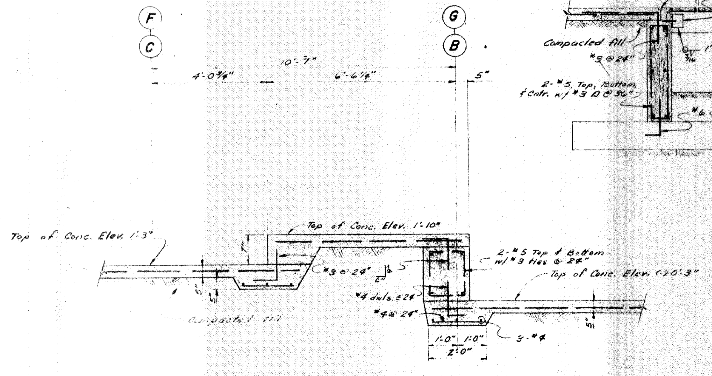
SECTION 9-9
