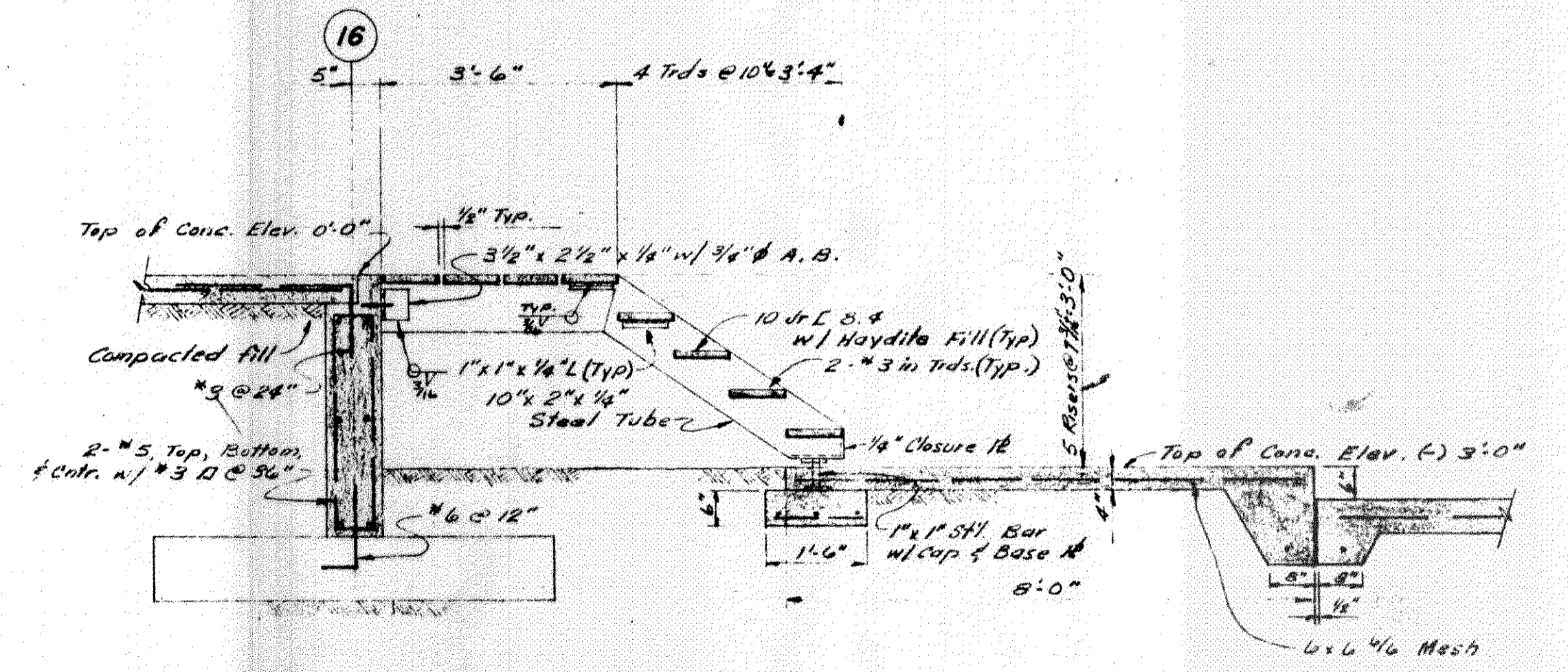
SECTION 4-4
