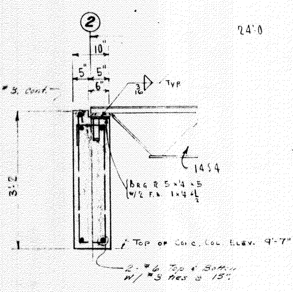
SECTION 1-1
