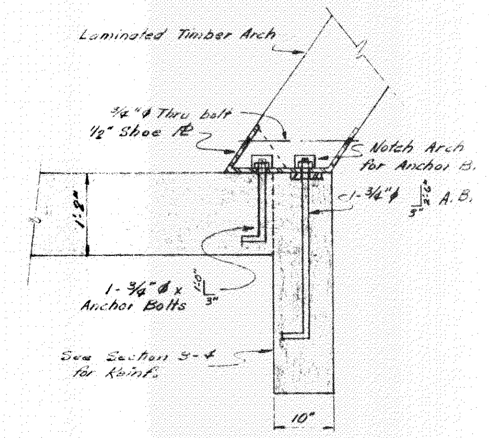
SECTION
