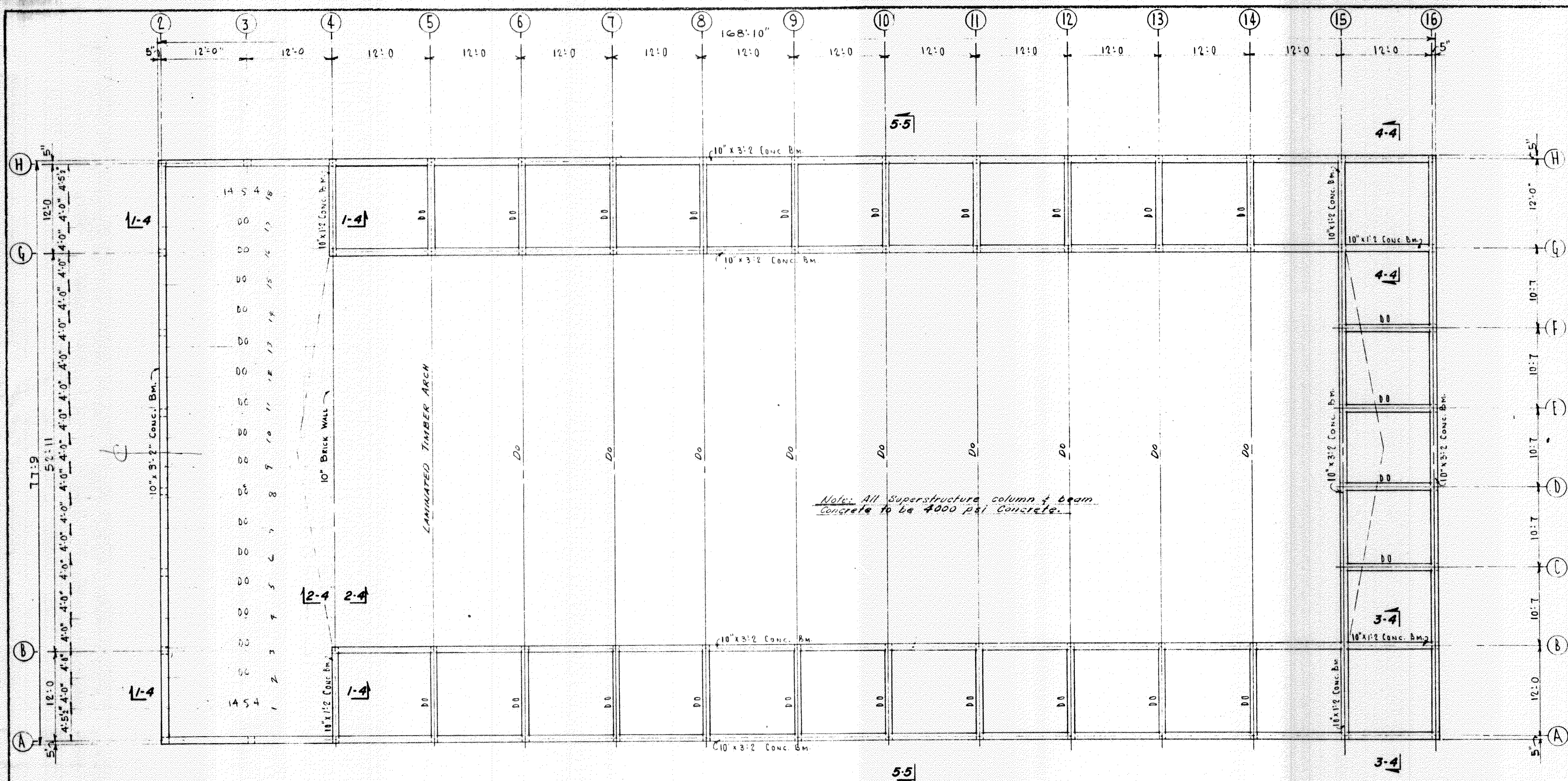
ROOF FRAMING PLAN
