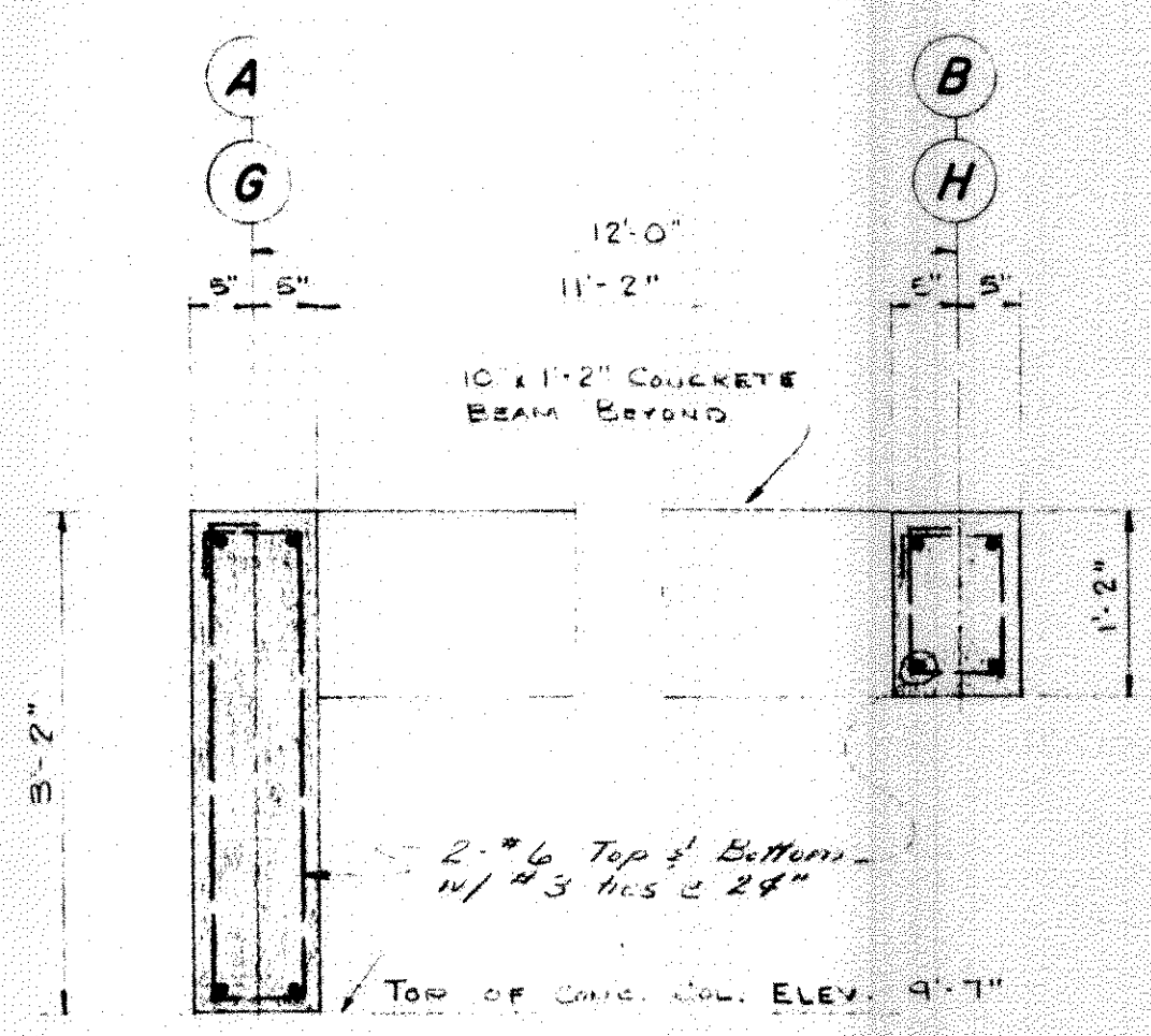
SECTION 3-3
