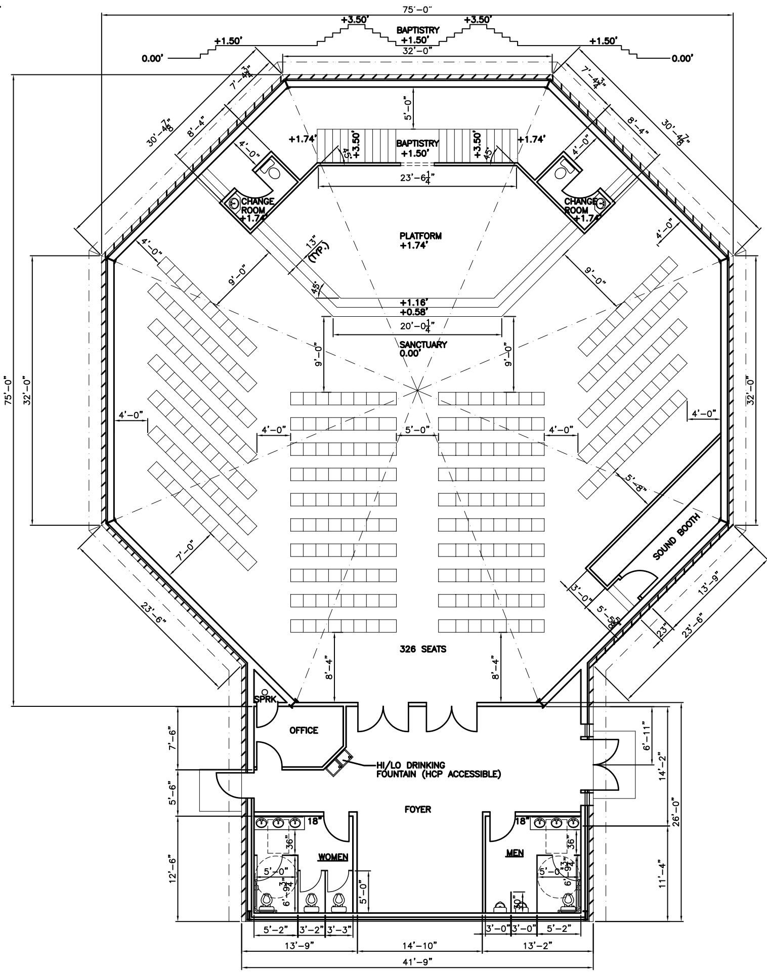
FLOOR PLAN SCALE: 3/16" = 1'-0"
