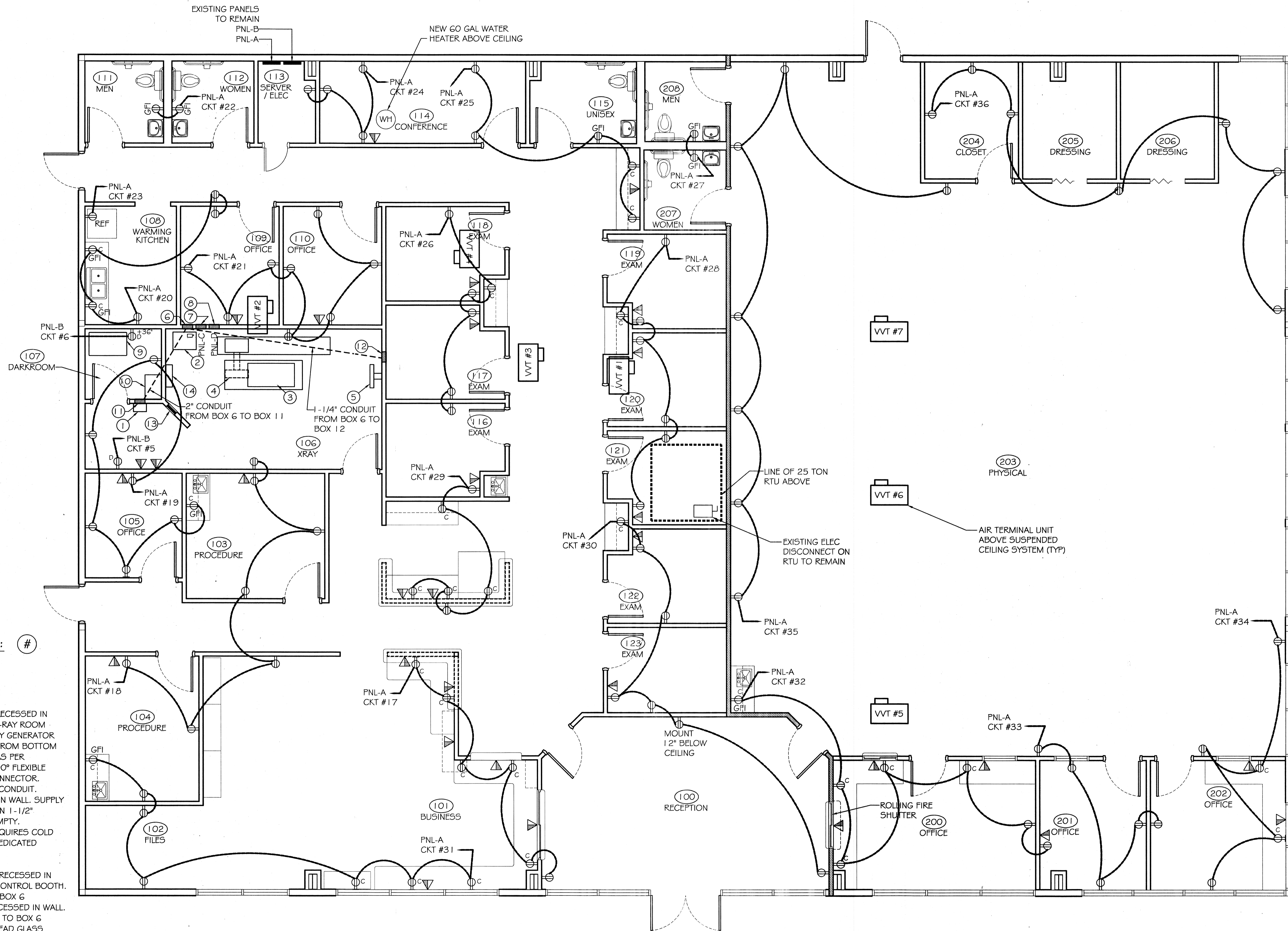
POWER PLAN SCALE: 1/4"=1'-0"
