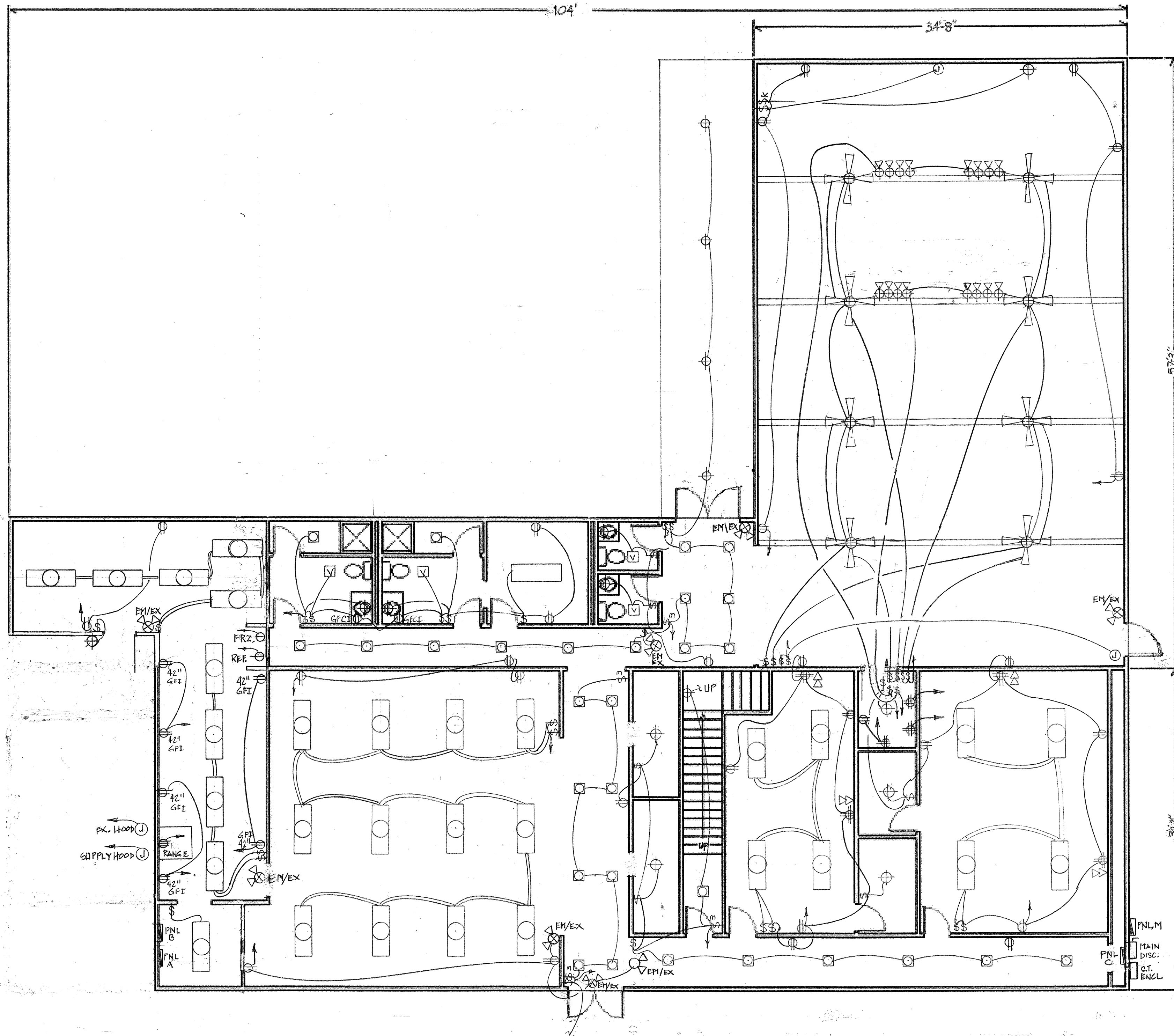
TRINITY LUTHERAN CHURCH - 1ST FLOOR ELECTRICAL PLAN : NO SCALE
