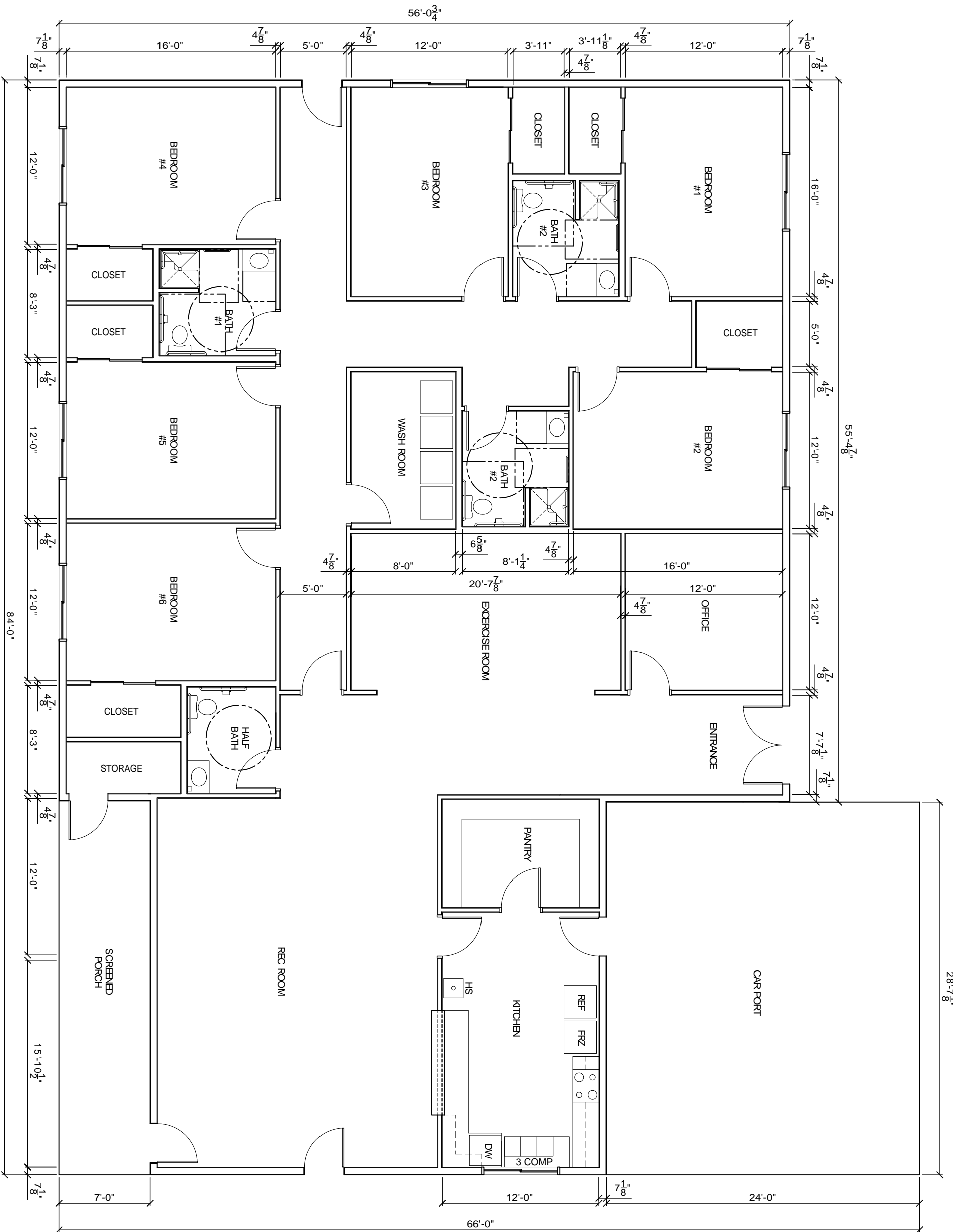
PRELIM. FLOOR PLAN #1 SCALE: 1/4" = 1'
