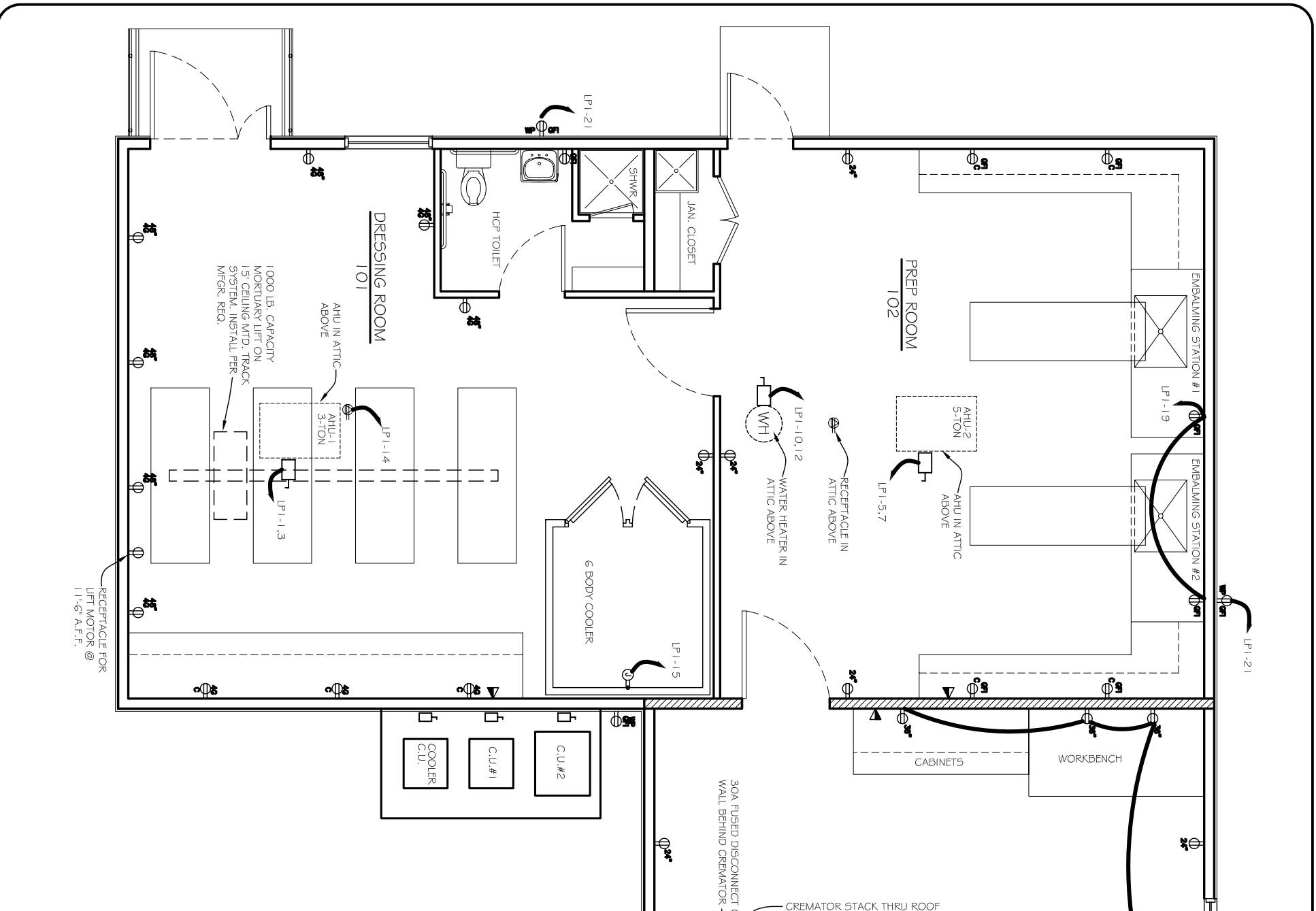
ELECTRICAL POWER PLAN SCALE: 3/8" = 1'-0"
