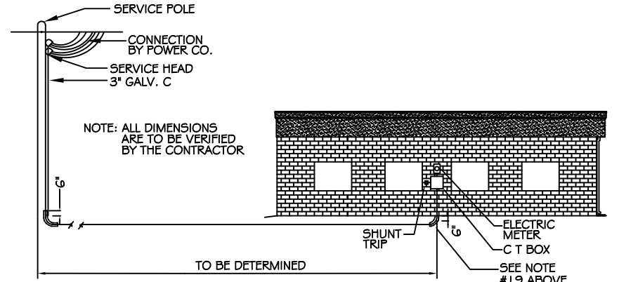
ELECTRICAL SERVICE DETAIL N.T.S. 208V 3 PHASE
