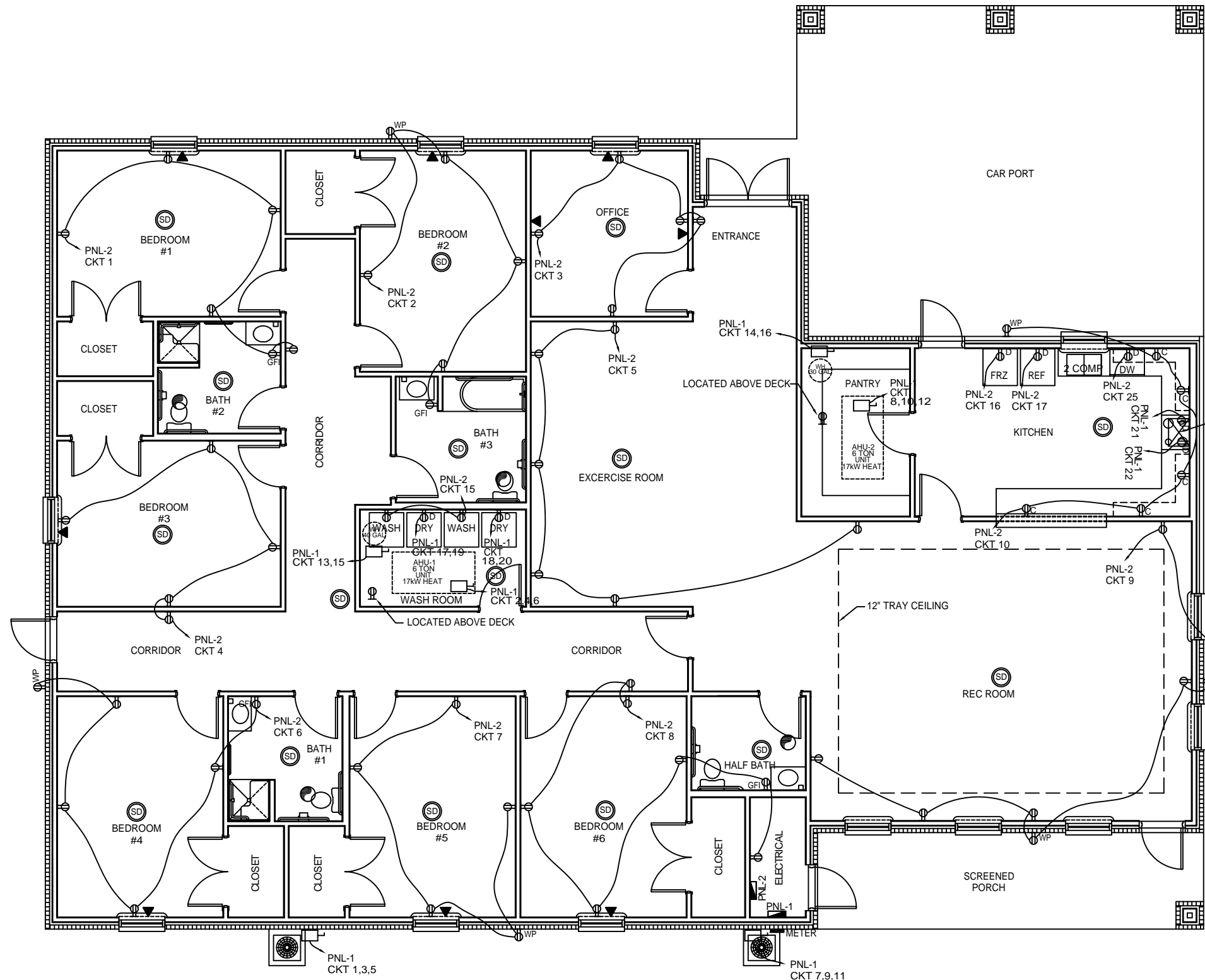
POWER PLAN SCALE: 1/4"=1'
