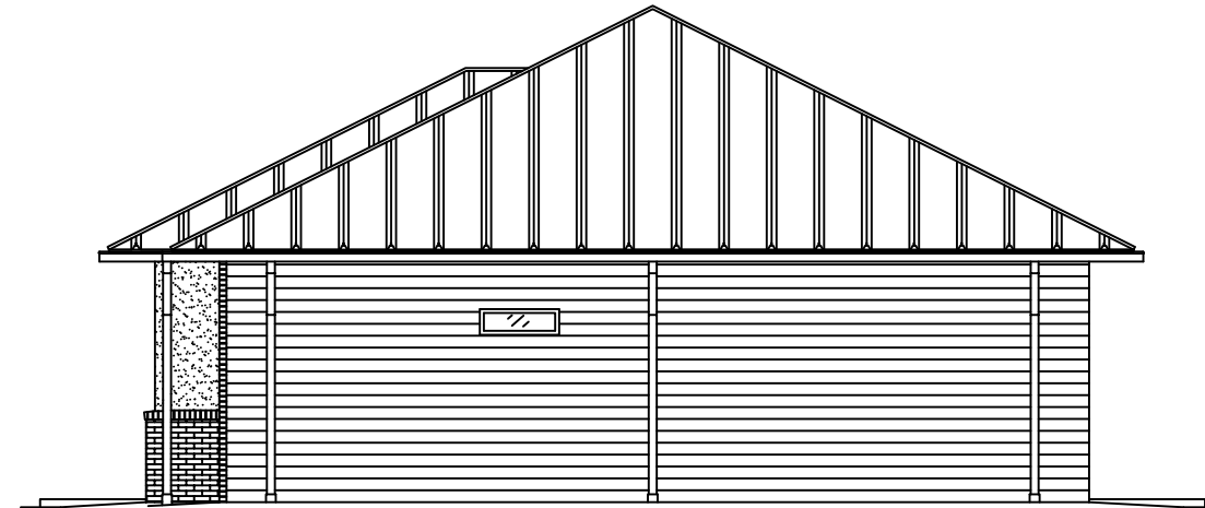
RIGHT SIDE ELEVATION SCALE: 1/4"=1'
