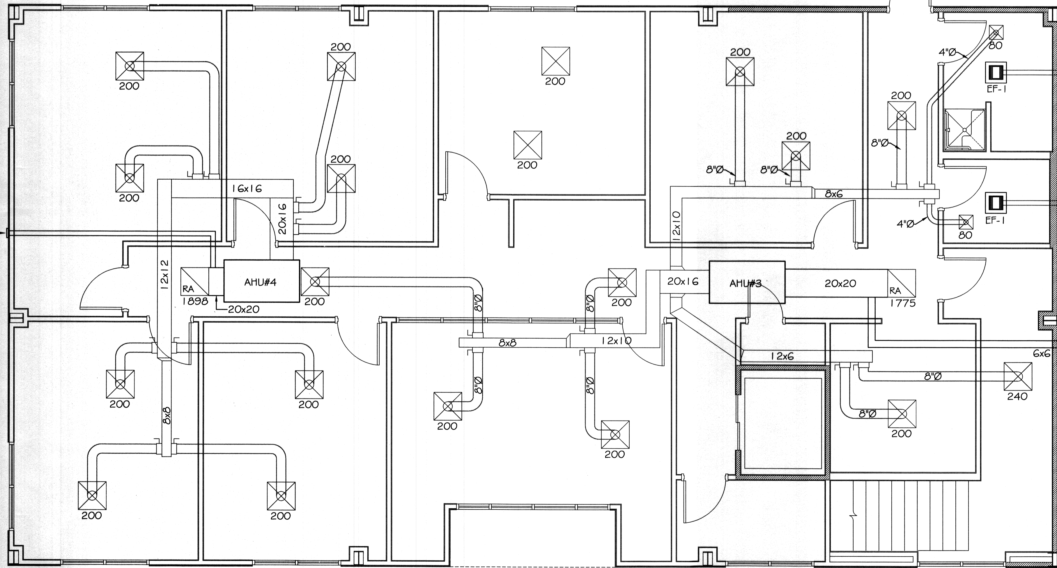
2ND FLOOR MECH. PLAN SCALE: 1/4" = 1'-0"
