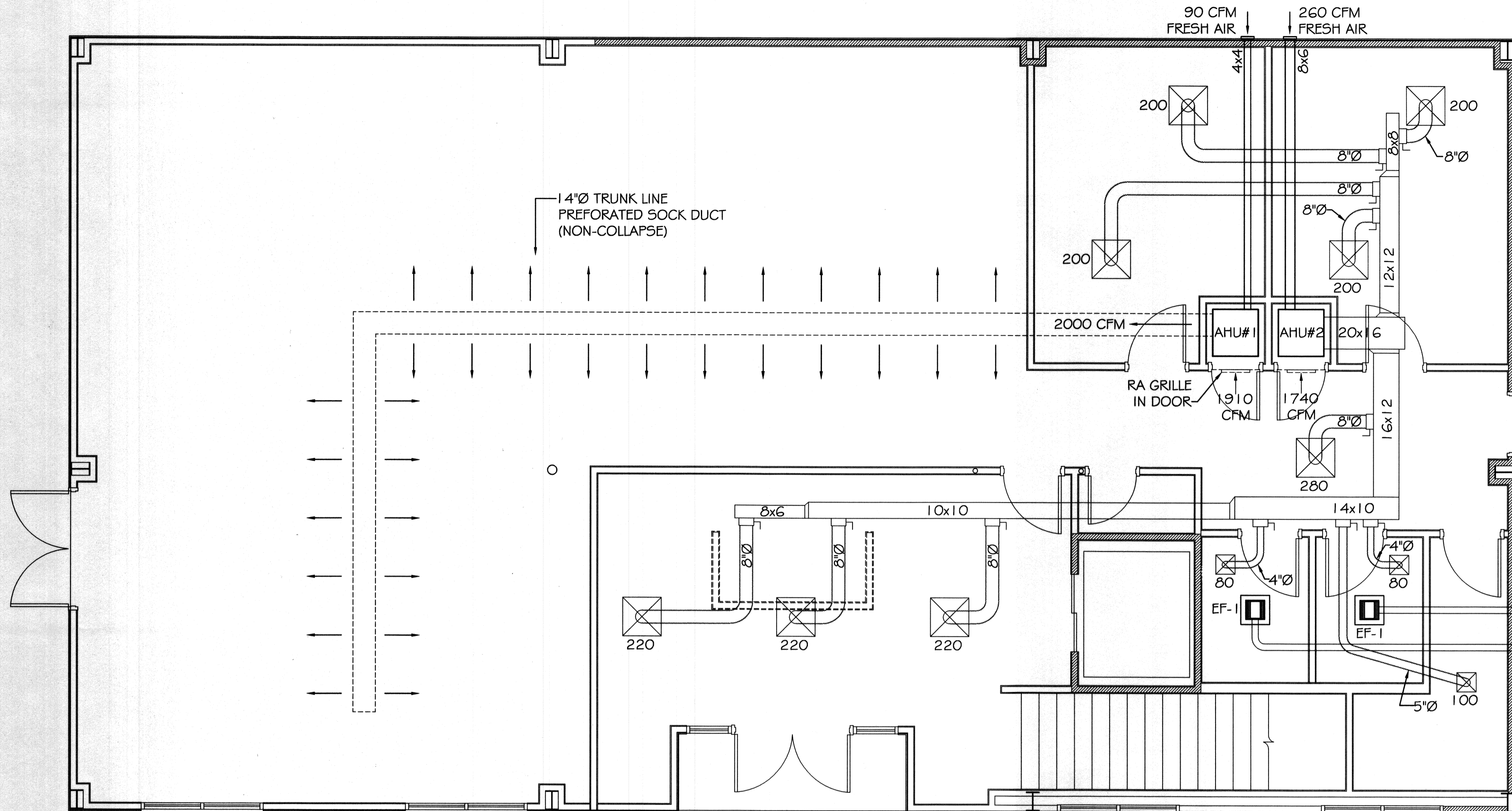
1ST FLOOR MECH. PLAN SCALE: 1/4" = 1'-0"
