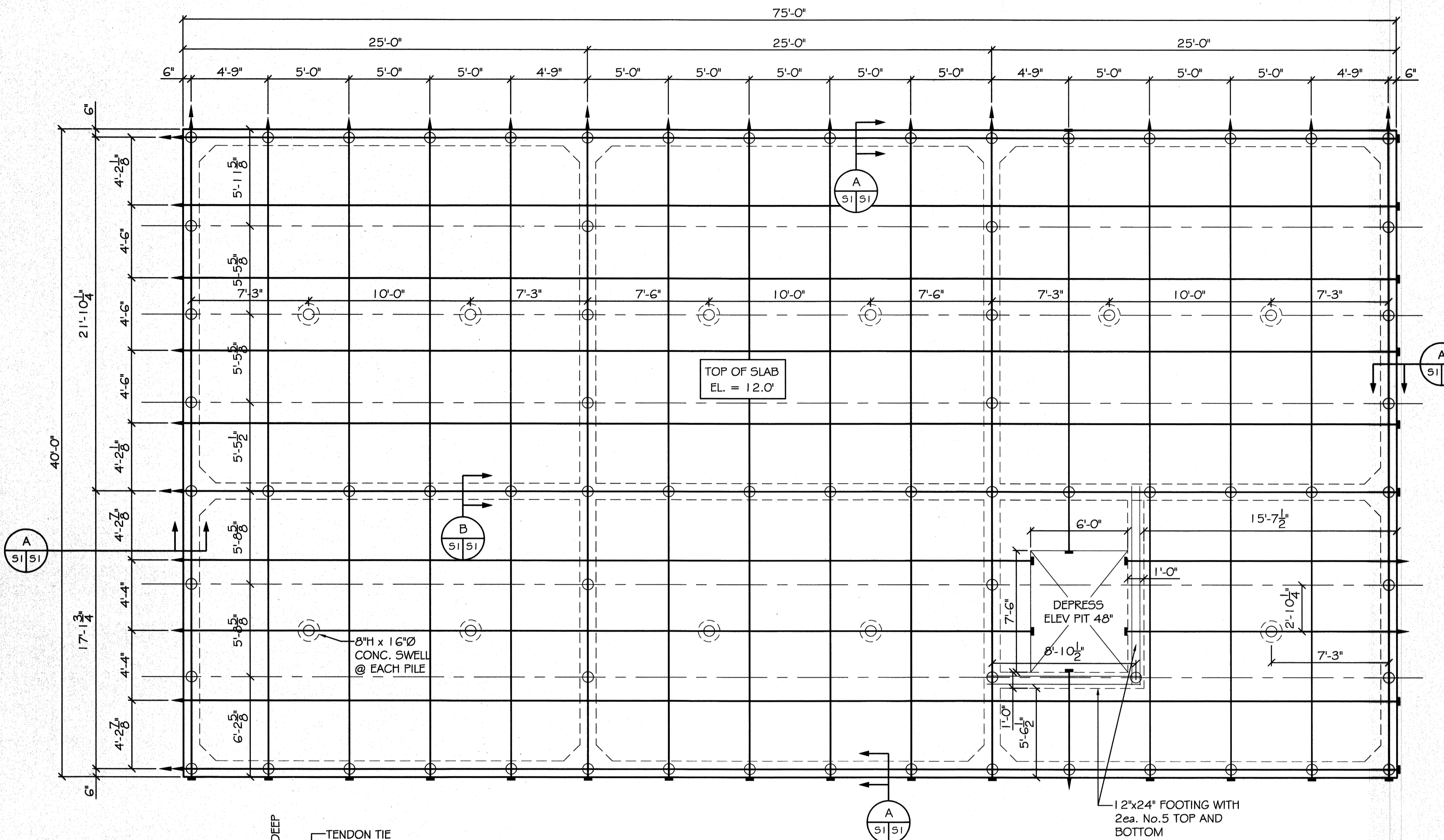
FOUNDATION AND PILING PLAN SCALE: 1/4" = 1'-0"
