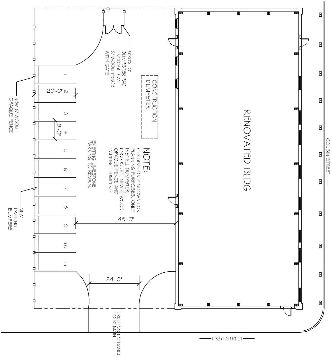
PARKING & DUMPSTER PLAN SCALE: 3/32"=1'-0"
