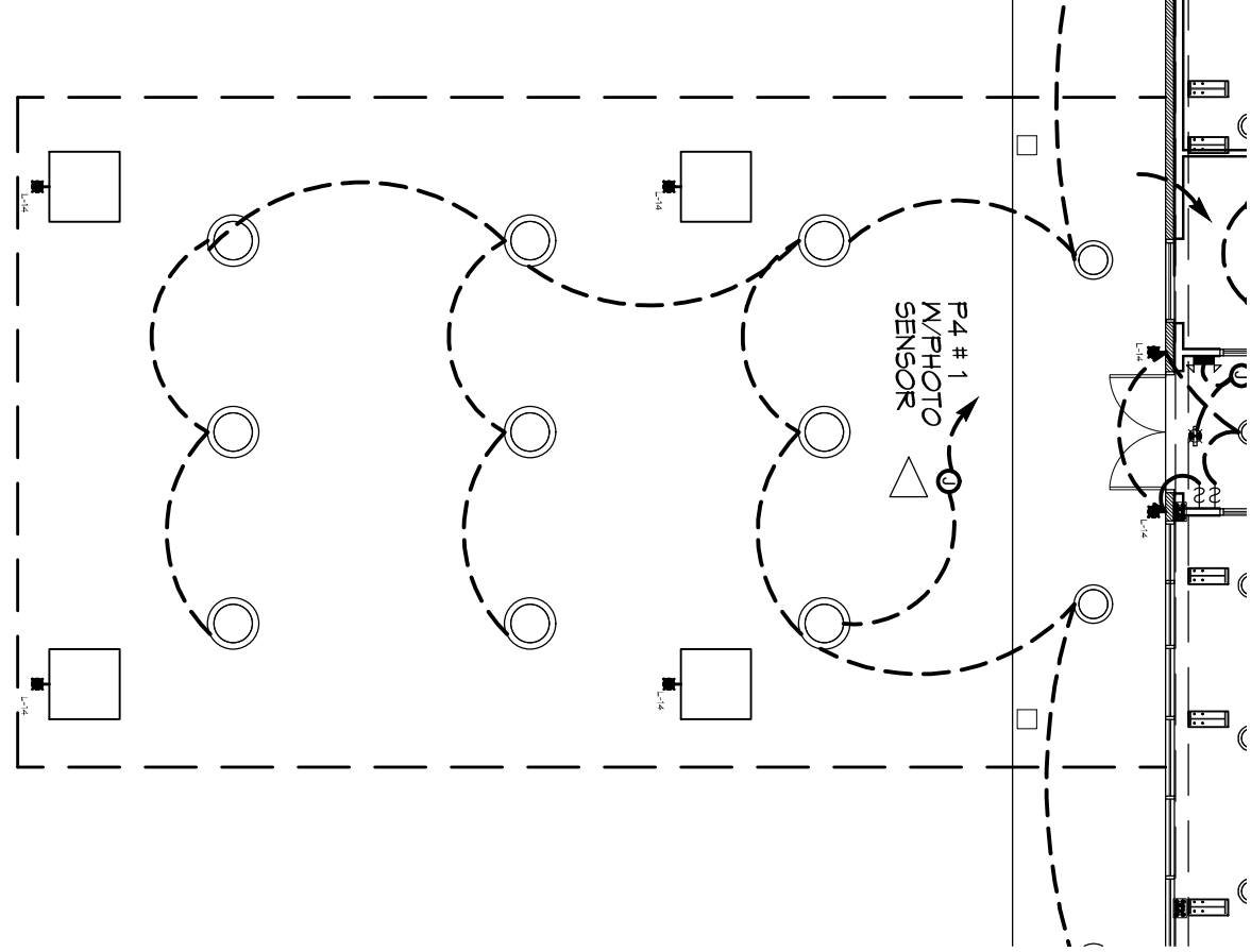
2 DRIVE THRU PLAN SCALE: 1/8" = 1'-0"
