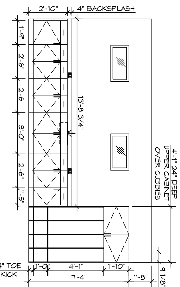
17 HOLDING/COSMETIZING ELEVATION SCALE: 1/4"=1'-0"
