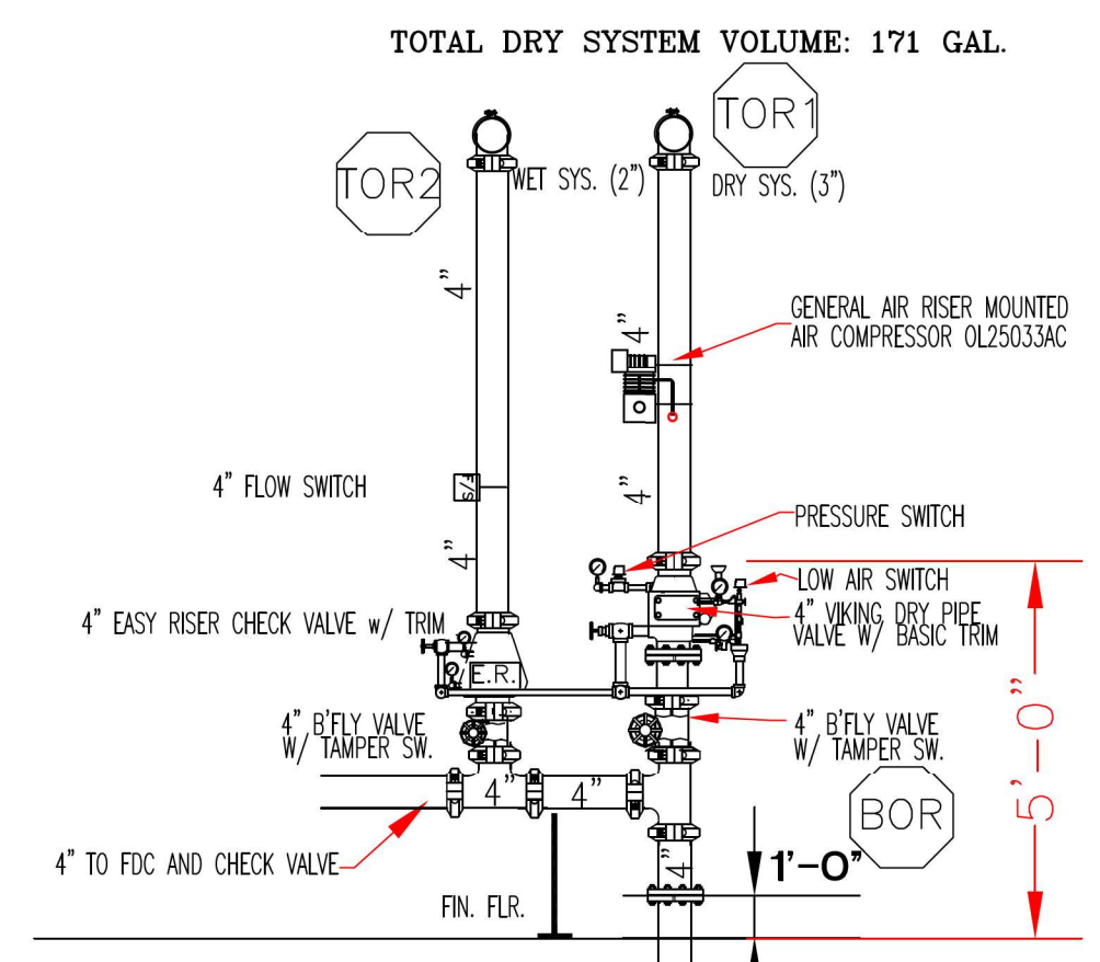
SYSTEM RISER DETAIL NOT TO SCALE
