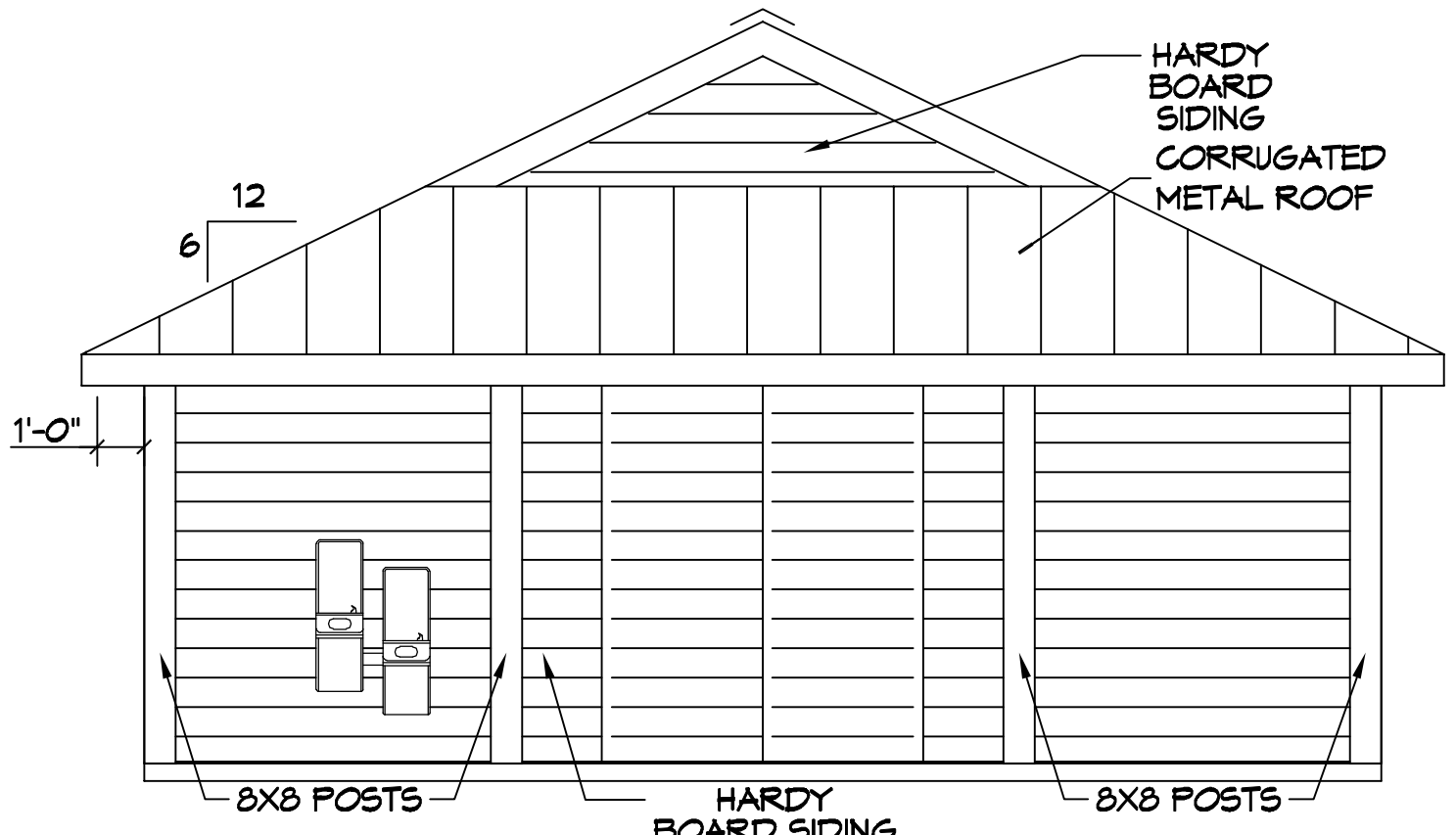
10 FRONT ELEVATION SCALE: 1/4" = 1'-0"
