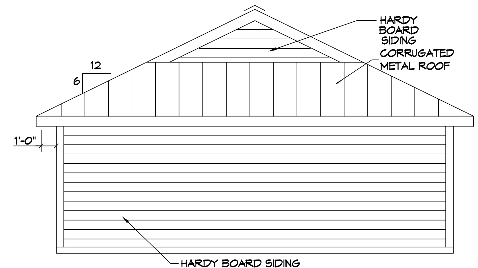
11 REAR ELEVATION SCALE: 1/4" = 1'-0"
