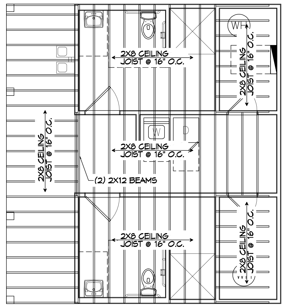
9 ROOF FRAMING PLAN SCALE: 1/4" = 1'-0"
