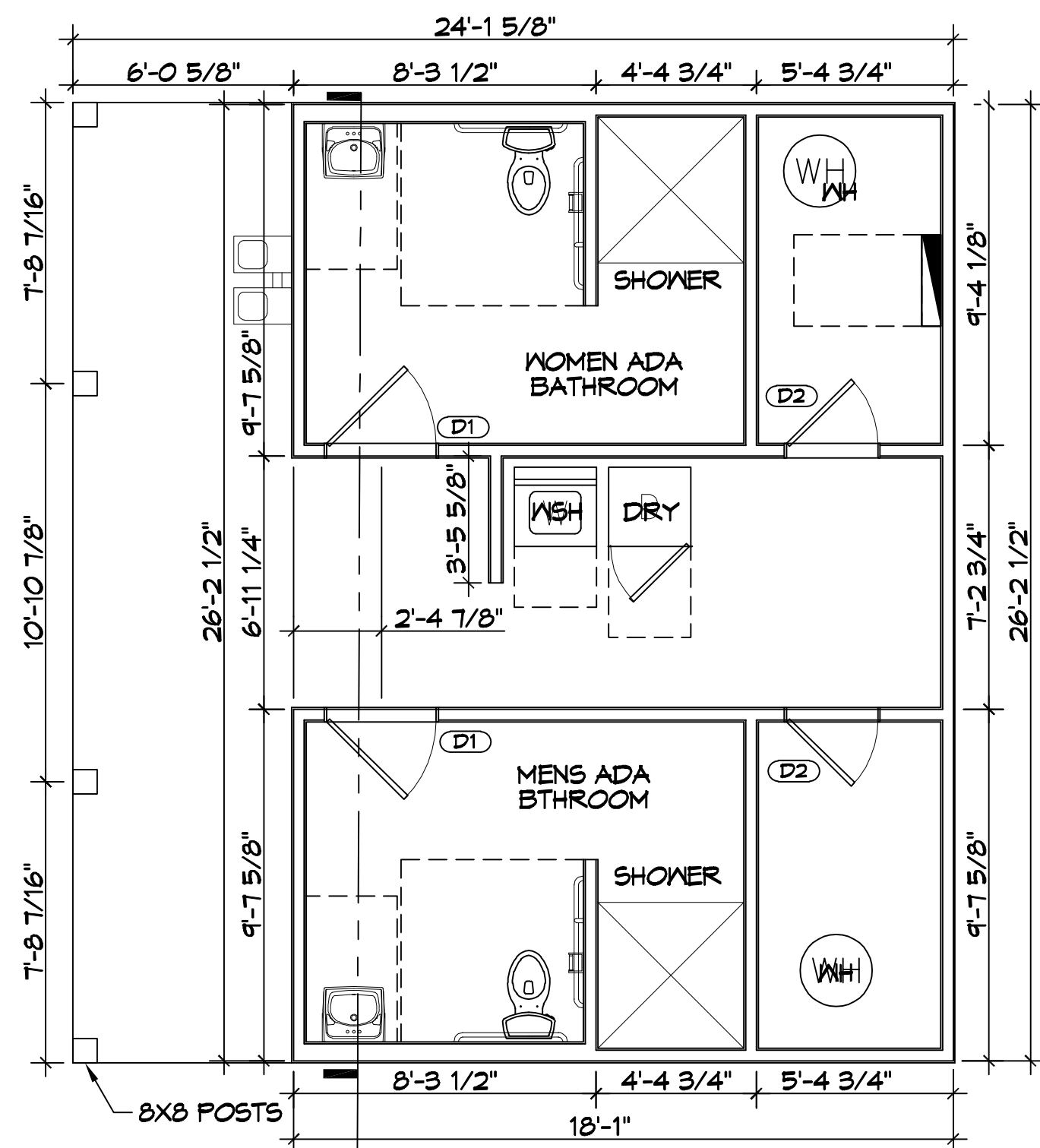
8 BATHROOM FLOOR PLAN SCALE: 1/4" = 1'-0"
