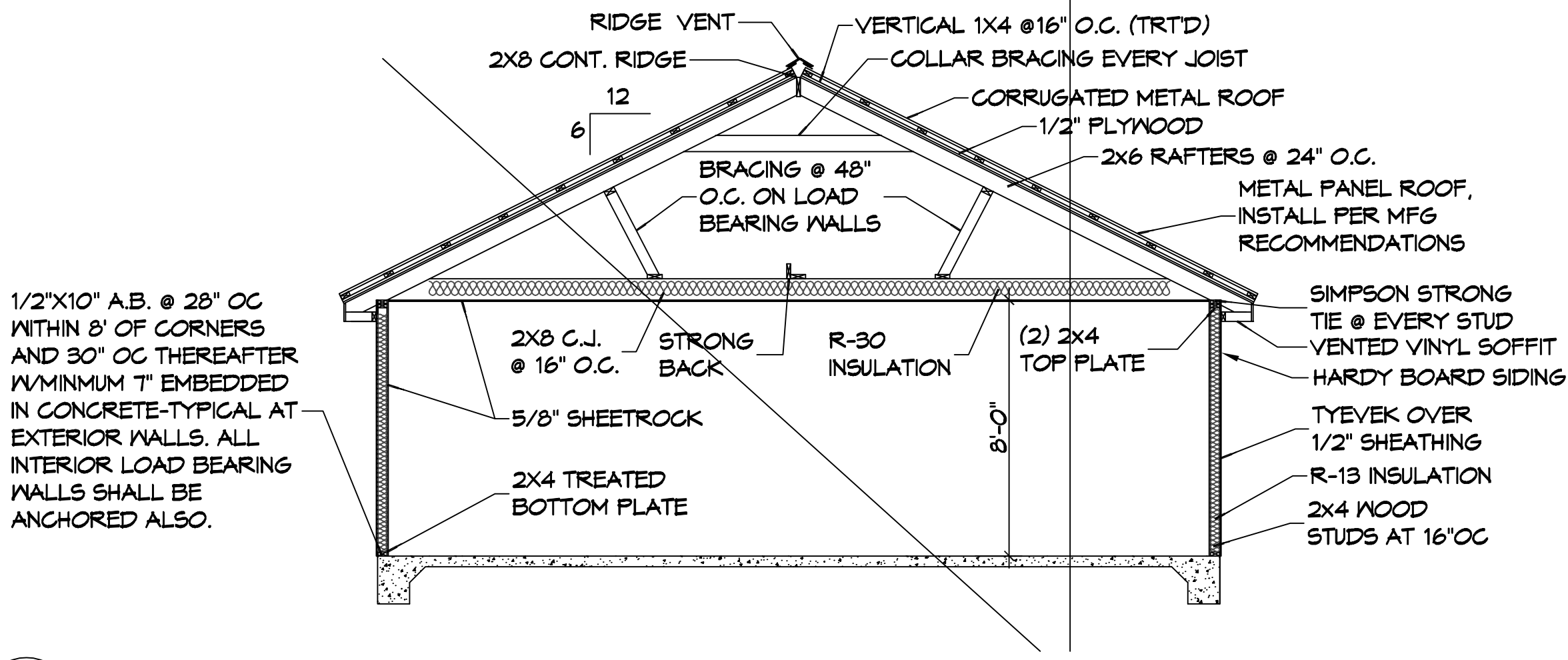
A SECTION VIEW SCALE: 1/4" = 1'-0"
