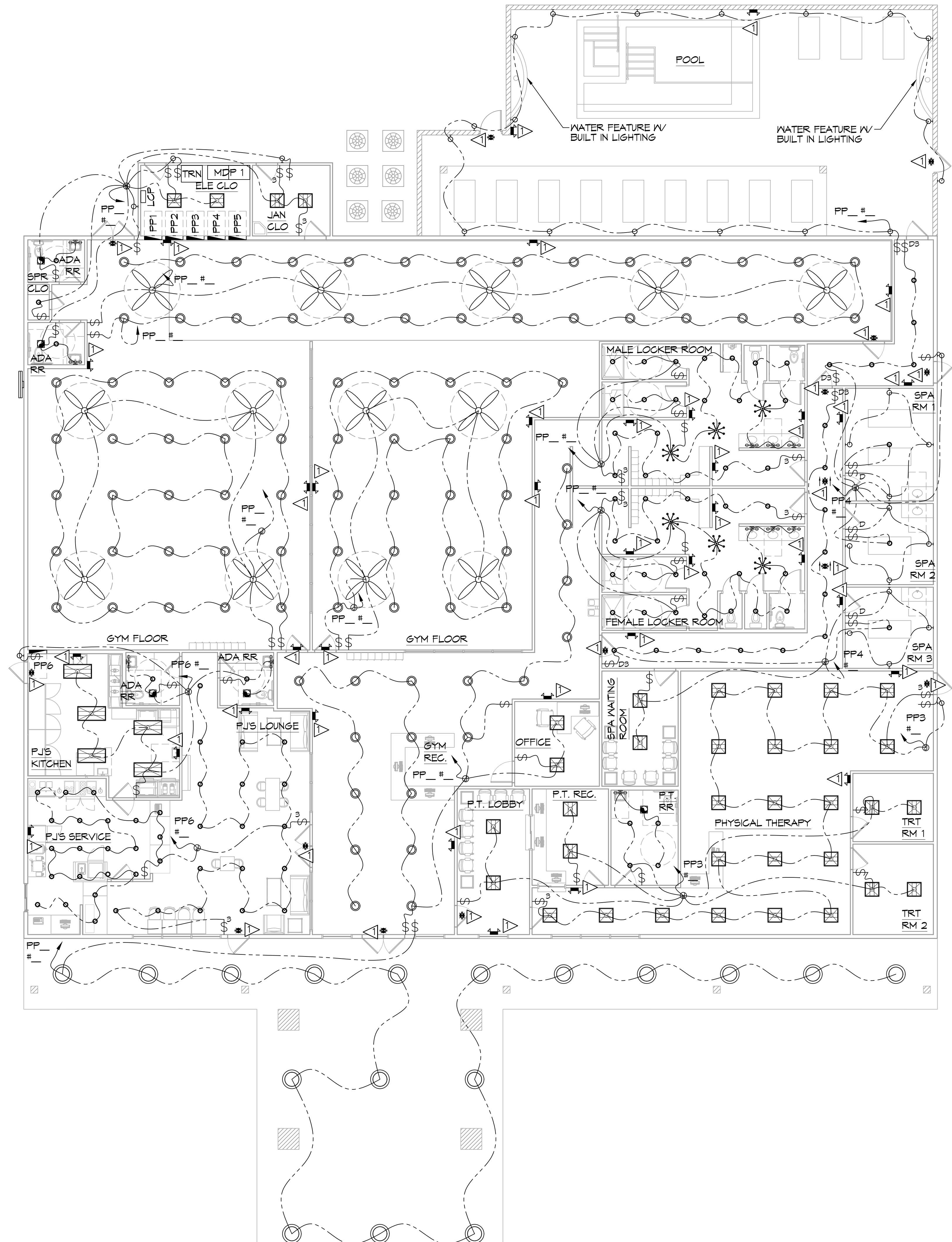
157 LIGHTING PLAN SCALE: 1/8" = 1'-0"
