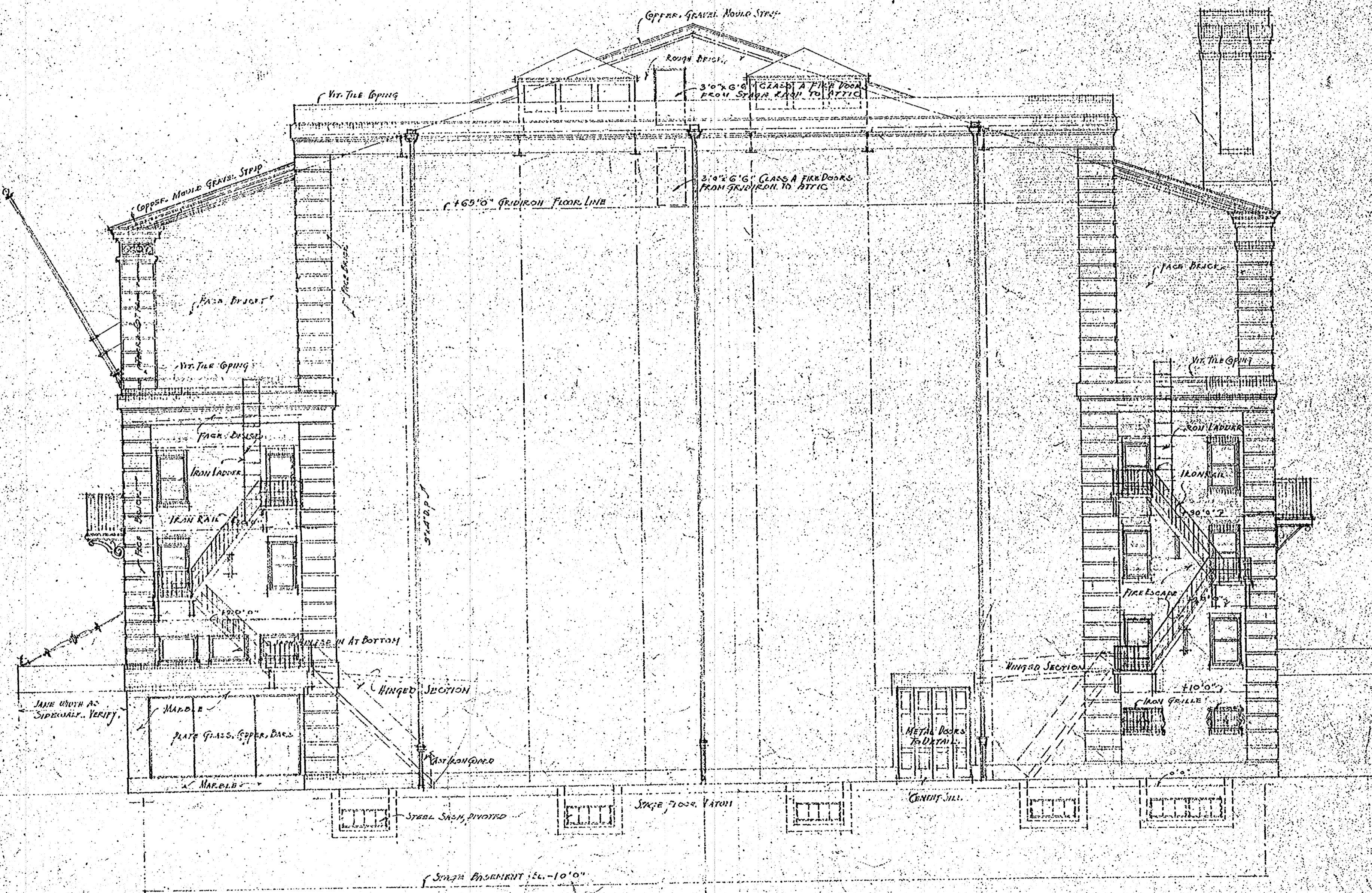
IBERVILLE STREET ELEVATION SCALE 1/8" = 1'-0"
