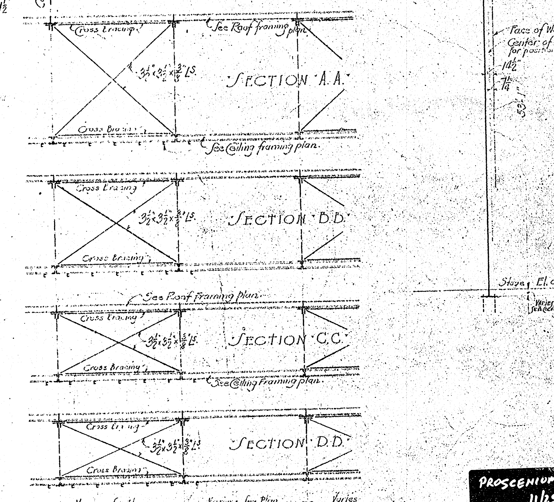
SECTION THRU TRUSSES SHOWING CROSS FRAMES
