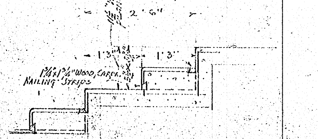
DETAIL OF AISLE STEPPING IN BALCONY SCALE 3/4 INCH = 1 FOOT
