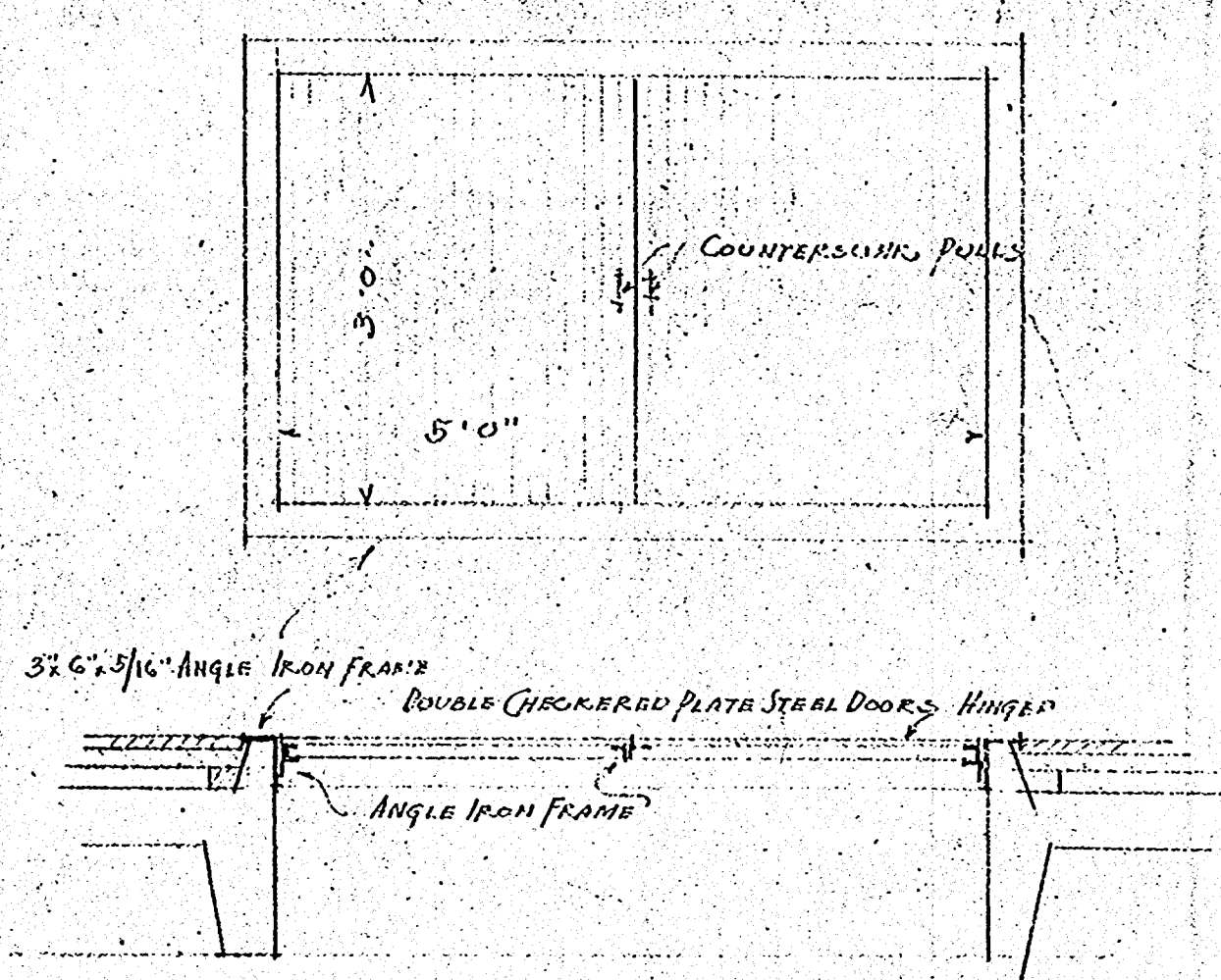
DETAIL OF TRUNK STOP SCALE 3/4 INCH = 1 FOOT
