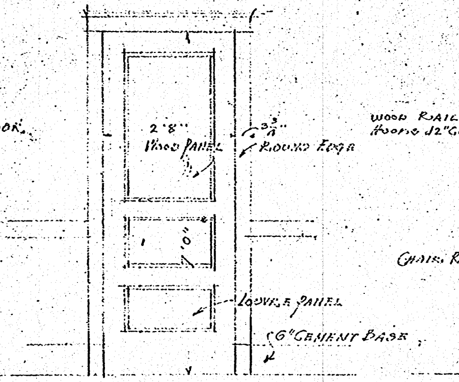
DRESSING ROOM DOORS SCALE 1/2 INCH = 1 FOOT
