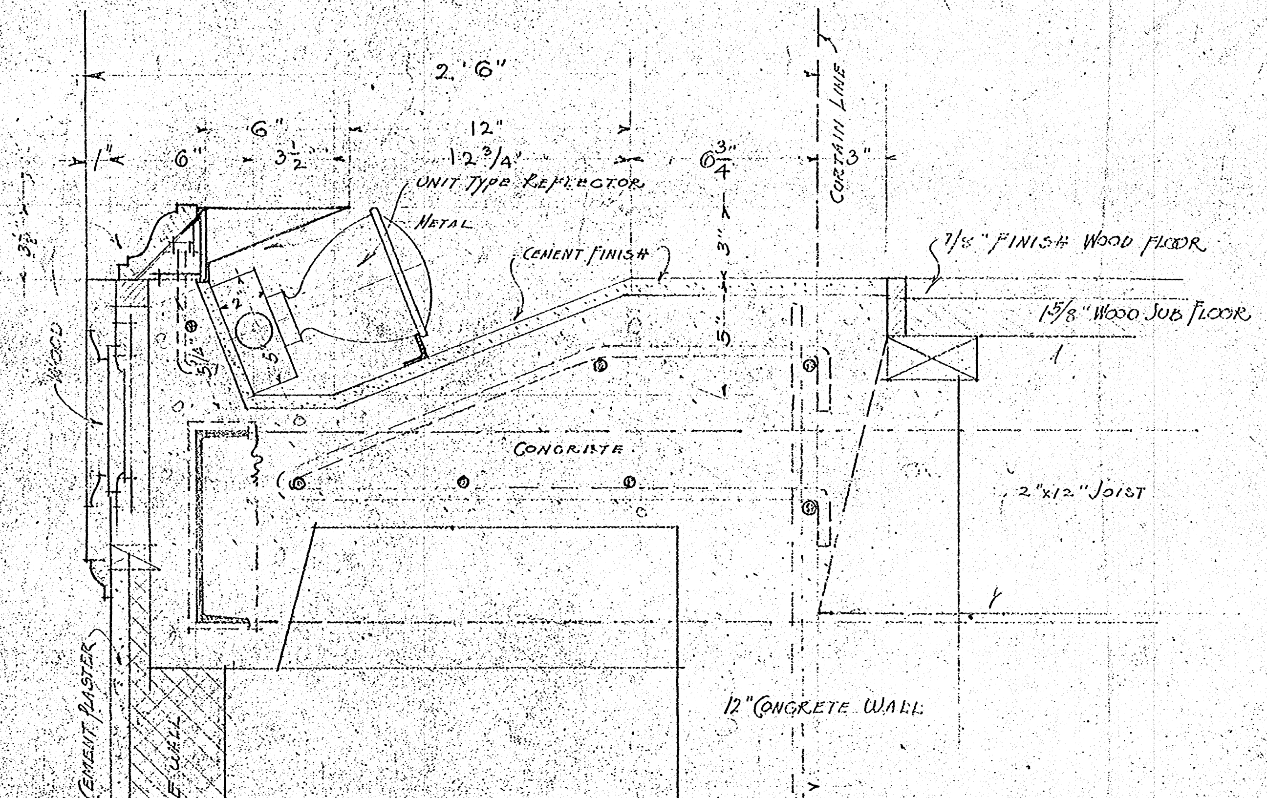
STAGE FRONT + FOOTLIGHTS SCALE 3 INCHES = 1 FOOT
