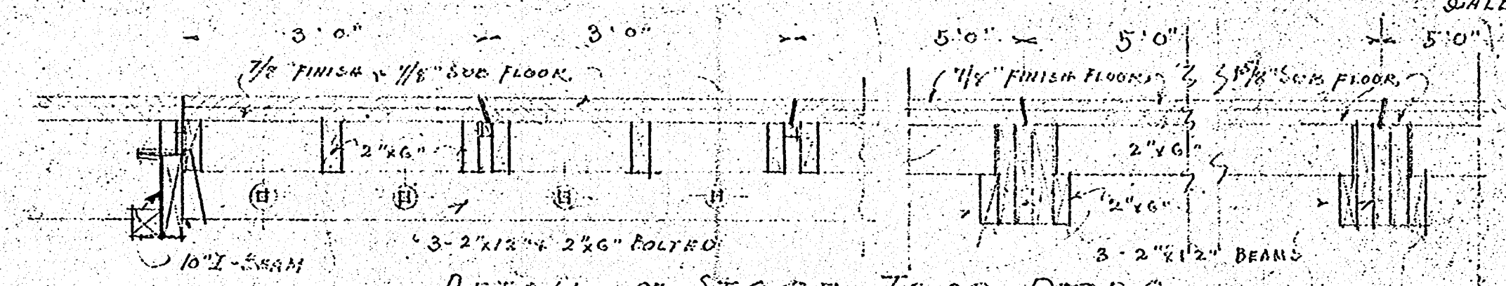
DETAIL OF STAGE TRAP DOORS SCALE 3/4 INCH = 1 FOOT
