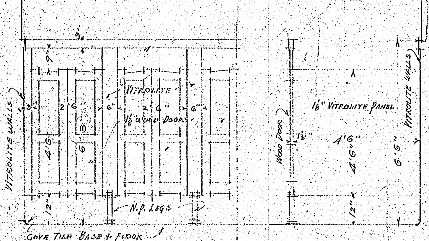
DETAIL OF TOILET STALLS (TYPICAL) SCALE 1/2 INCH = 1 FOOT
