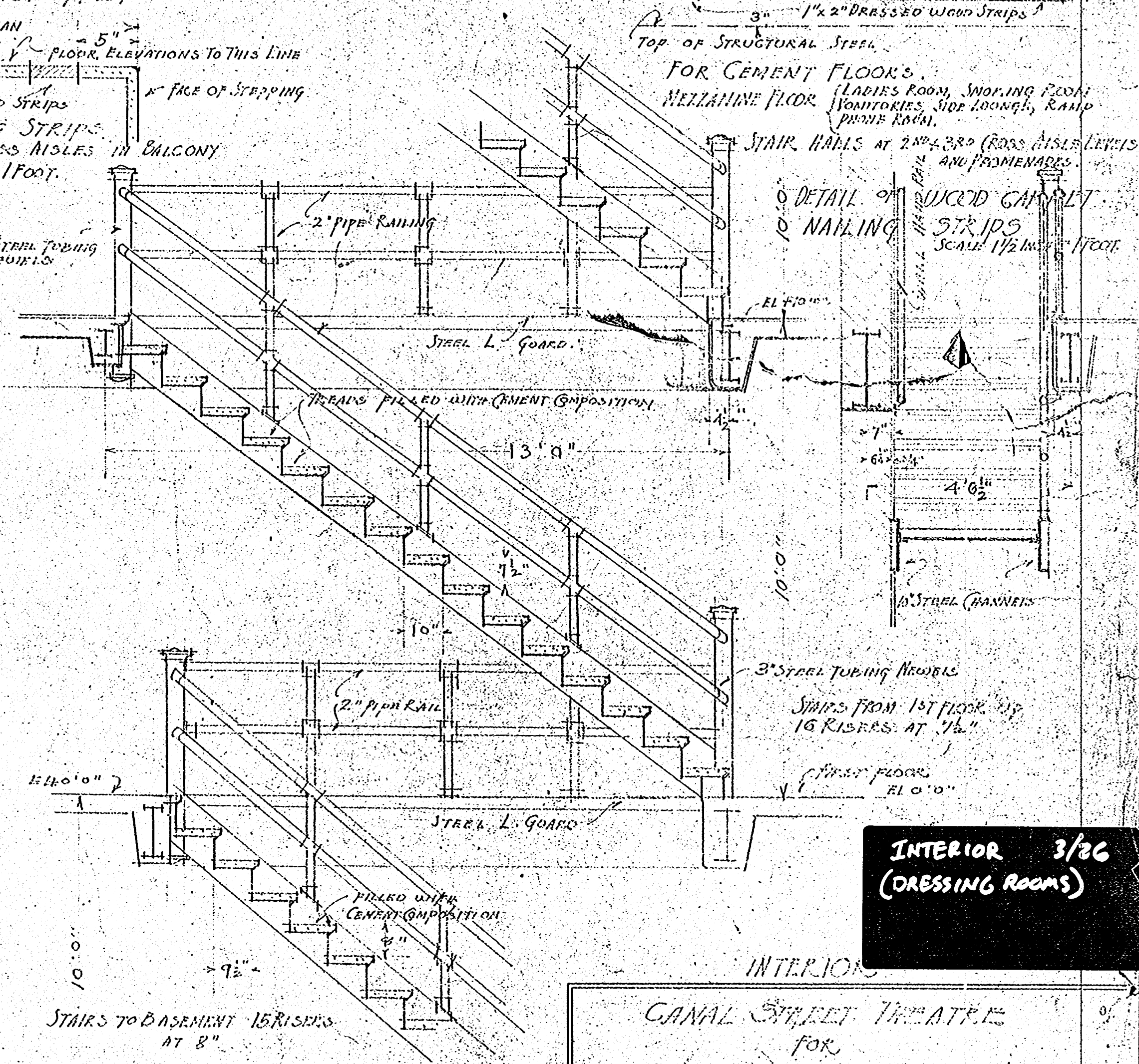
DRESSING ROOM STAIRS SCALE 1/2 INCH = 1 FOOT
