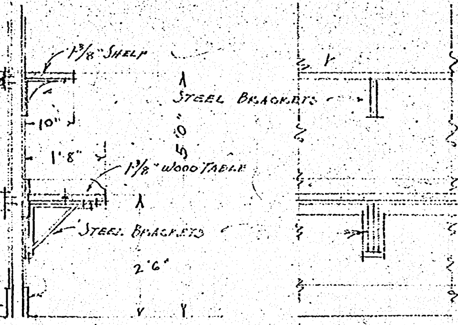
DRESSING ROOM TABLES ETC. SCALE 1/2 INCH = 1 FOOT
