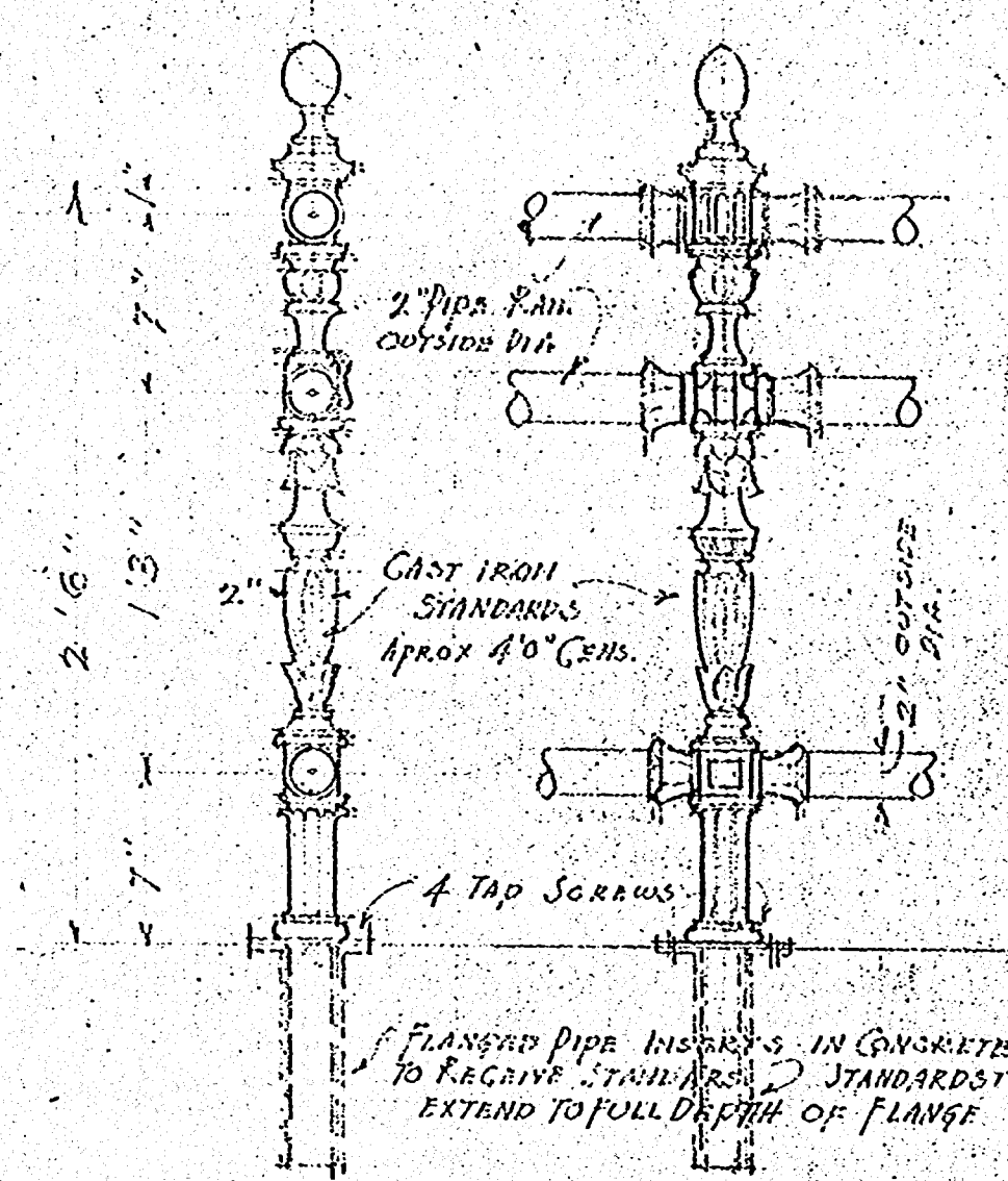
DETAIL OF PIPE + IRON RAILS FOR BALCONY CROSS AISLES SCALE 1/2 INCH = 1 FOOT
