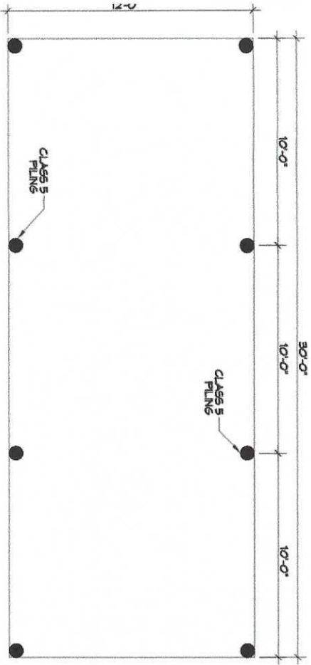
PILING PLAN
