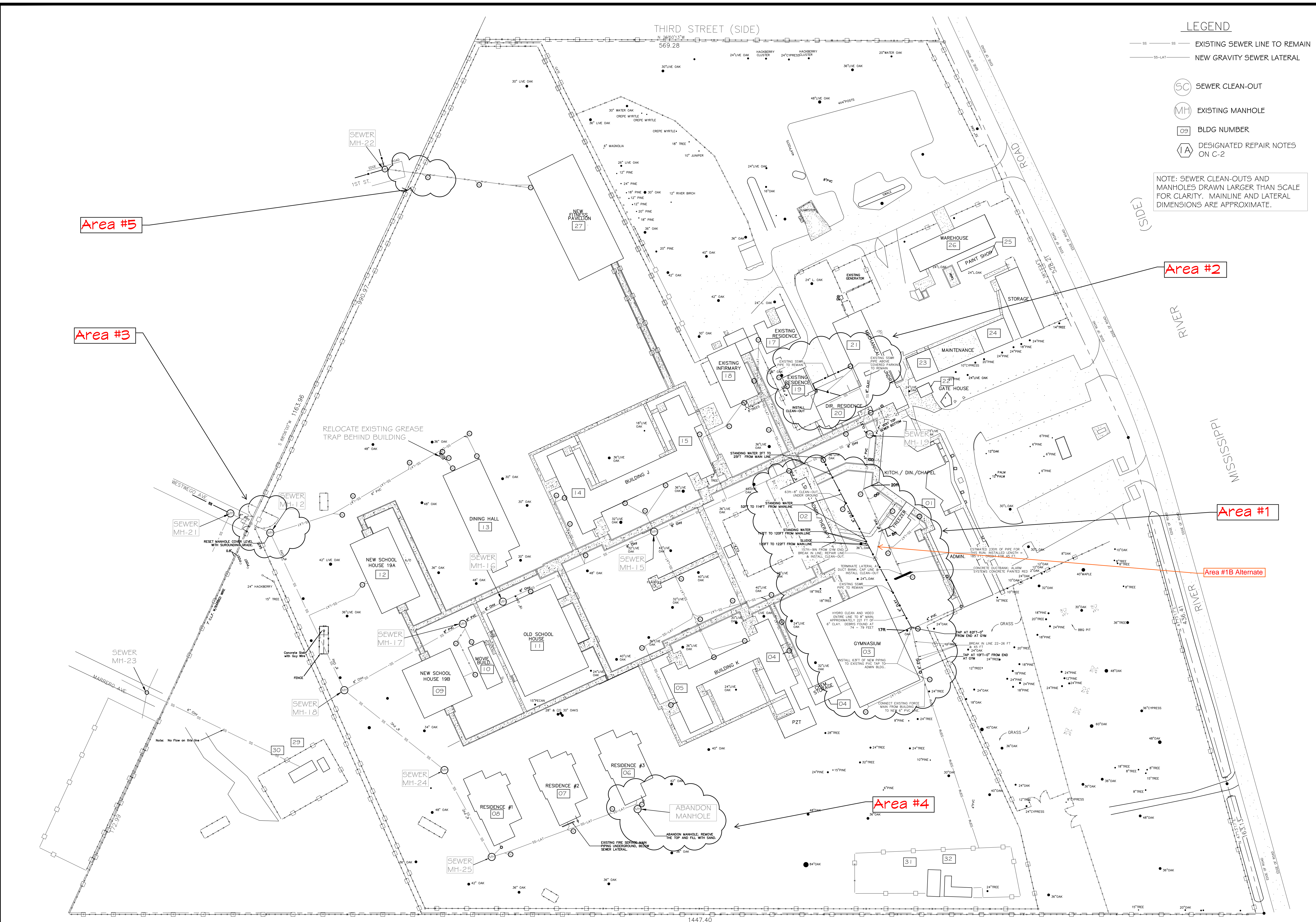
SITE PLAN SCALE: 1" = 50' 1447.40 S 26°50'13"E 50 25 0 50 SCALE IN FEET
