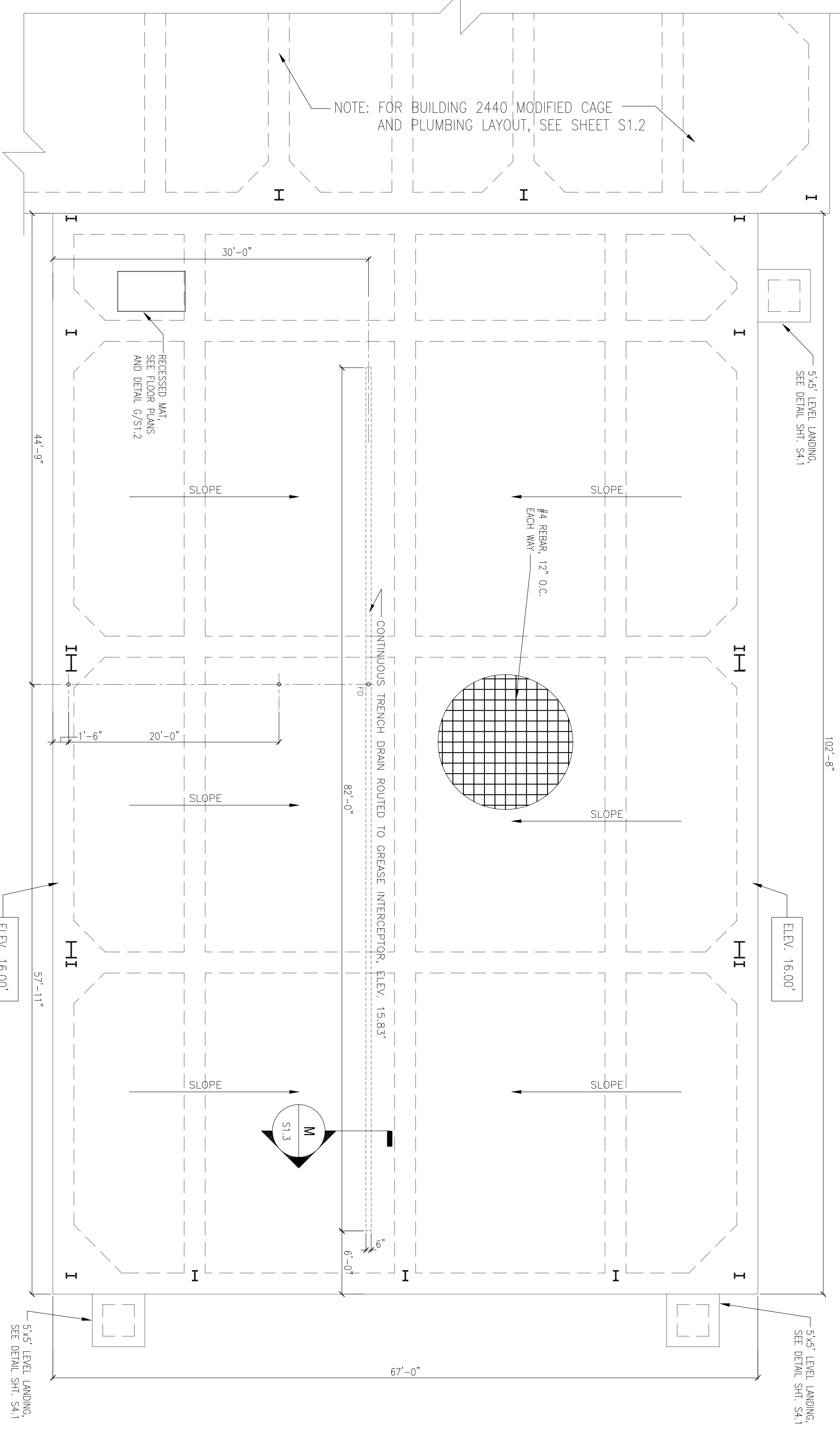
BLDG. 2441 MODIFIED PLUMBING LAYOUT SCALE: 3/16" = 1'-0"
