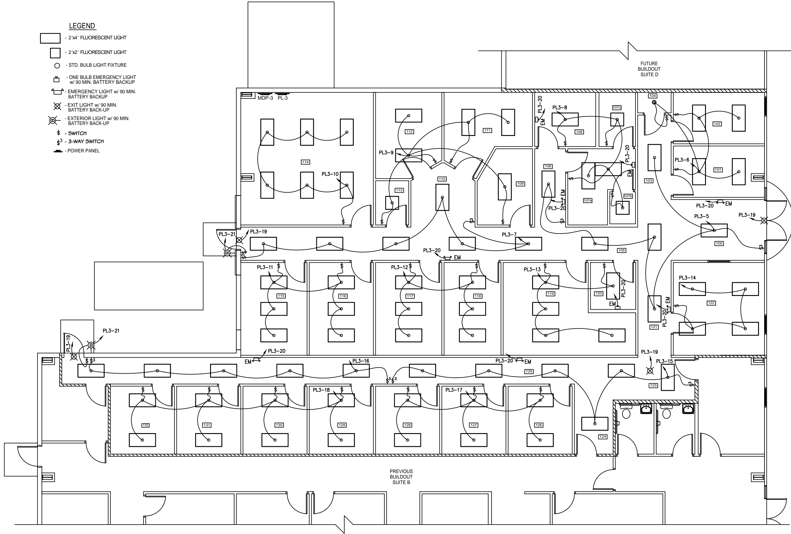
ELECTRICAL LIGHTING PLAN-SUITE C SCALE: 1/4"=1'
