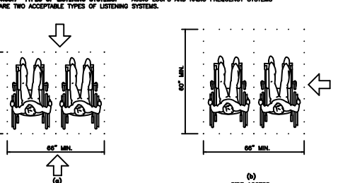
FIG. 46 SPACE REQUIREMENTS FOR WHEELCHAIR SEATING SPACES IN SERIES N.T.S.
