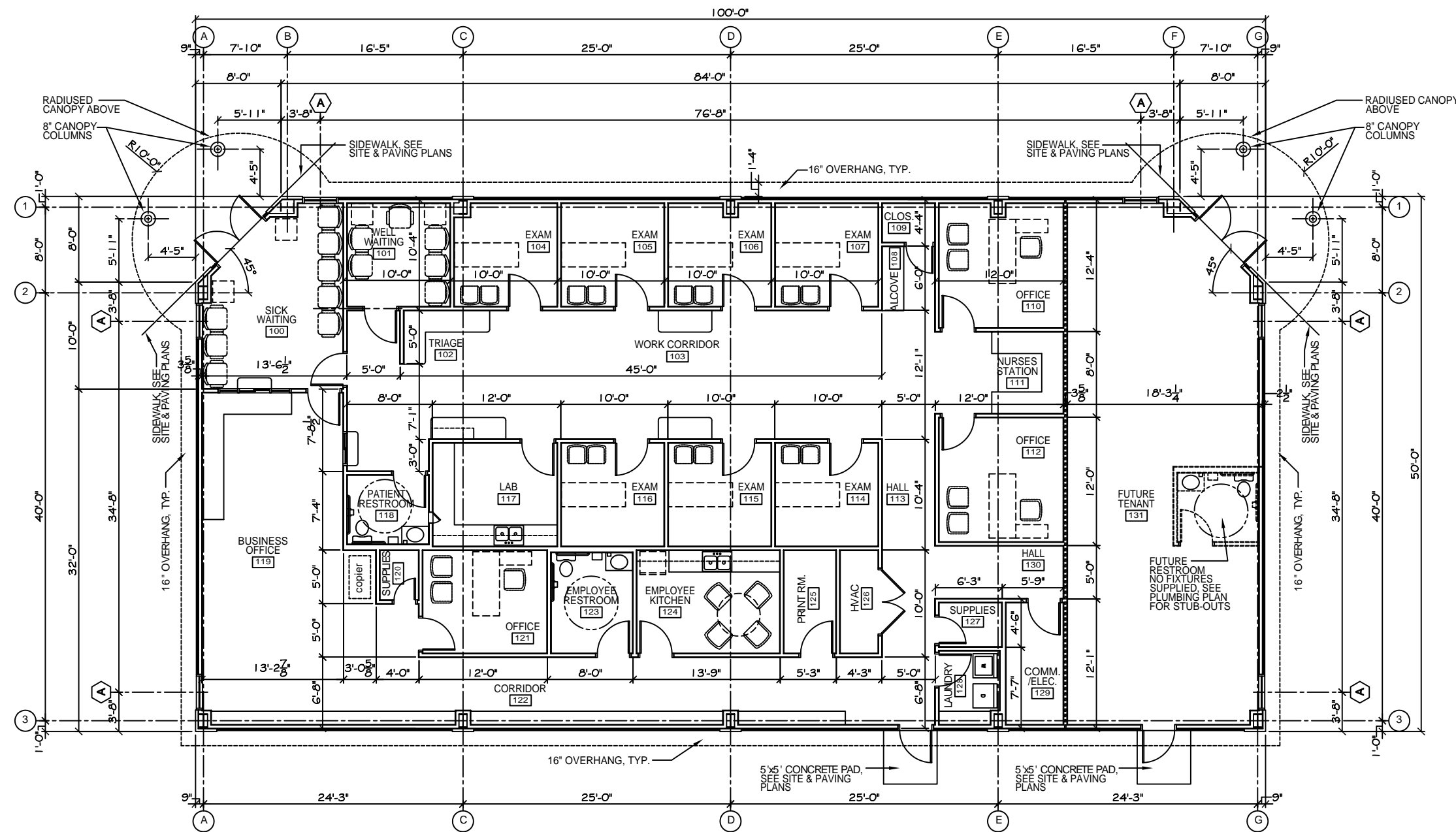
FLOOR PLAN SCALE: 3/16"=1'
