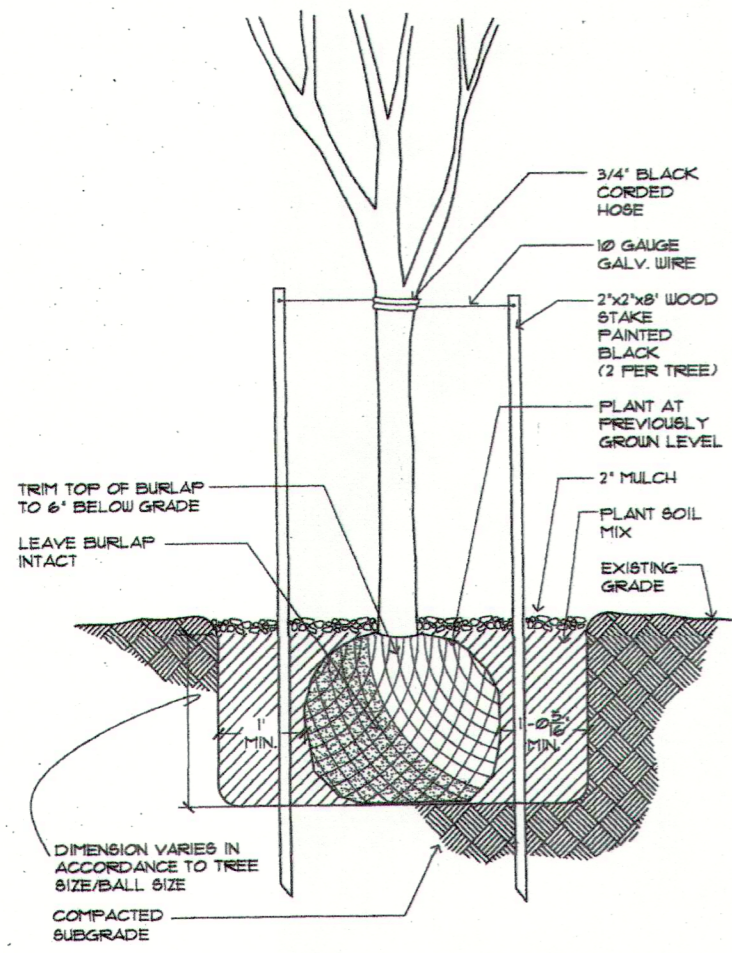
TREE PLANTING DETAIL NOT TO SCALE
