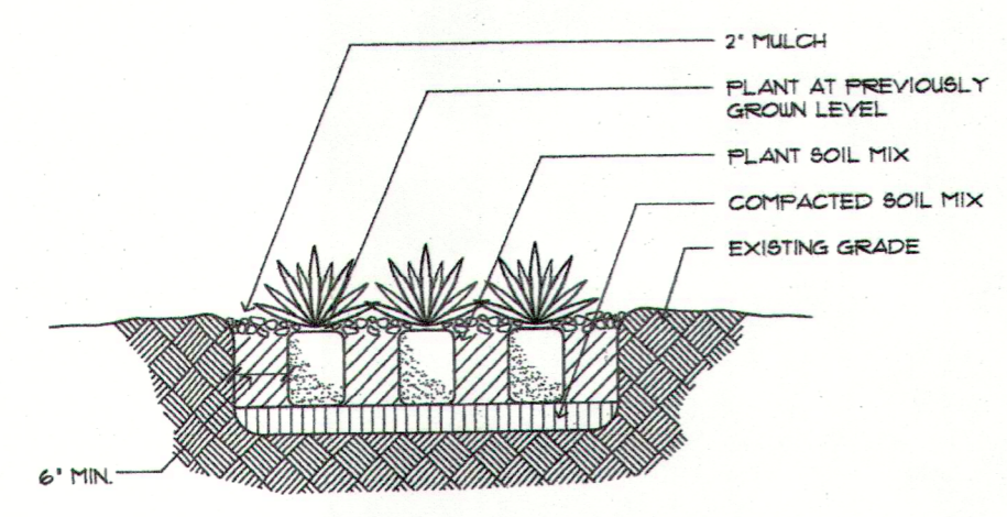
GROUNDCOVER PLANTING DETAIL NOT TO SCALE
