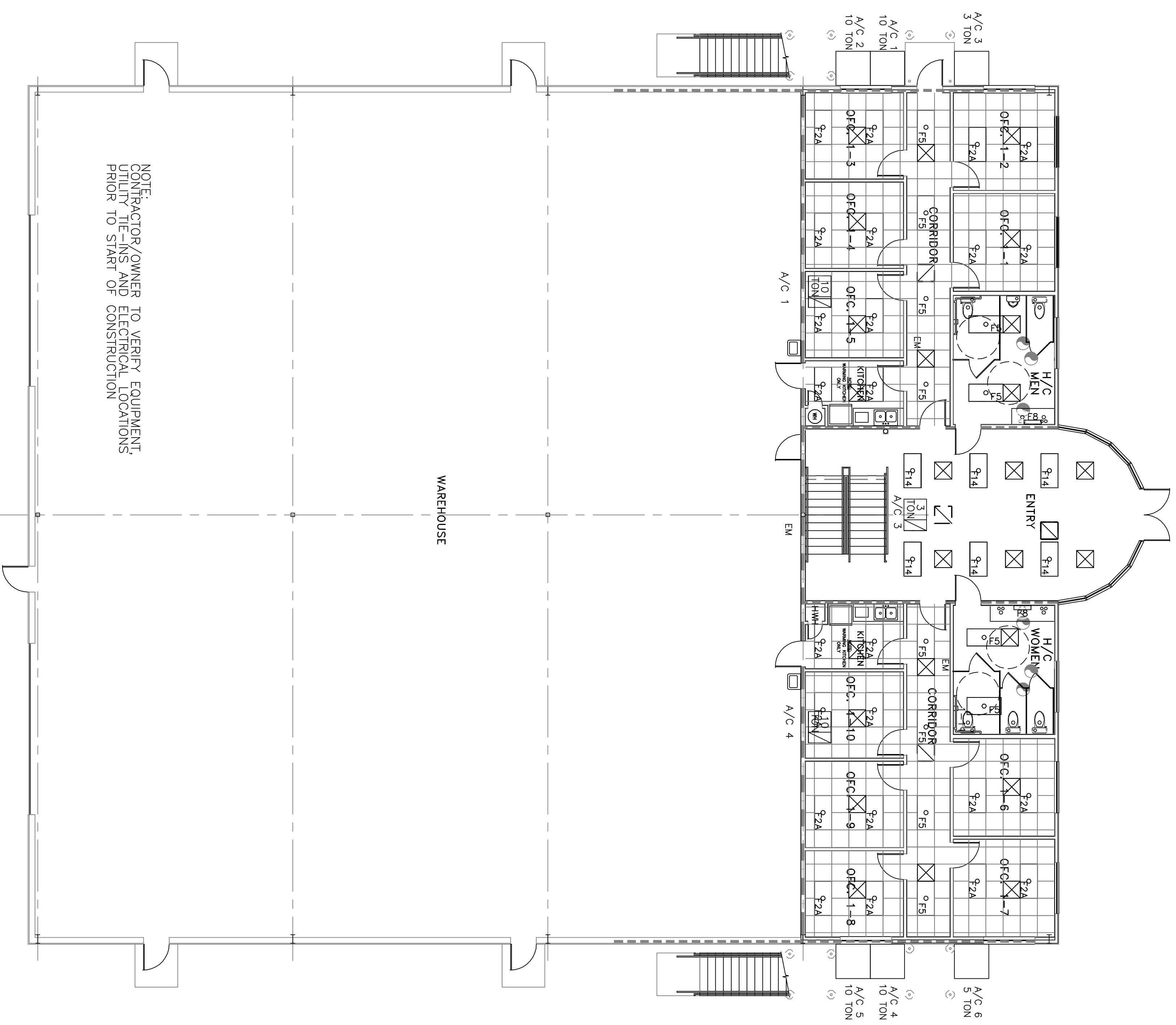
FIRST FLOOR REFLECTED CEILING PLAN SCALE: 1/8"=1'-0"
