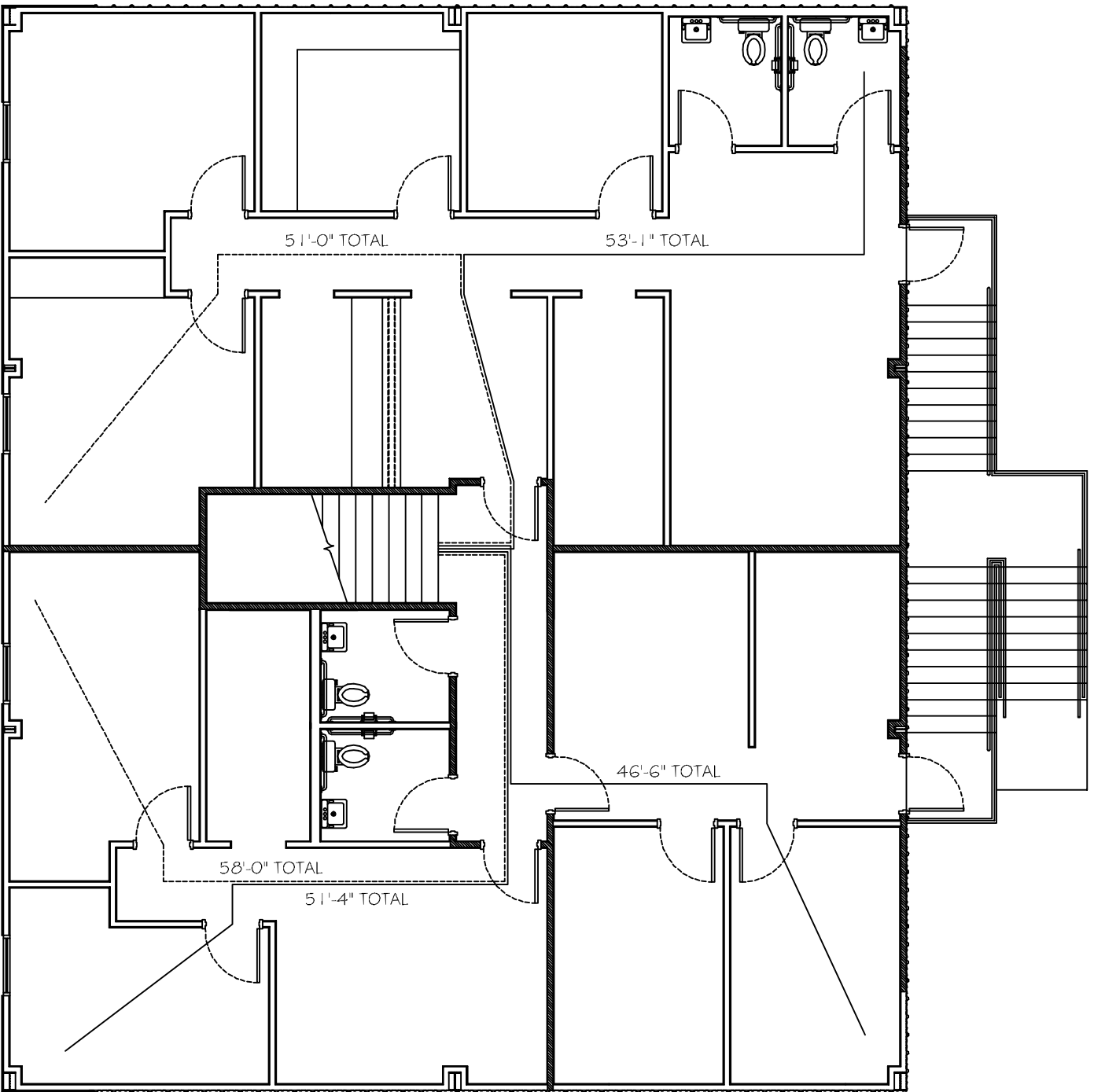
SECOND FLOOR PLAN SCALE: 3/16" = 1'-0"
