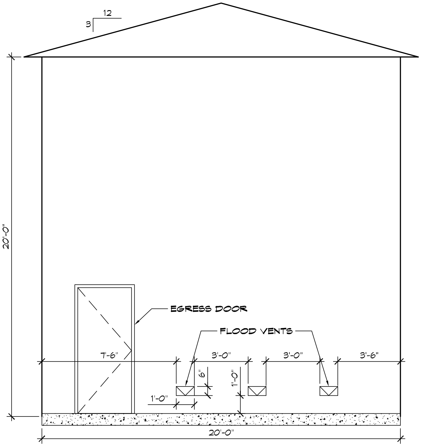
FLOOD VENTS
